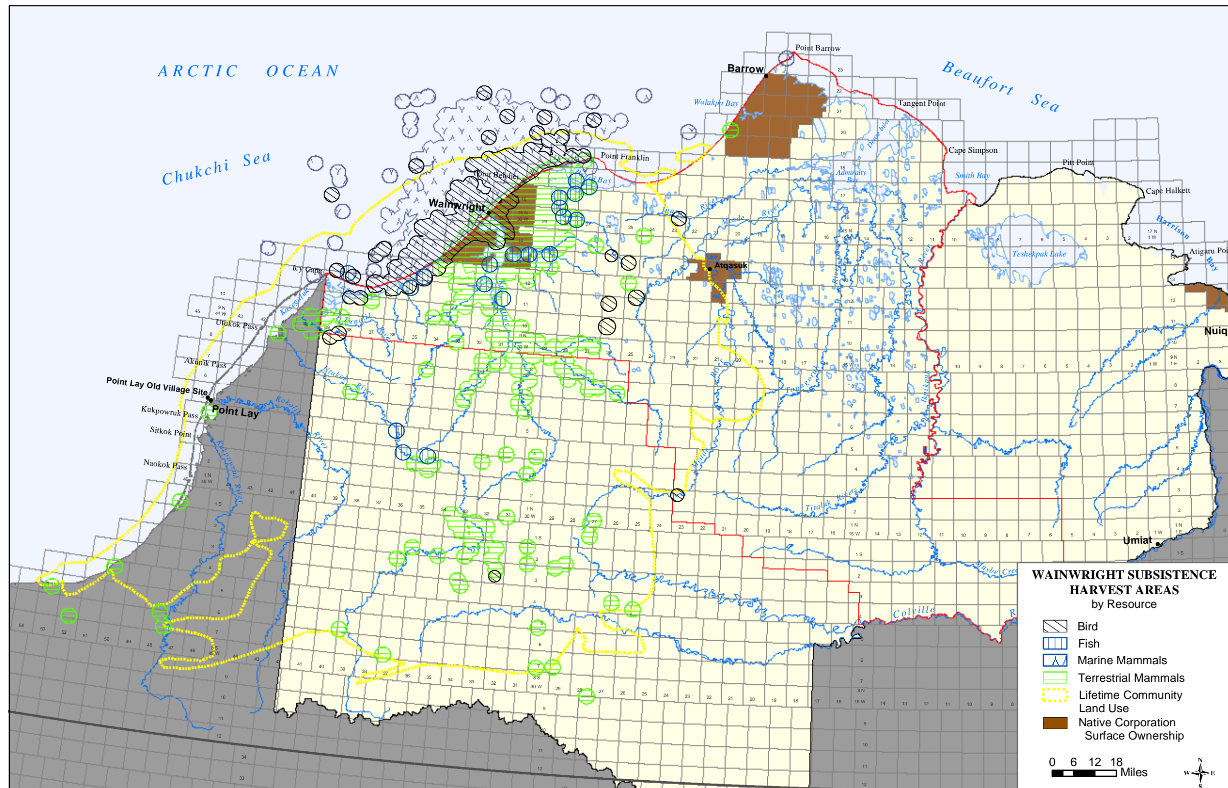
Map 69. Wainwright Subsistence Harvest Sites for Fish, Birds, and Terrestrial and Marine Mammals
