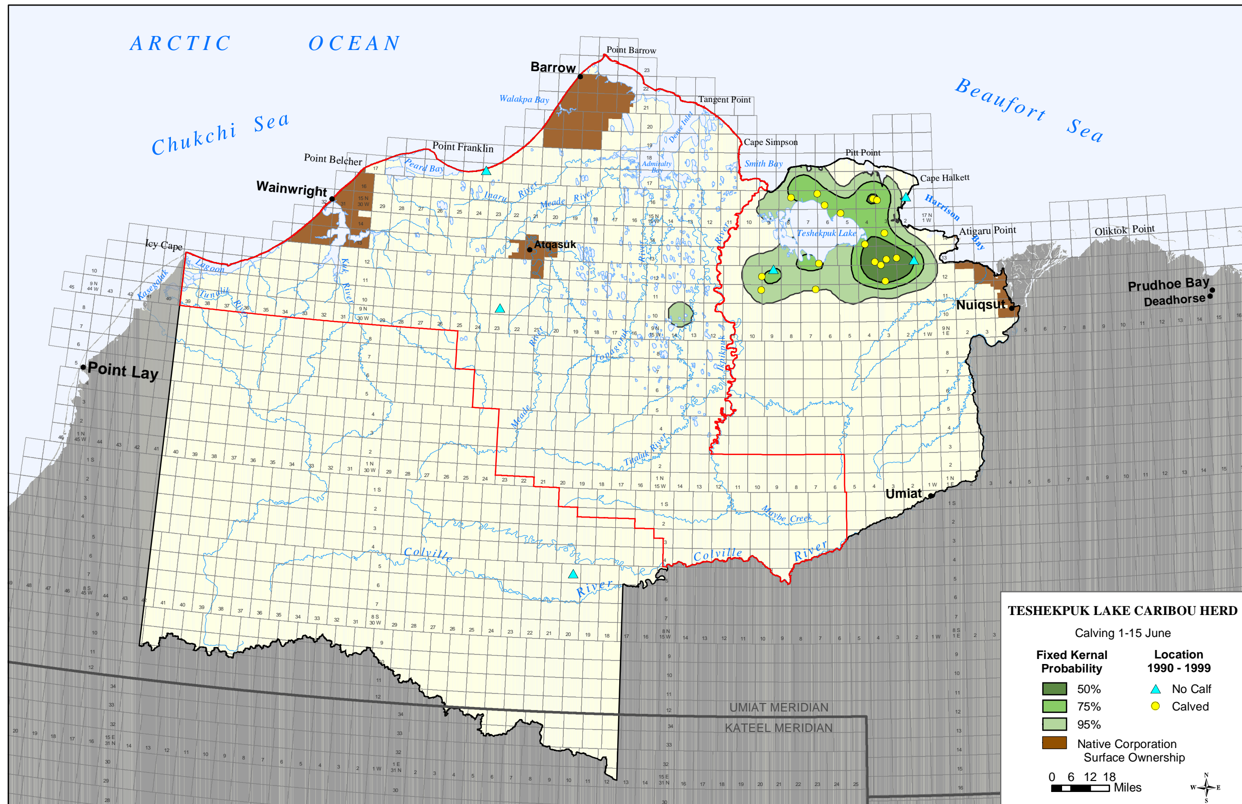
Map 48. Teshekpuk Lake Caribou Herd Calving Grounds (1990 - 1999 Satellite Telemetry Data)
