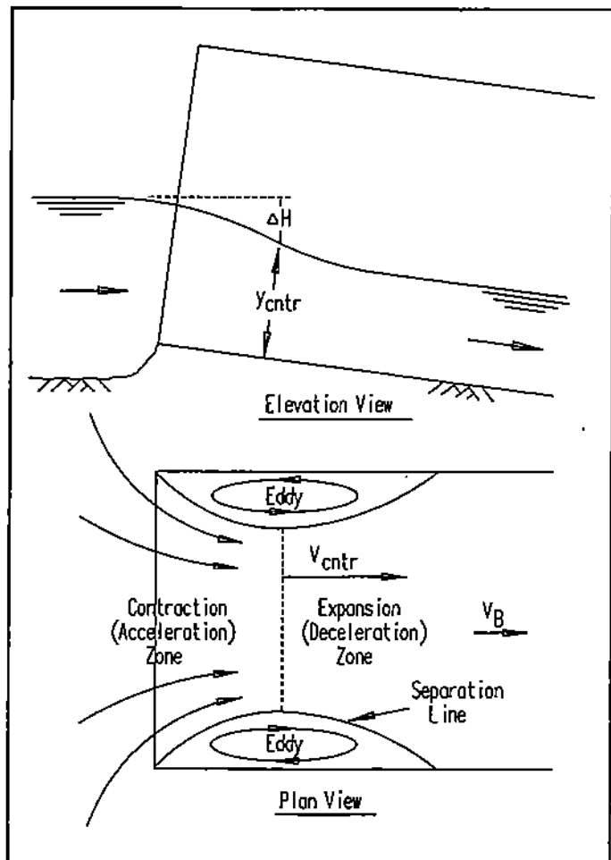
Figure IV-18. Details of flow in culvert inlet zone.
