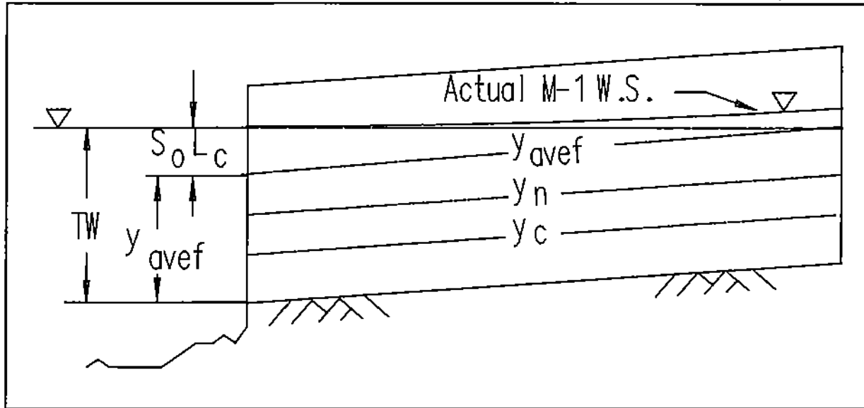
Figure VI-2. Safe TW elevation when safe fish passage water depth is less than normal depth, and normal depth is greater than critical depth. M-1 water surface profile provides some safety factor.
