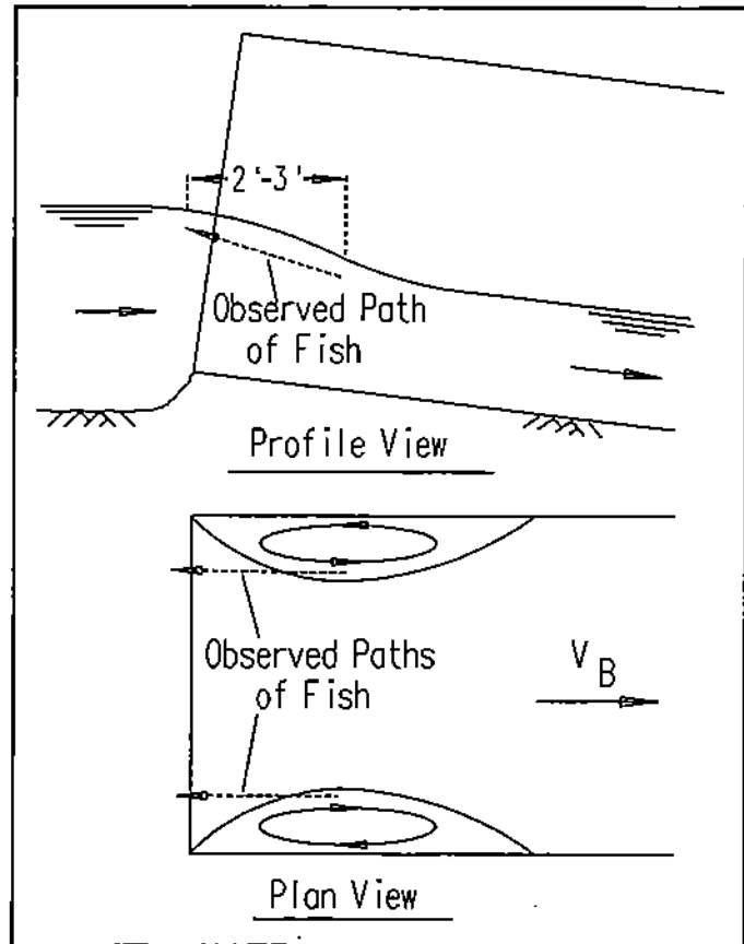
Figure IV-20. Observed fish passage routes at difficult inlet.
