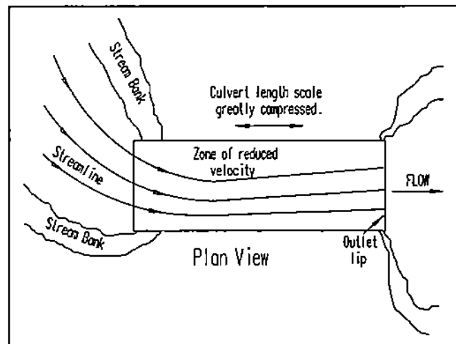
Figure IV-19. Conceptual sketch of how culvert skew reduces water velocity on one side of the culvert.
