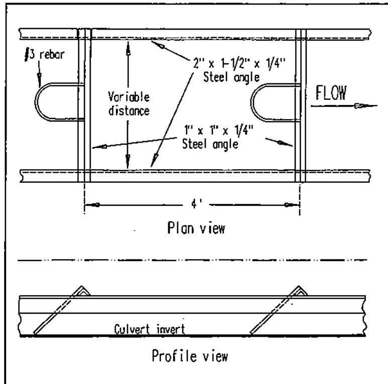
Figure IV-17. Montana bedload connector. "Ladder" is fabricated in 20-foot sections and bolted together when placed in culvert. Cross #3-members and rebar loops are welded to side members.
