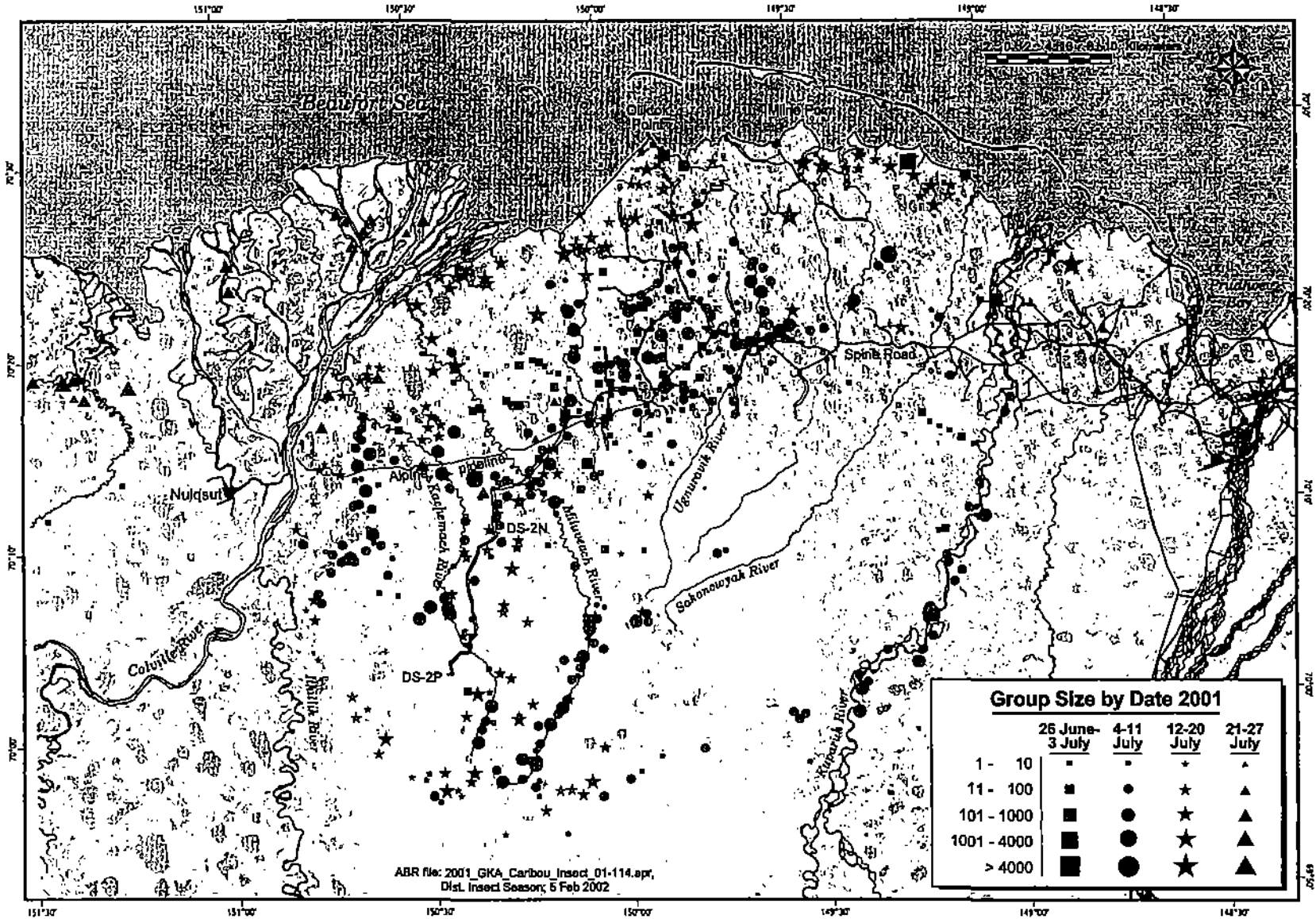
Figure 13. Distribution and sizes of caribou groups observed on systematic and reconnaissance aerial surveys of the Kuparuk-Colville region during the insect season, 26 June-27 July 2001. Survey coverage was not uniform over the entire area portrayed.
