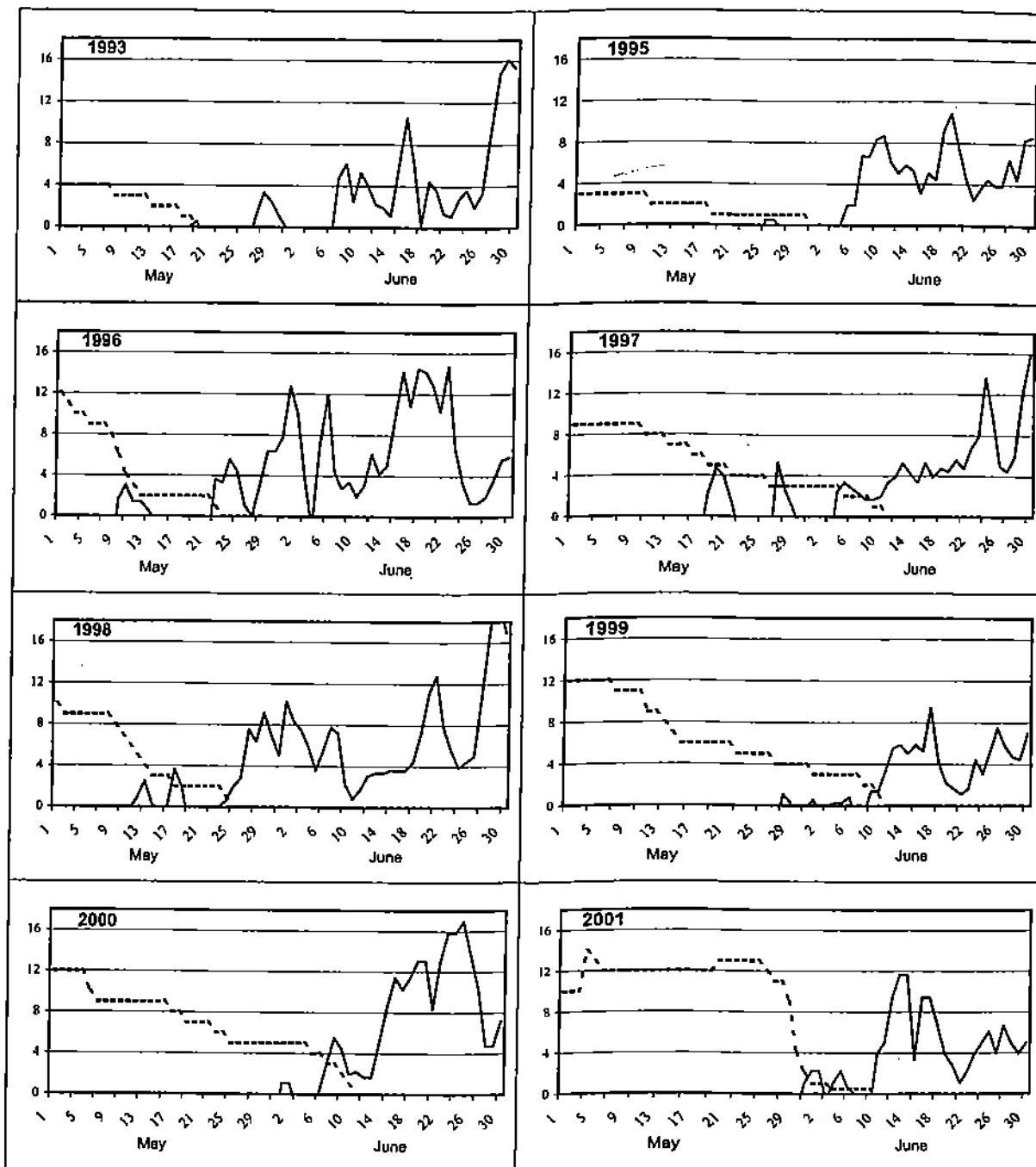
Figure 2. Snow depth (inches; dashed lines) and average daily temperature ( ^{\circ} C; solid lines) at the Kuparuk airstrip, May–June 1993–2001.
