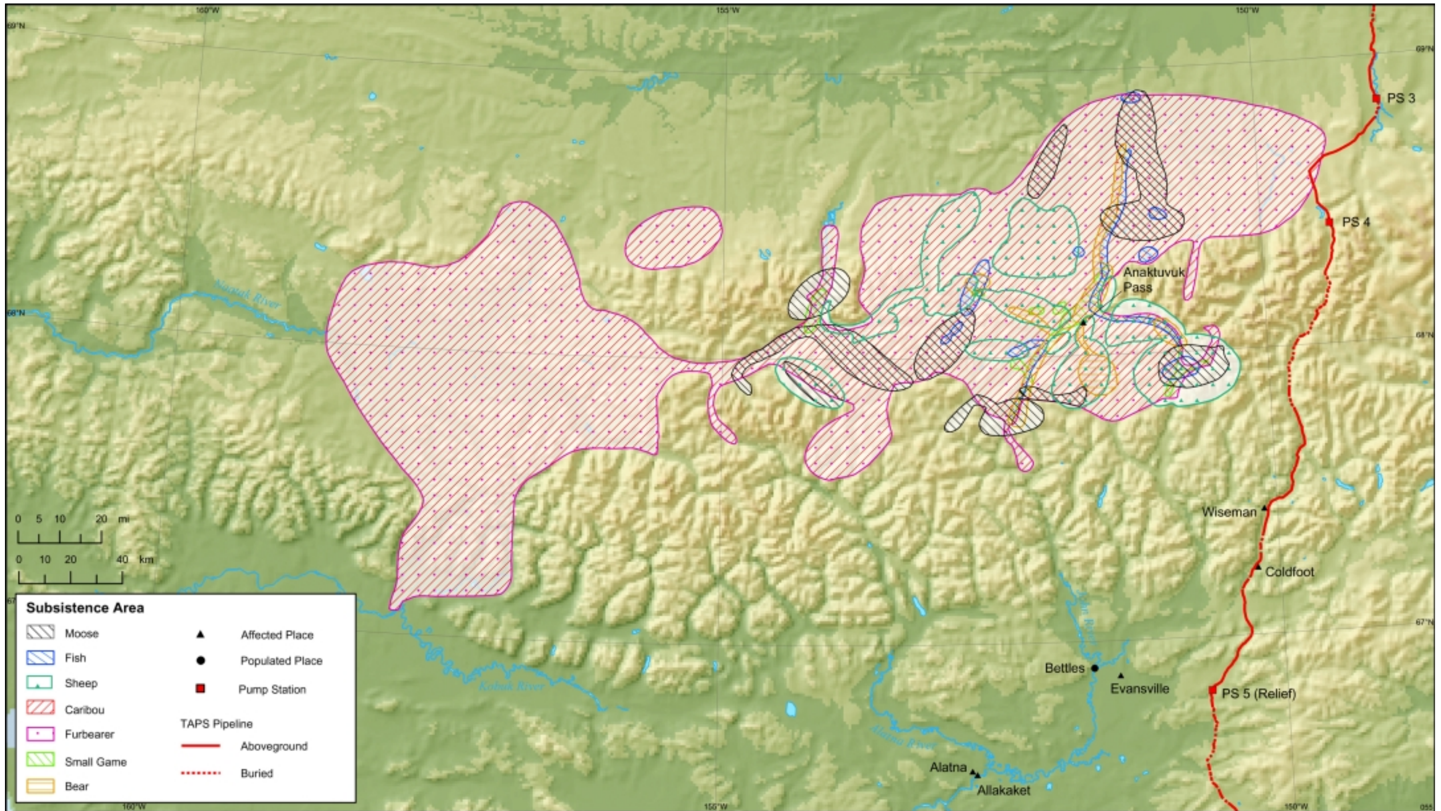
FIGURE D-6 Subsistence Harvest Areas Associated with Anaktuvuk Pass (Data Source: ADF&G undated)
