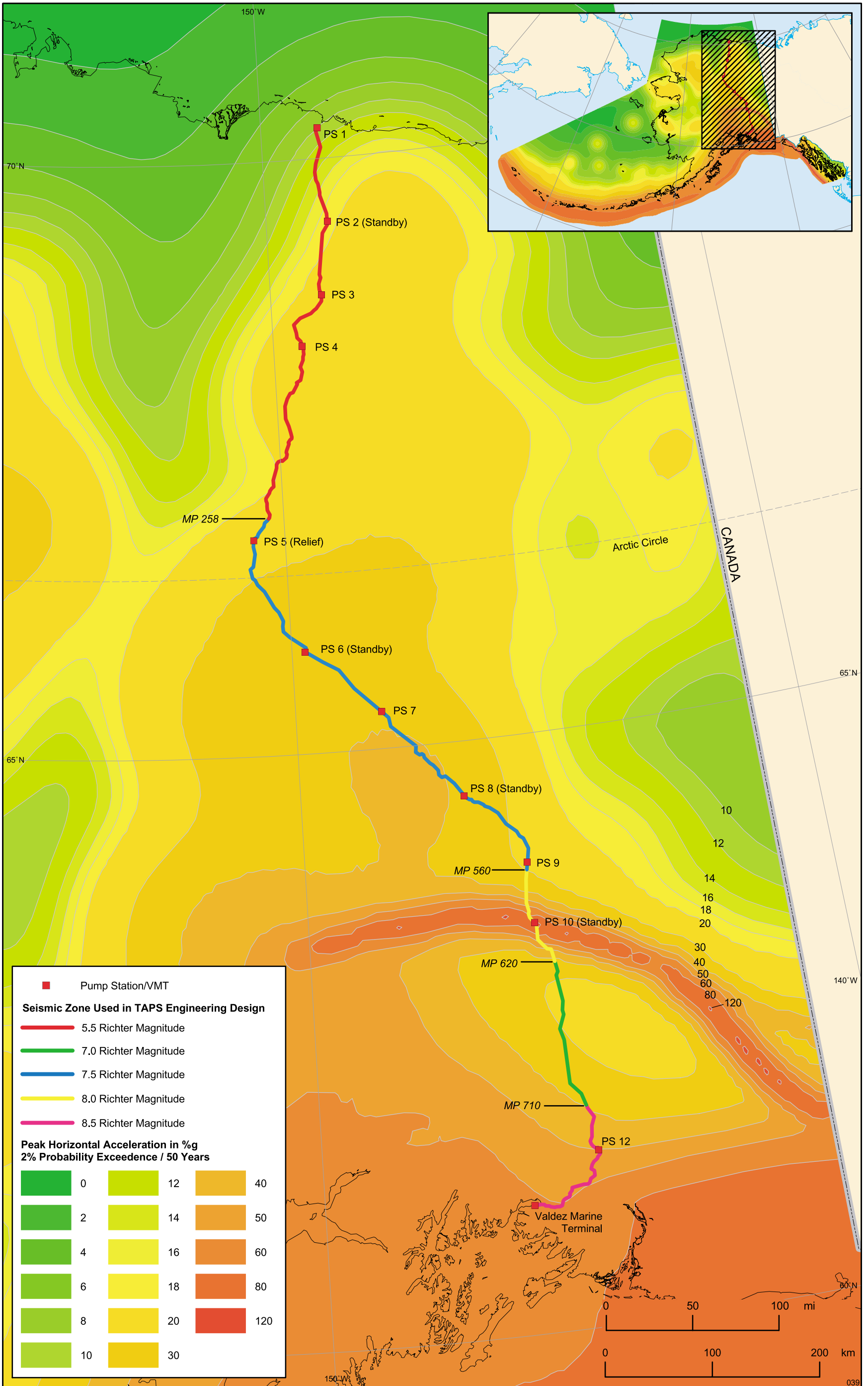
FIGURE 3.4-2 Estimated Peak Ground Acceleration and Design Ground Acceleration for the Design Contingency Earthquake Used in TAPS Design (Modified from Wesson et al. 1999; APSC 2001e)
