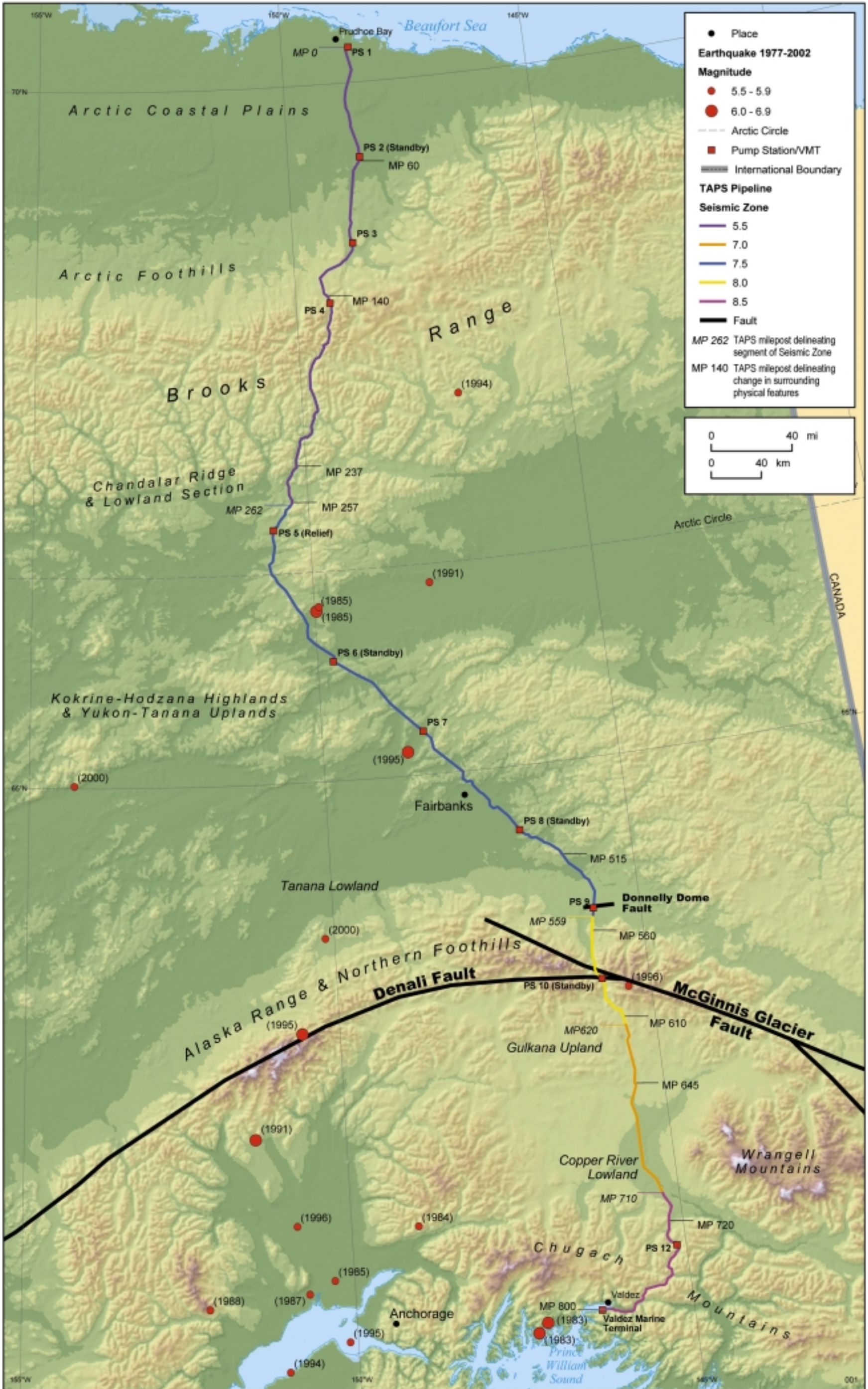
FIGURE 3.4-1 Seismic Zones and Fault Crossings along the TAPS and Locations of Earthquakes Greater Than 5.5 in Magnitude That Have Occurred near the TAPS since Startup (Source: TAPS Owners 2001a, Figure 3.1-10)
