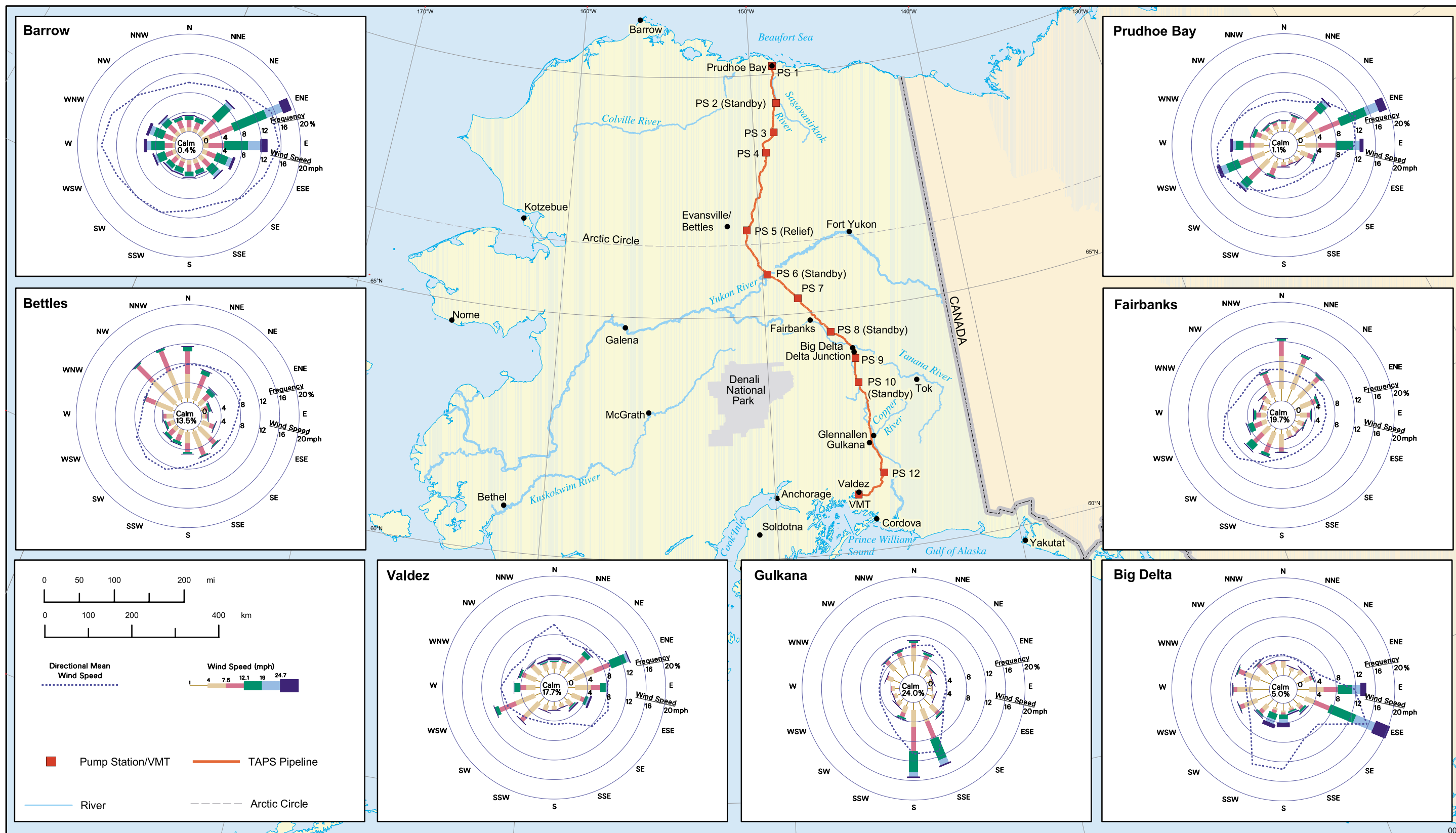
FIGURE 3.12-3 Wind Roses for Six National Weather Service Stations along the TAPS ROW and at Prudhoe Bay (Source: NCD 2001b; SECOR 1995)
