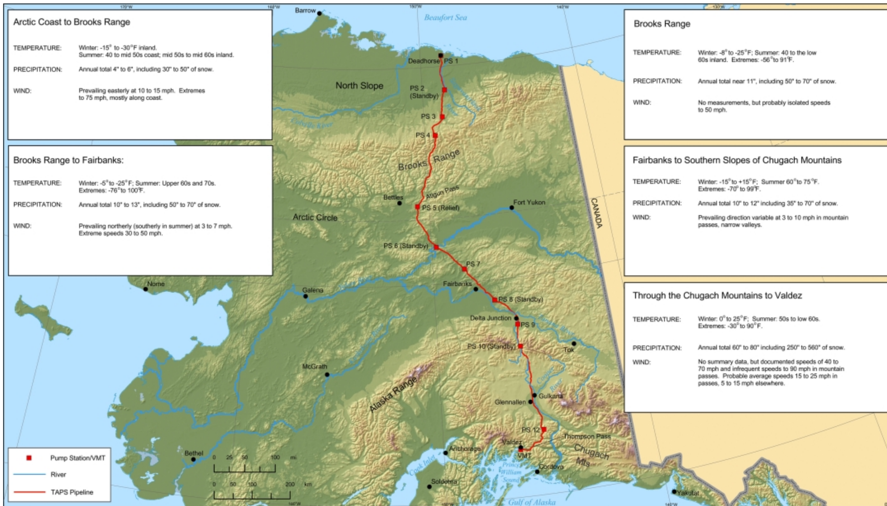
FIGURE 3.12-2 Summary of Climate along the TAPS ROW (Source: Modified from Searby 1968)
