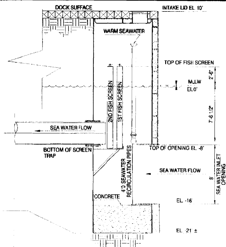
SIDE ELEVATION
