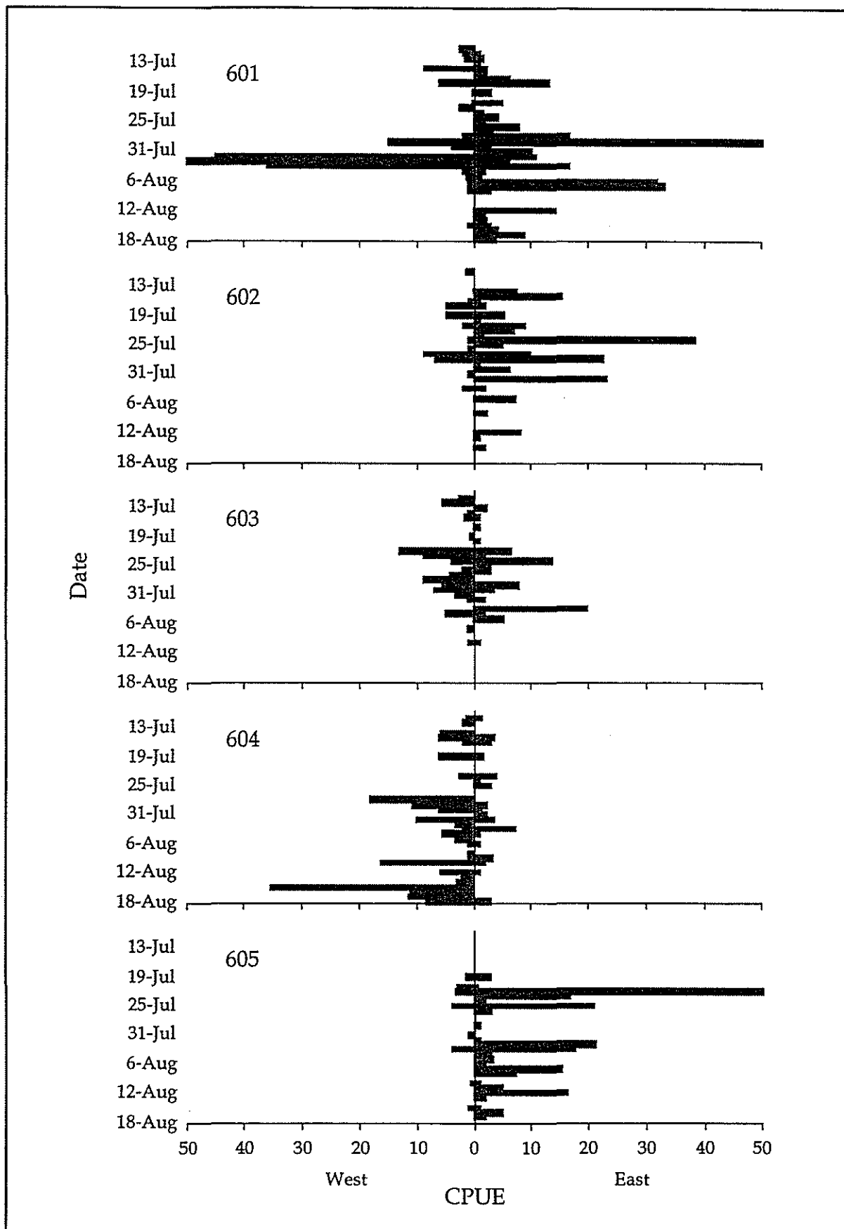
Figure 26. Catch-per-unit-effort (CPUE: fish/net/24 h) by side of net for Cohort 4 (≥age-3) Arctic cisco collected at Point Thomson through 18 August 1999 (the last sampling day prior to the end-of-season storm).
