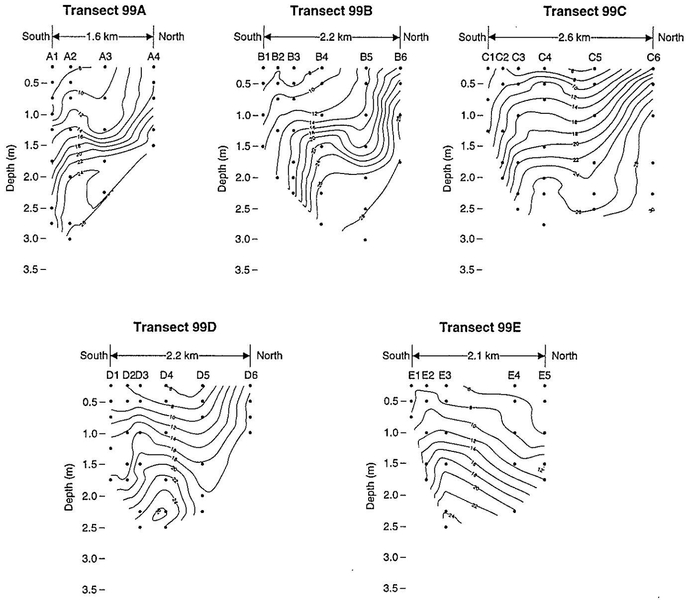
FIGURE E-11 1999 Physical Oceanography July 30, 1999 Salinity Transects (parts per thousand)
