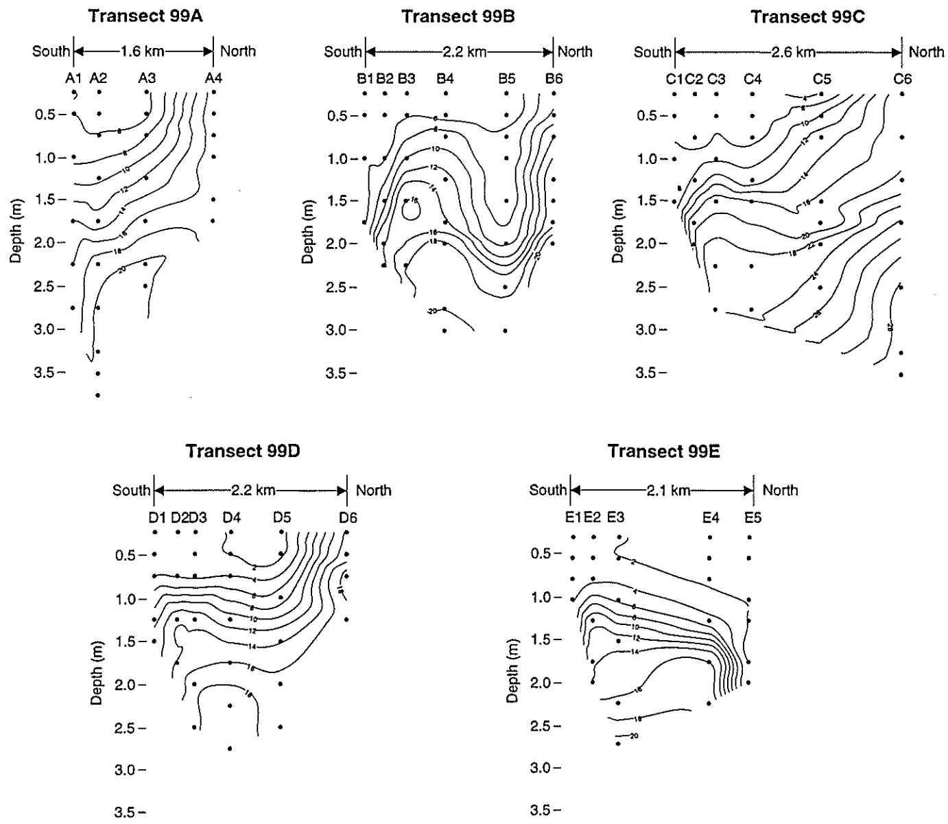
FIGURE E-9 1999 Physical Oceanography July 25, 1999 Salinity Transects (parts per thousand)
