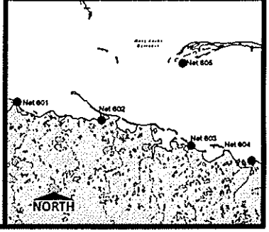
FIGURE G-1 1999 Physical Oceanography July 6, 1999 Salinity (parts per thousand) Surf Zone Transects Notes: Base map was digitized from USGS 1:63360 Topographic Map by BPXA Cartography.
