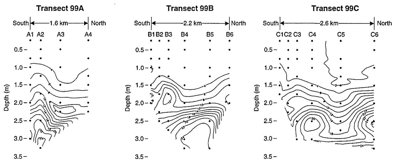
FIGURE E-2 1999 Physical Oceanography July 9, 1999 Salinity Transects (parts per thousand)
