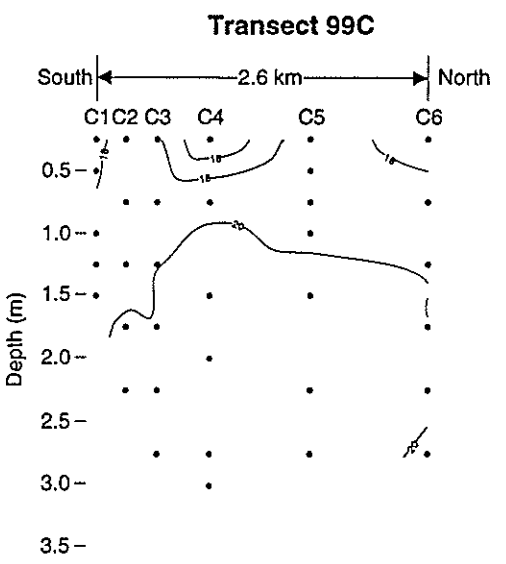
FIGURE E-6 1999 Physical Oceanography July 19, 1999 Salinity Transects (parts per thousand)
