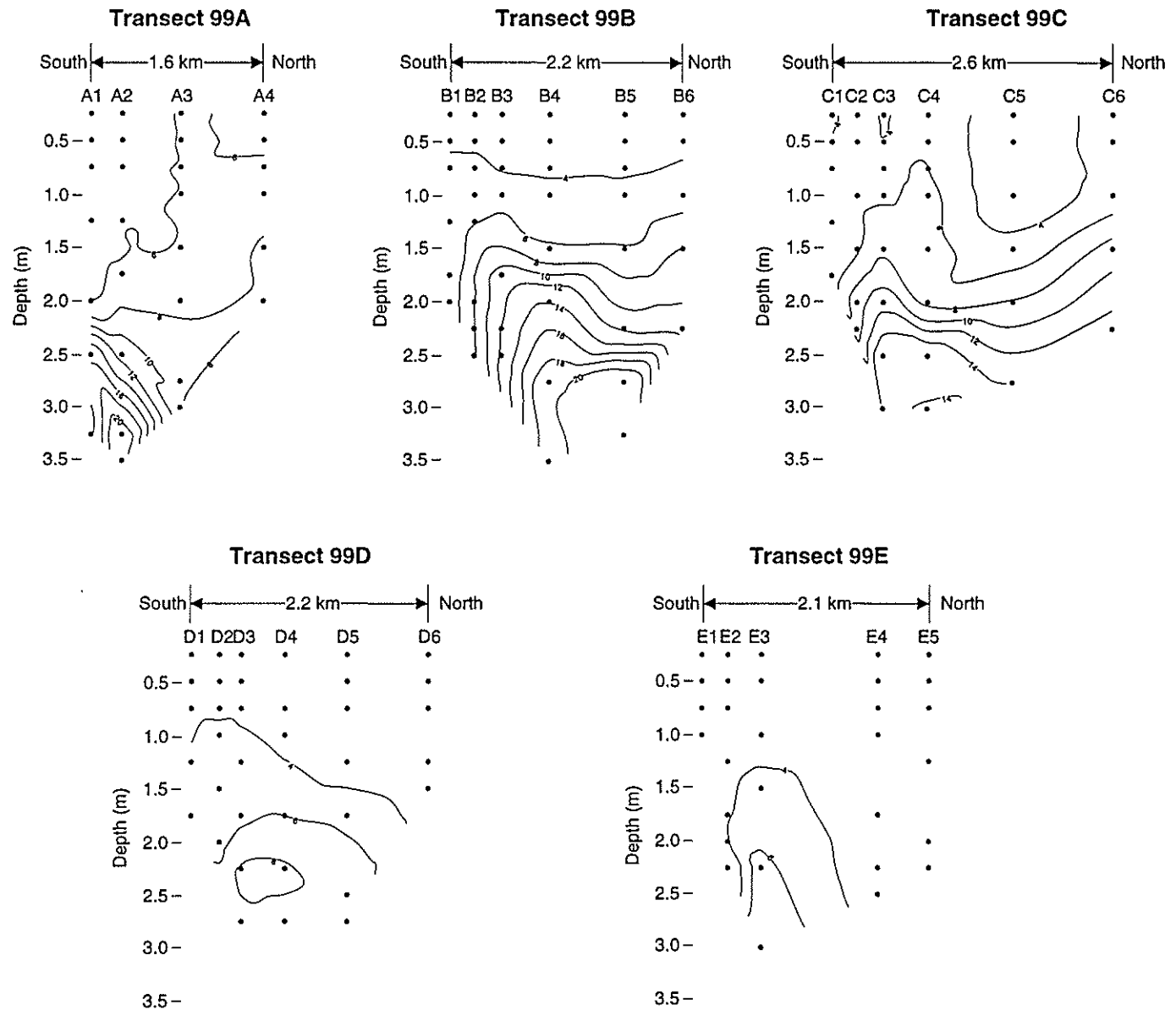
FIGURE E-3 1999 Physical Oceanography July 12, 1999 Salinity Transects (parts per thousand)
