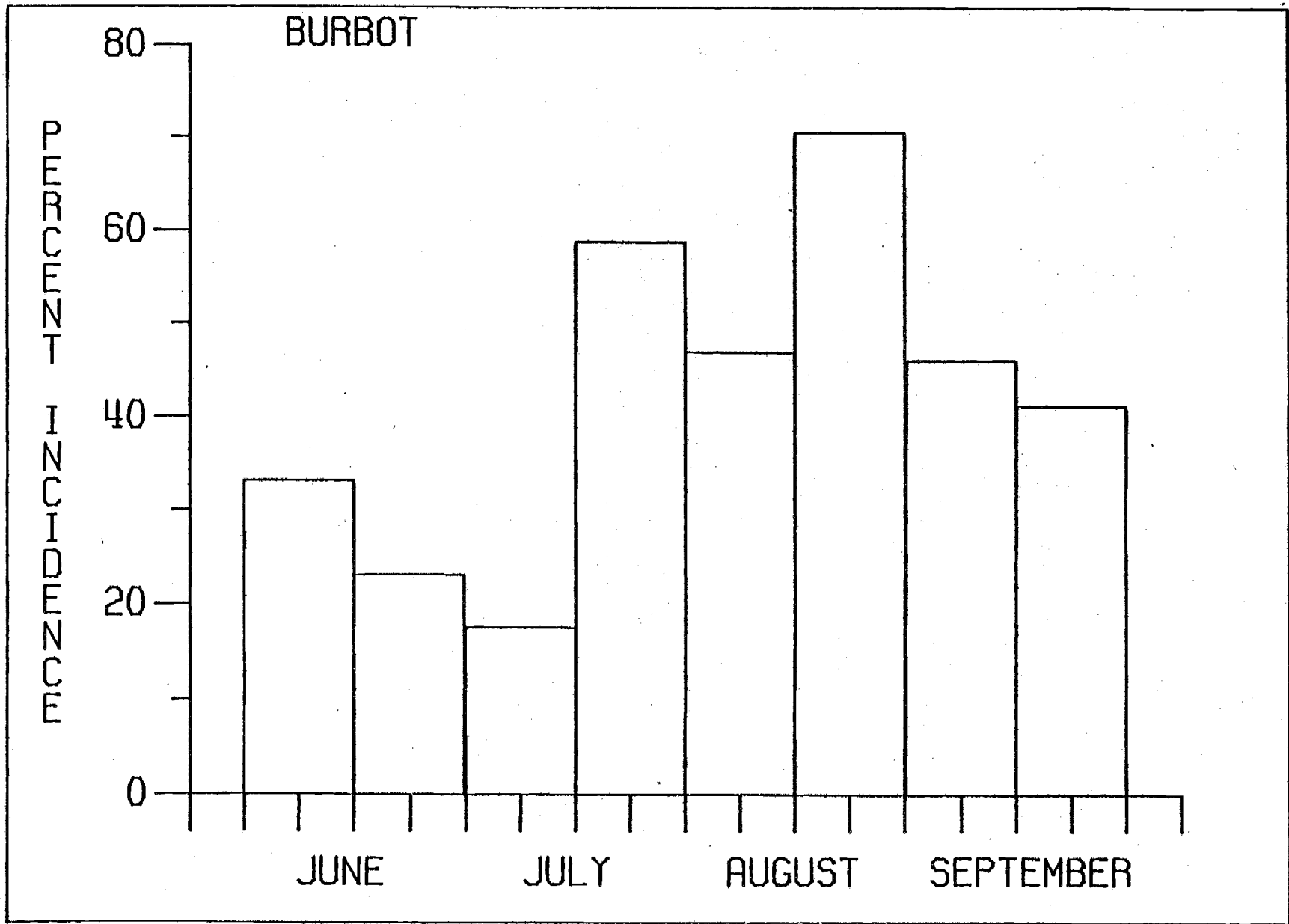
Figure E.3.3.2. Percent incidence of burbot captured at habitat location sites on the Susitna River between Talkeetna and Devil Canyon, June to September, 1981.
