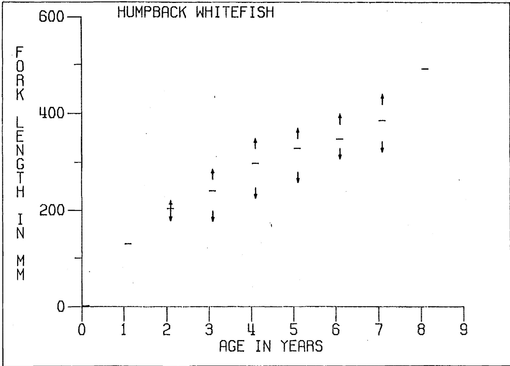
Figure E.3.5.3. Age and length relationship for humpback whitefish captured at habitat location sites on the Susitna River between Cook Inlet and Devil Canyon, June to October, 1981. The mean length for each age class is indicated by a horizontal bar and the range is indicated by arrows.
