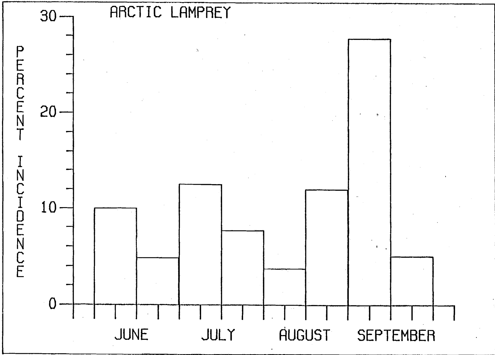
Figure E.3.11.1. Percent incidence of Arctic lamprey captured at habitat location sites on the Susitna River between Cook Inlet and Talkeetna, June to September, 1981.
