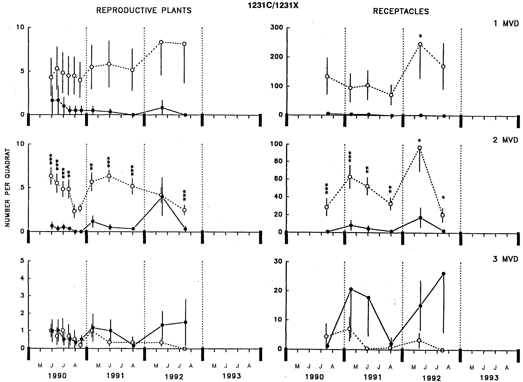
Figure 2.9. The number of reproductive Fucus plants and receptacles per quadrat at the 1231C/1231X site pair.
