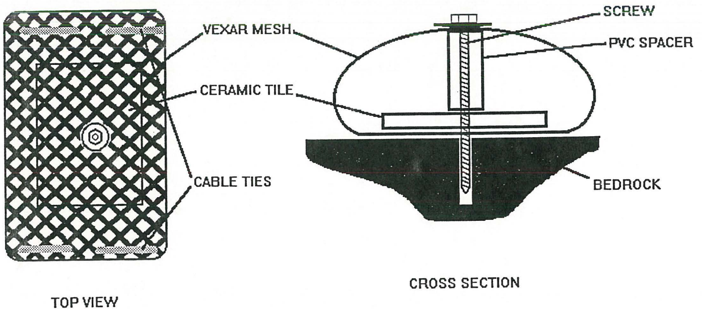
Figure 2.1. Schematic diagram of a ceramic Fucus recruitment tile and the vixar cage used to manipulate herbivores. To control for cage effects the cable ties were left off of one end of the vixar cage such that that end of the cage was open to herbivores.
