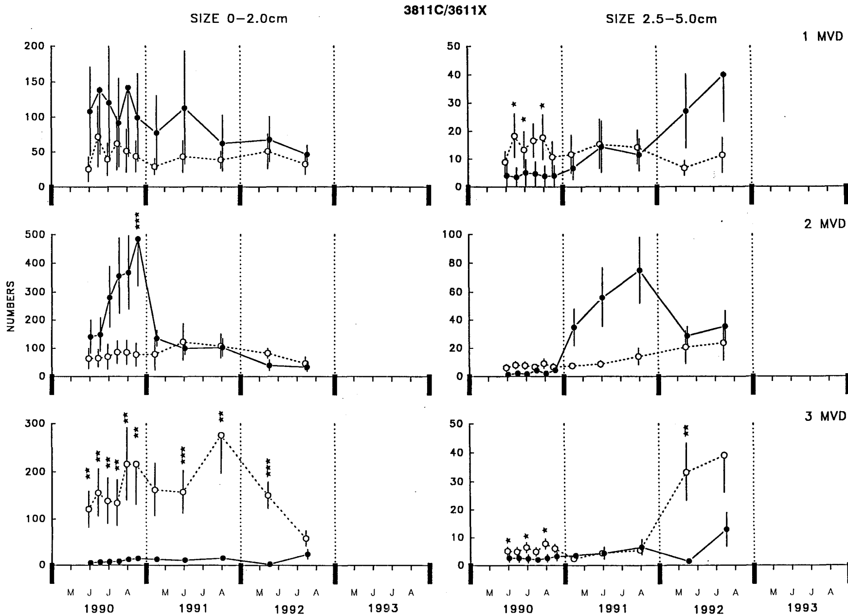
Figure 2.8. The number of Fucus germlings and small plants at the 3811C/3611X site pair. Event is the same
