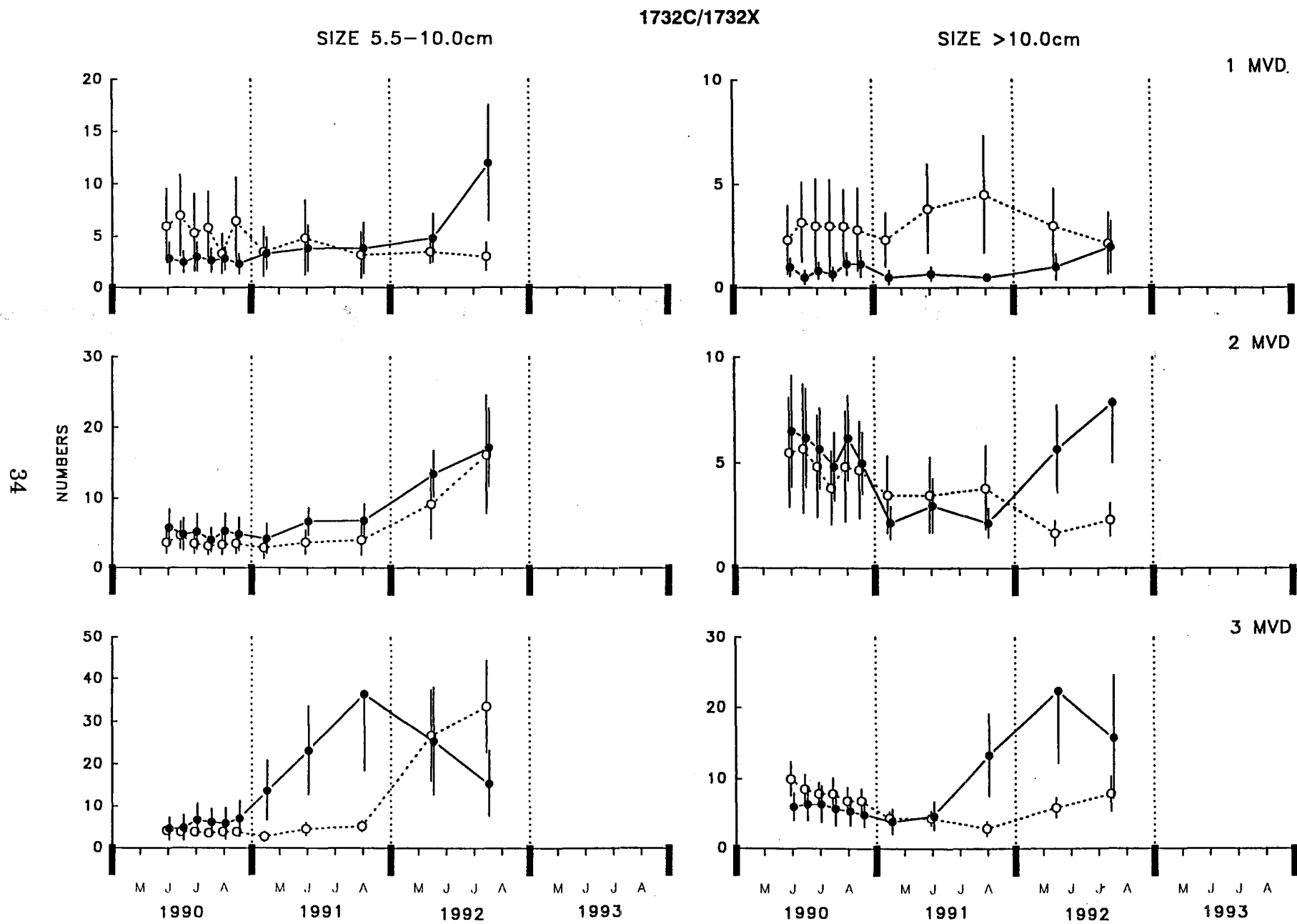
Figure 2.5. The number of medium and large Fucus plants at the 1732C/1732X site pair. Layout is the same as
