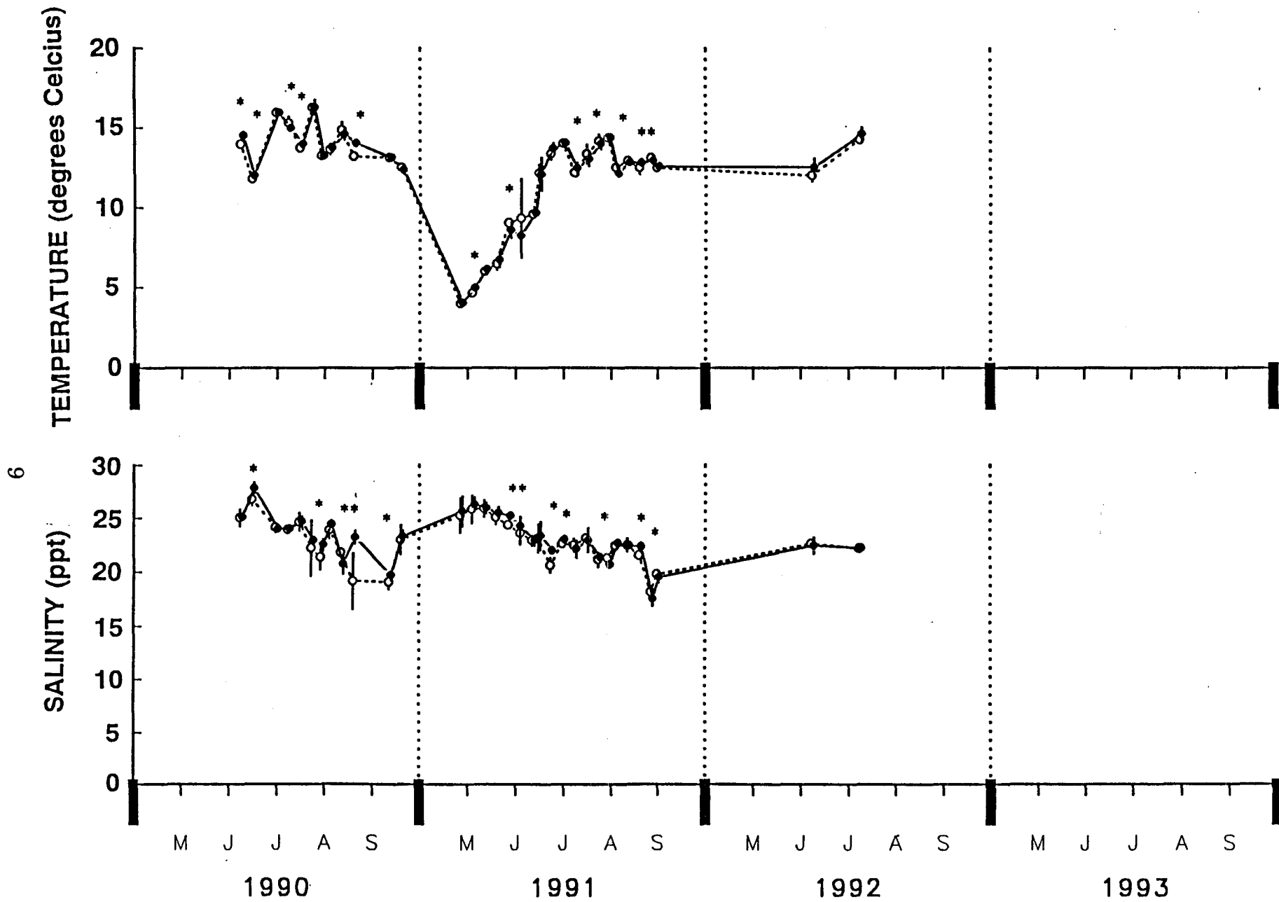
Figure 1.3. The temperature and salinity at 1 meter depth at oiled and control areas of Herring Bay. Error bars represent one standard deviation, and
