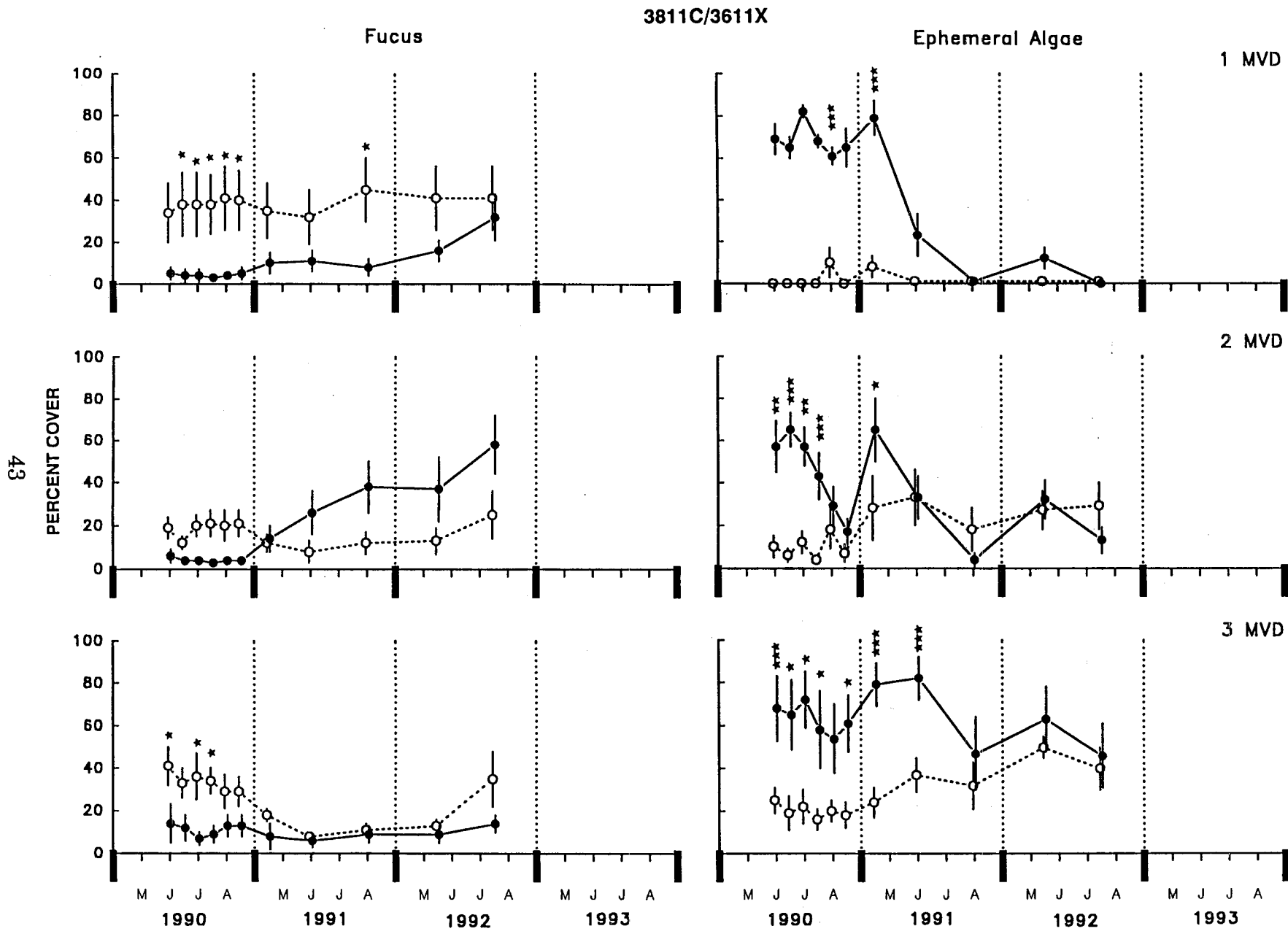
Figure 2.14. The percent cover of Fucus and ephemeral algae at the 3811C/3611X site pair. Layout is the same
