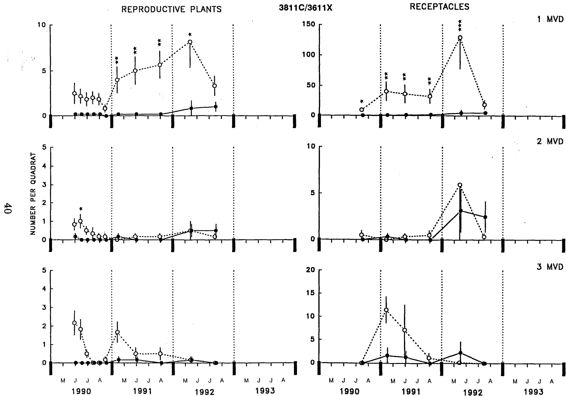
Figure 2.11. The number of reproductive Fucus plants and receptacles per quadrat at the 3811C/3611X site pair. Layout is the same as Figure 2.3.
