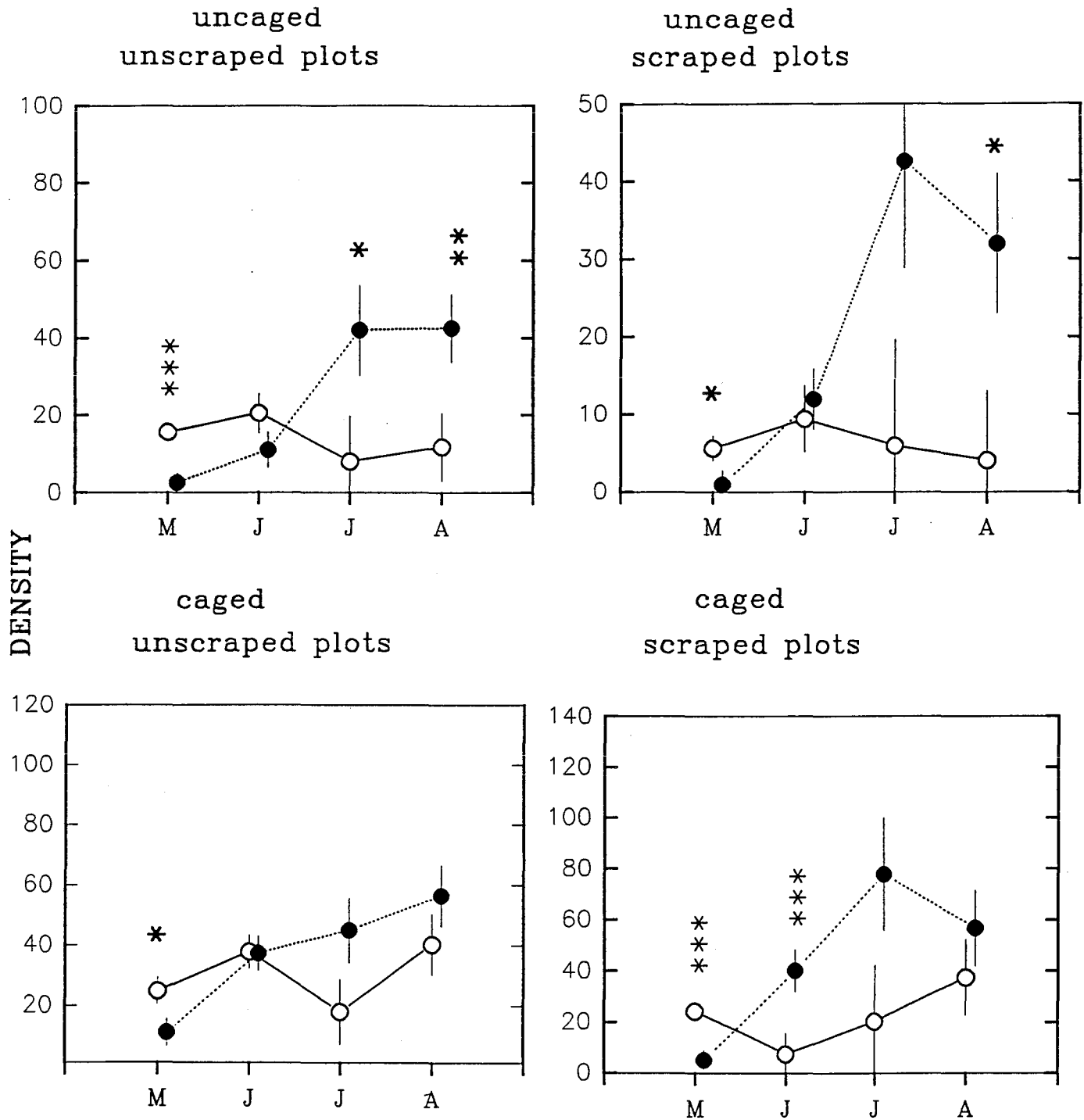
Figure 3.61. Density (No./0.01 m 2 ) of barnacle juveniles compared between control and oiled sites on unscrapped and scraped plots during 1992. Treatments also included caged and uncaged plots. N=3 for each treatment. Control sites are open circles connected by solid lines. Oiled sites are solid circles connected by dotted lines. There were 4 sample dates in 1992 between 5/31 and 8/27. Months are represented by letters on the X-axis. The asterisks represent statistical significance from ANOVA, blocking control and oiled sites (*=p≤0.05, **=p≤0.025, ***=p≤0.01).
