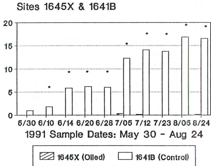
Figure 3.87. Density (No./0.01 m 2 ) of grazers (limpets and littorines) in 1991 compared between oiled and control plots. The '*' represents significance ( p \leq 0.05 -ANOVA). Site 1641B served as the control for oiled sites 1645X and 1746X.
