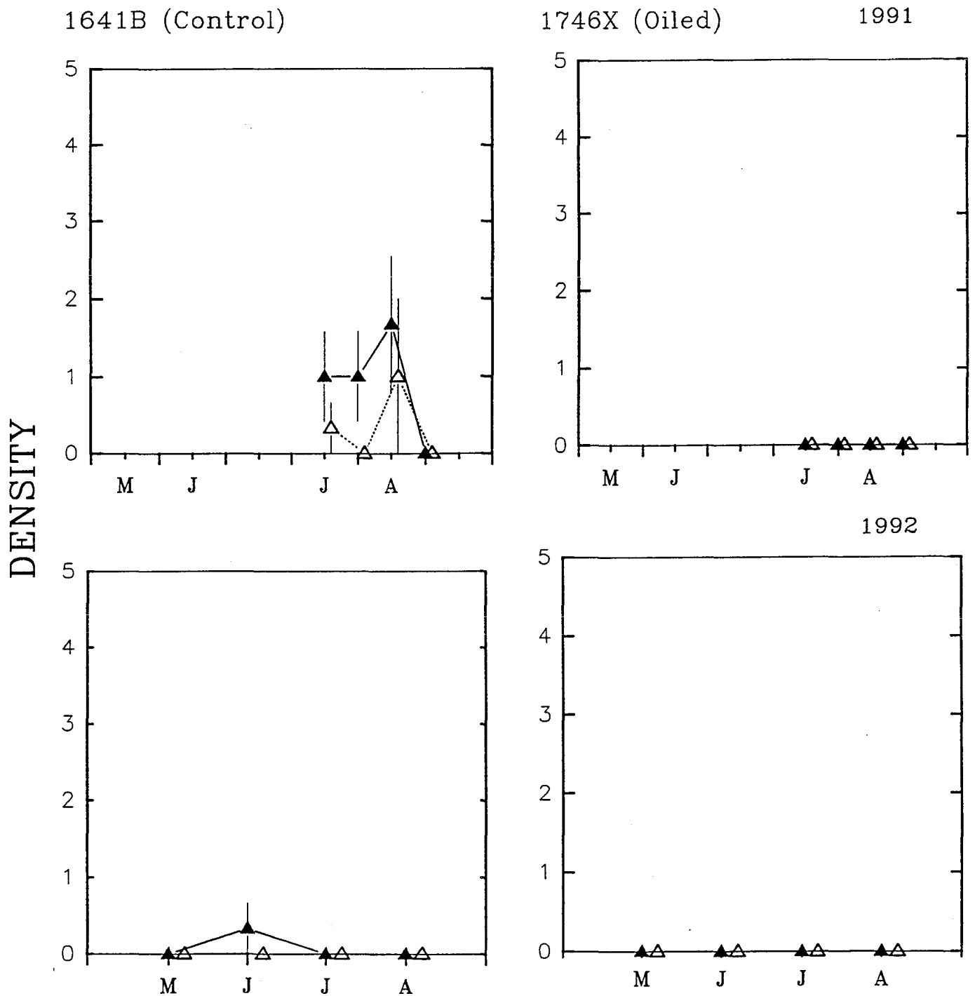
Figure 3.77. Density (No./0.01 m 2 ) of Fucus germlings that settled on uncaged, tarred and scraped vertical rock faces at site pair 1746X during spring-fall 1991-1992. Site 1641B serves as the control match for this pair. Sampling of this site began in July, 1991. Layout same as Figure 3.48. N=3.
