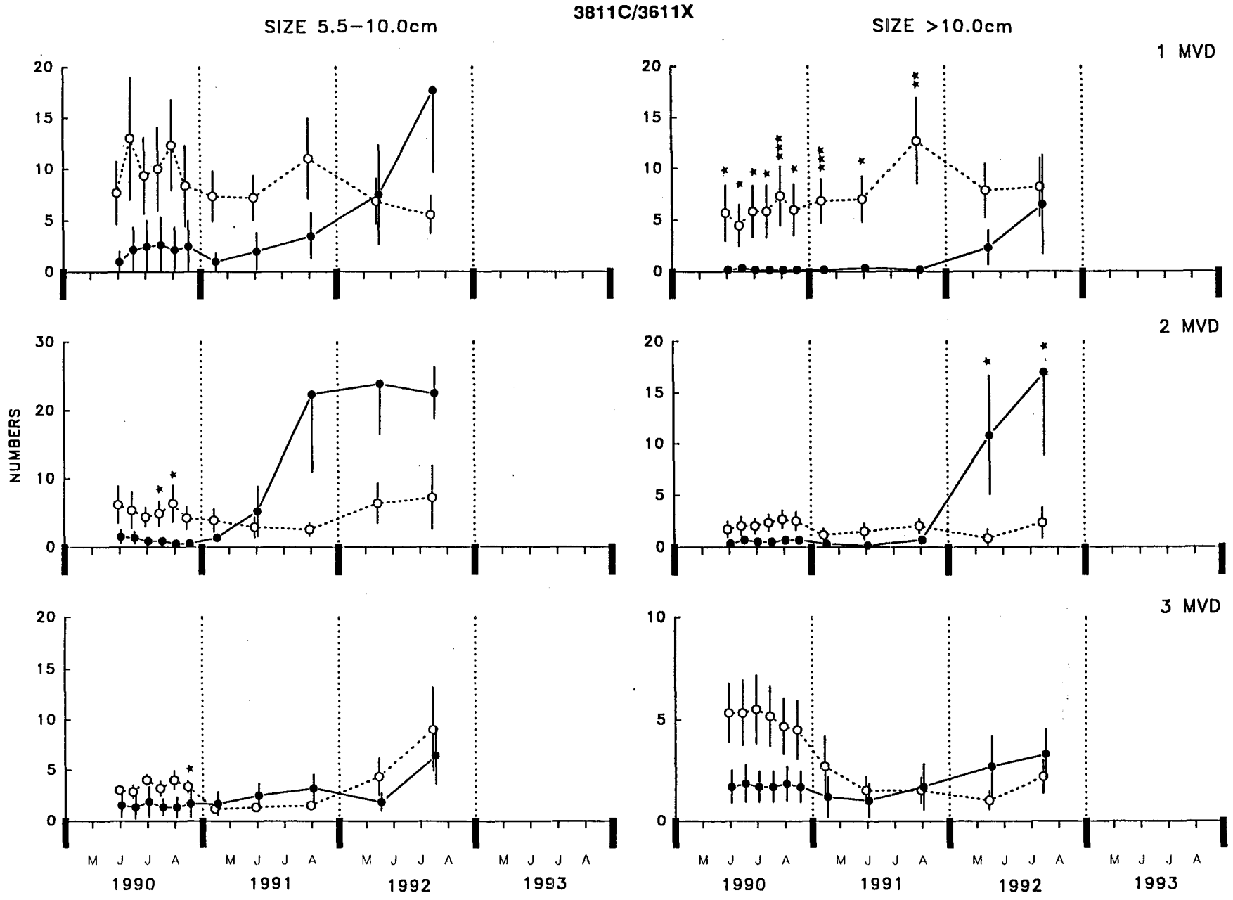
Figure 2.7. The number of medium and large Fucus plants at the 3811C/3611X site pair. Lavout is the same as
