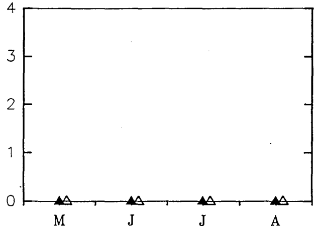
Figure 3.72. Density (No./0.01 m 2 ) of Fucus germlings that settled on uncaged, tarred and scraped vertical rock faces at site pair 1641 during spring-fall 1990-1992. N=5 for 1990. N=3 for 1991 and 1992. Layout same as Figure 3.48. Note scale differences.
