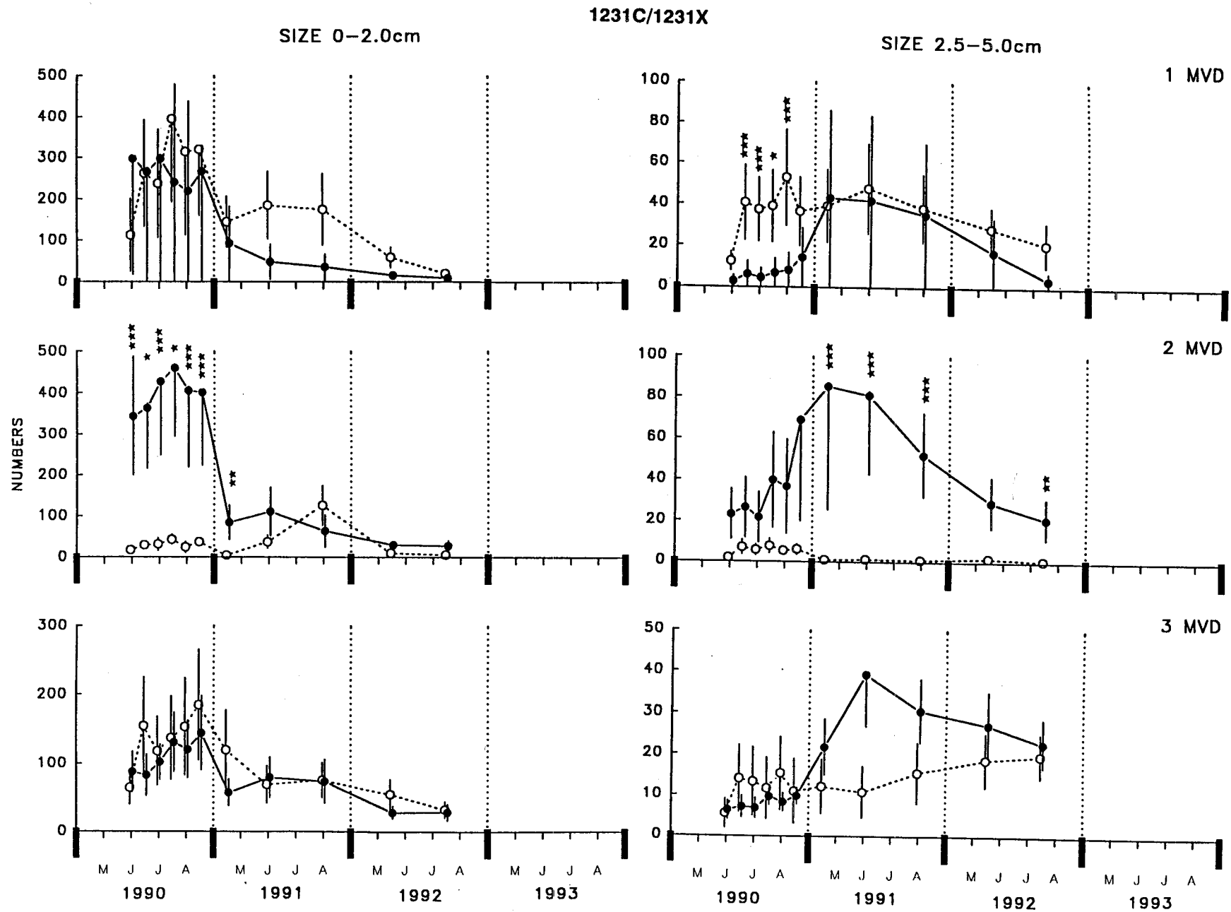
Figure 2.4. The number of Fucus germlings (0-2.0 cm) and small (2.5-5.0 cm) plants at the 1231C/1231X site near. Layout is the same as Figure 2.2
