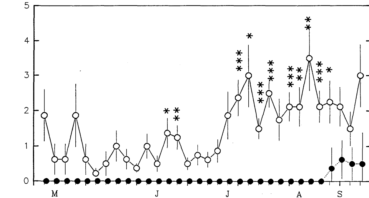
Figure 3.83. Density (No./0.01 m 2 ) of Fucus germlings compared between control and oiled sites on unscraped and scraped plots during 1990. All plots were unscraped. Control sites are open circles connected by solid lines. Oiled sites are solid circles connected by dotted lines. Error bars represent plus and minus one standard error of the mean. There were 32 sample dates in 1990 between 5/30 and 9/21. Months are represented by letters on the X-axis. The asterisks represent statistical significance from ANOVA, blocking control and oiled sites (*= p \leq 0.05 , **= p \leq 0.025 , ***= p \leq 0.01 ).
