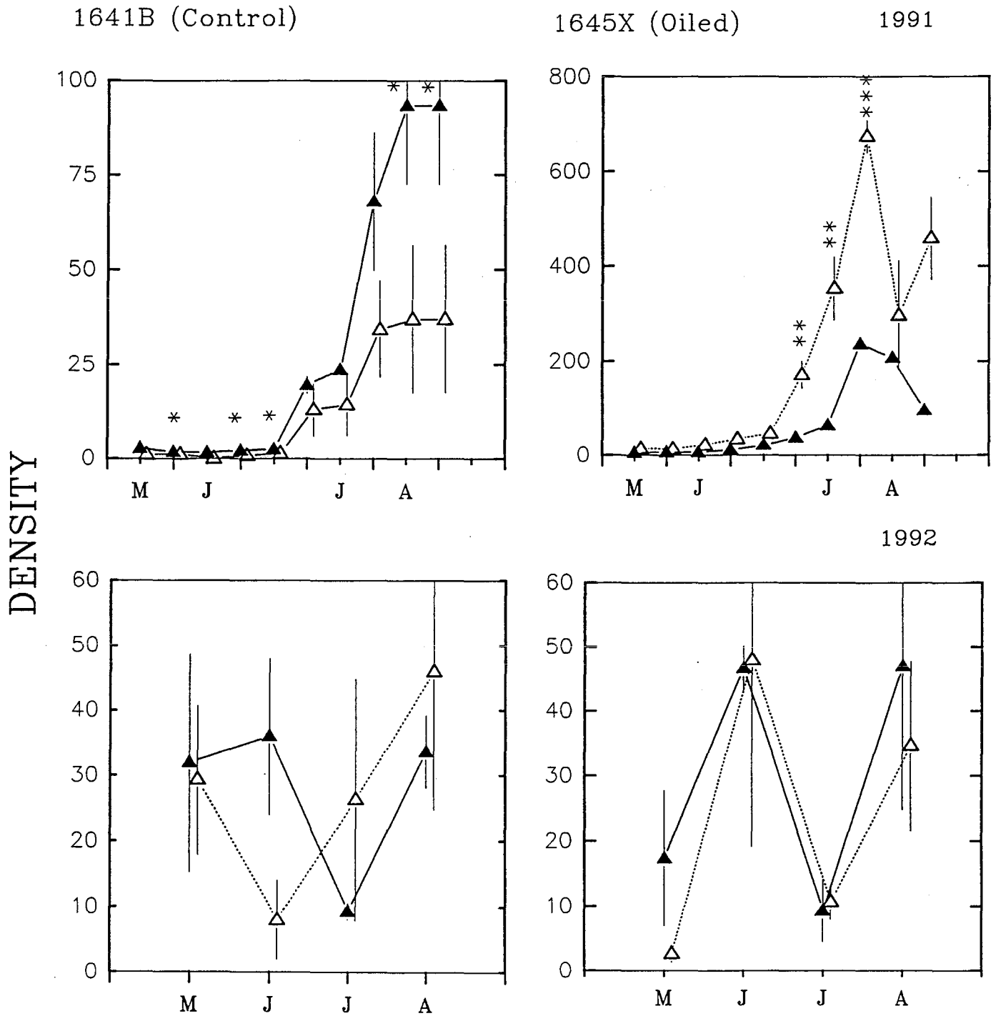
Figure 3.57. Density (No./0.01 m 2 ) of barnacle recruits that settled on caged, tared and scraped vertical rock faces at site pair 1645X during spring-fall 1991-1992. Site 1641B serves as the control match for this pair. Layout same as Figure 3.48. N=3.
