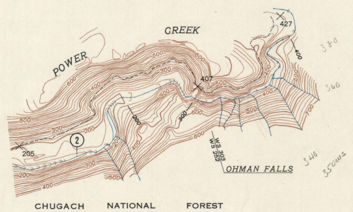
DAM SITE (MILE 2.7 SHEET 1)
