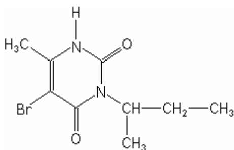
Bromacil Chemical Structure
