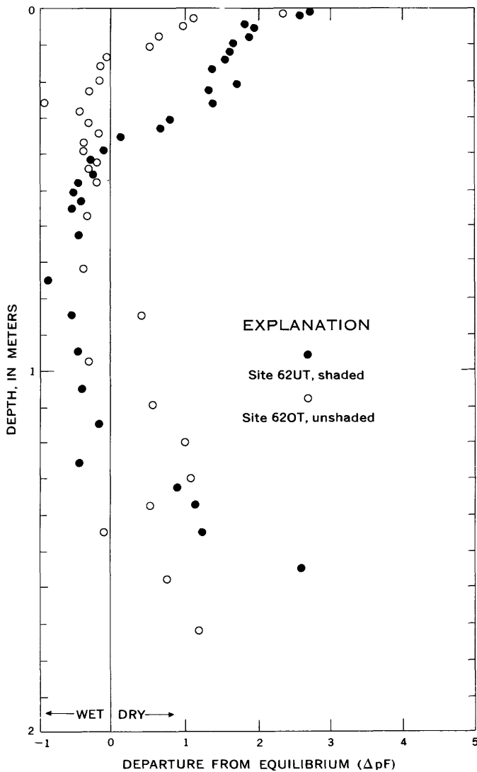
FIGURE 23.—Profiles of \Delta pF for shaded and unshaded sites 62UT and 62OT associated with saltcedar trees near section 11 of the Gila River Phreatophyte Project area. Sampled May 30, 1962.
