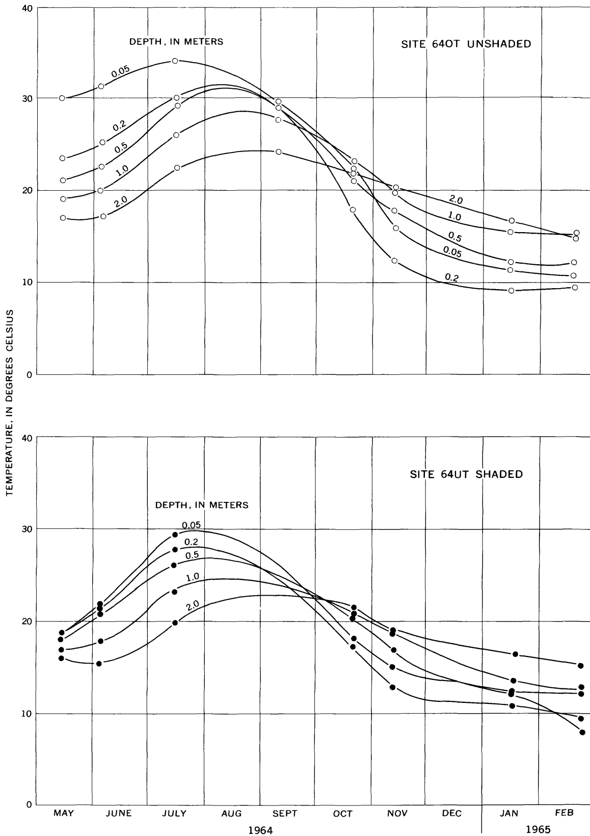
FIGURE 11.—Seasonal temperature fluctuations at selected depths for the period May 15, 1964, to February 25, 1965, at sites 640T and 64UT near section 23 of the Gila River Phreatophyte Project area. Measurements were obtained with thermistors in experimental moisture-stress measuring columns.
