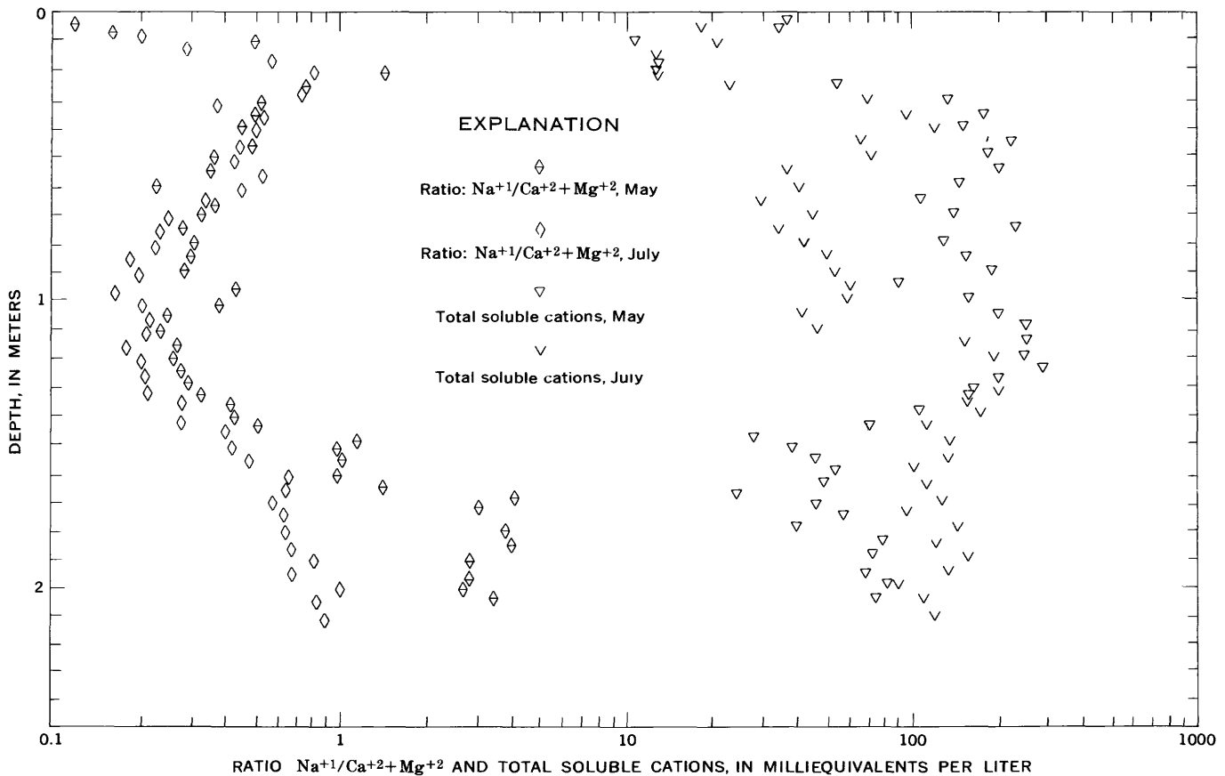
FIGURE 15.—Logarithmic profiles of the ratio of monovalent to divalent cations and the TSC for unshaded site 640T associated with saltcedar trees near section 23 of the Gila River Phreatophyte Project area. Sampled May 10 and July 16, 1964.
