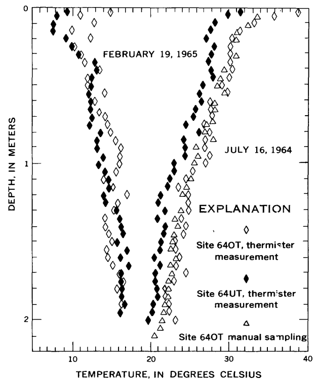
FIGURE 10.—Soil-temperature profiles obtained with thermisters in experimental moisture-stress measuring columns installed at sites 64OT and 64UT near section 23 of the Gila River Phreatophyte Project area. A temperature profile obtained by manual sampling methods at the unshaded site 64OT is included for comparison of methods. Measurements were obtained on July 16, 1964, and February 19, 1965.
