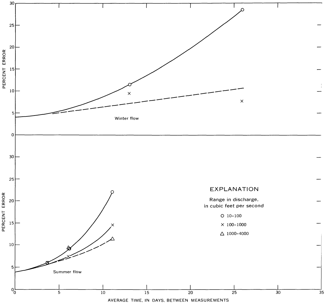
FIGURE 10.—Standard error of computed discharge for different ranges of discharge, Gila River at Calva.
