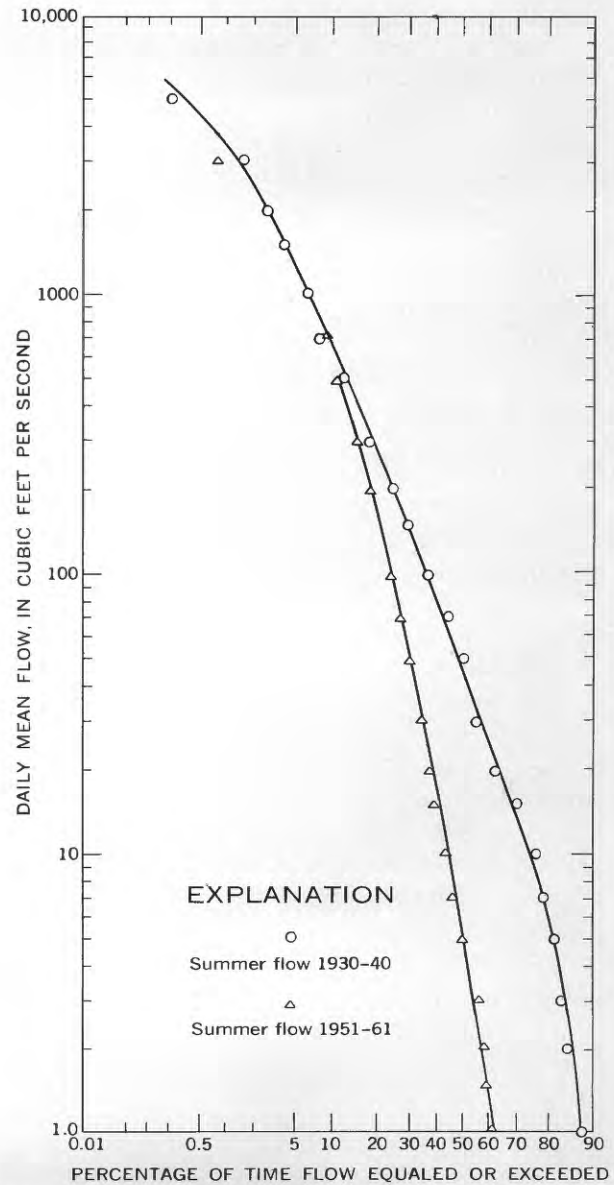
FIGURE 6.—Duration curves of summer flow, 1930–40 and 1951–61, Gila River at Calva.
