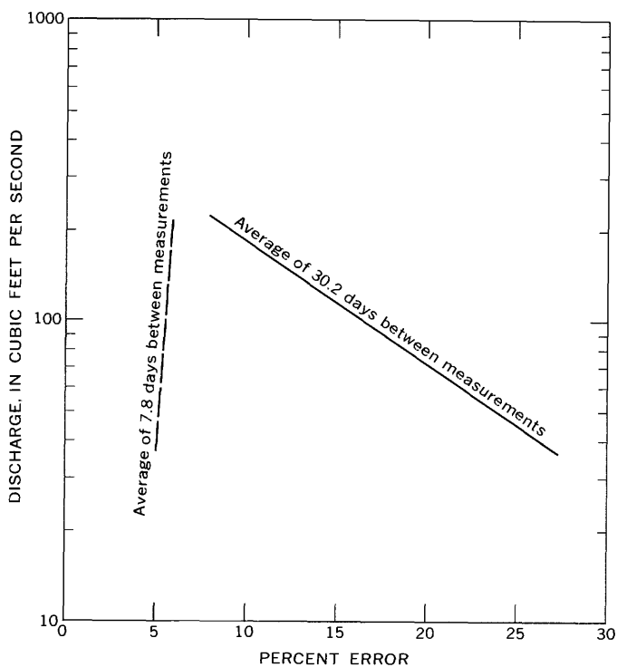
FIGURE 14.—Standard error of computed discharge for winter flow, Gila River at Calva.
