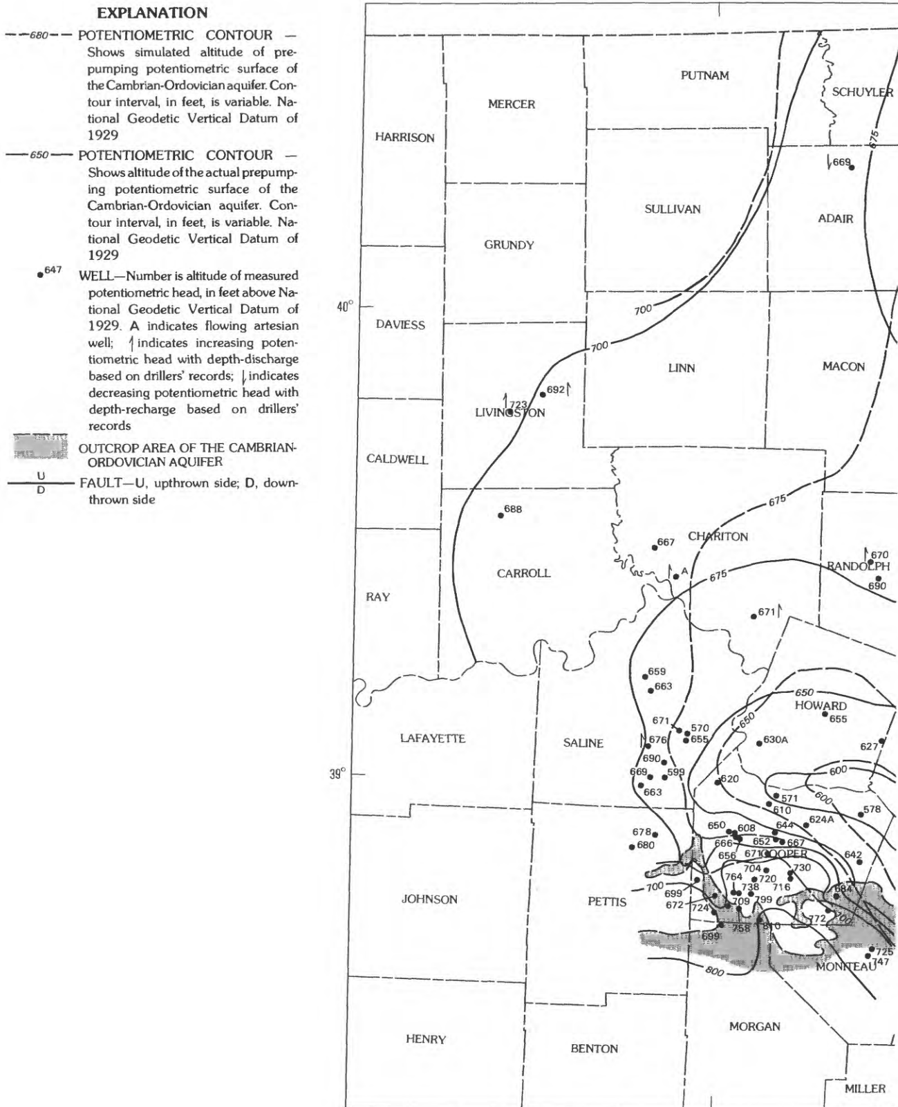
FIGURE 22.—Altitude of the simulated and actual prepumping potentiometric surfaces of the Cambrian-Ordovician aquifer.
