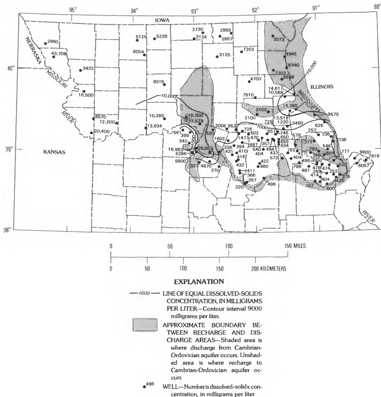
FIGURE 17.—Areas of recharge and discharge and the dissolved-solids concentration in the Cambrian-Ordovician aquifer.
