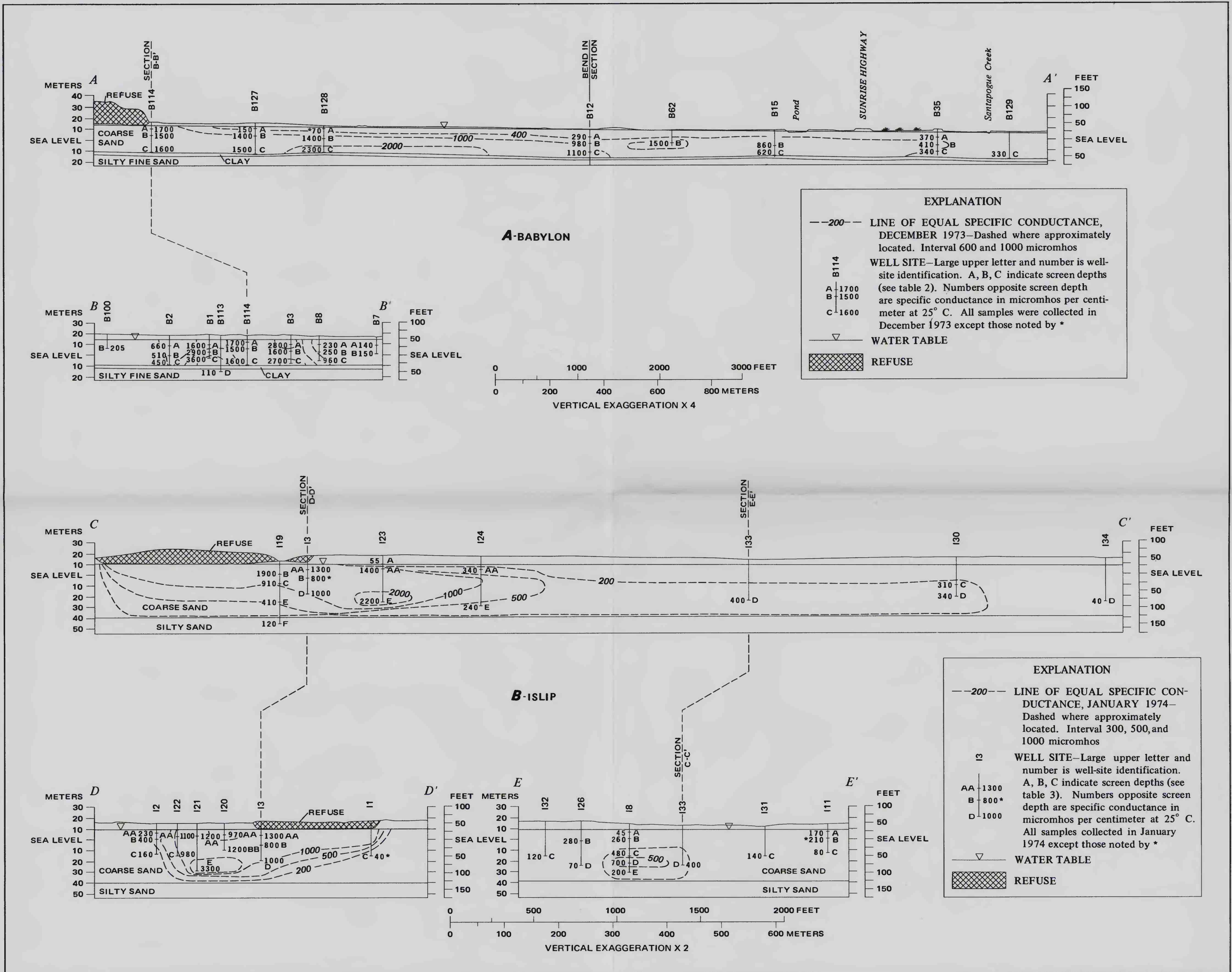
HYDROCHEMICAL SECTIONS THROUGH THE PLUMES OF LEACHATE-ENRICHED GROUND WATER AT BABYLON AND ISLIP LANDFILLS, LONG ISLAND, NEW YORK
