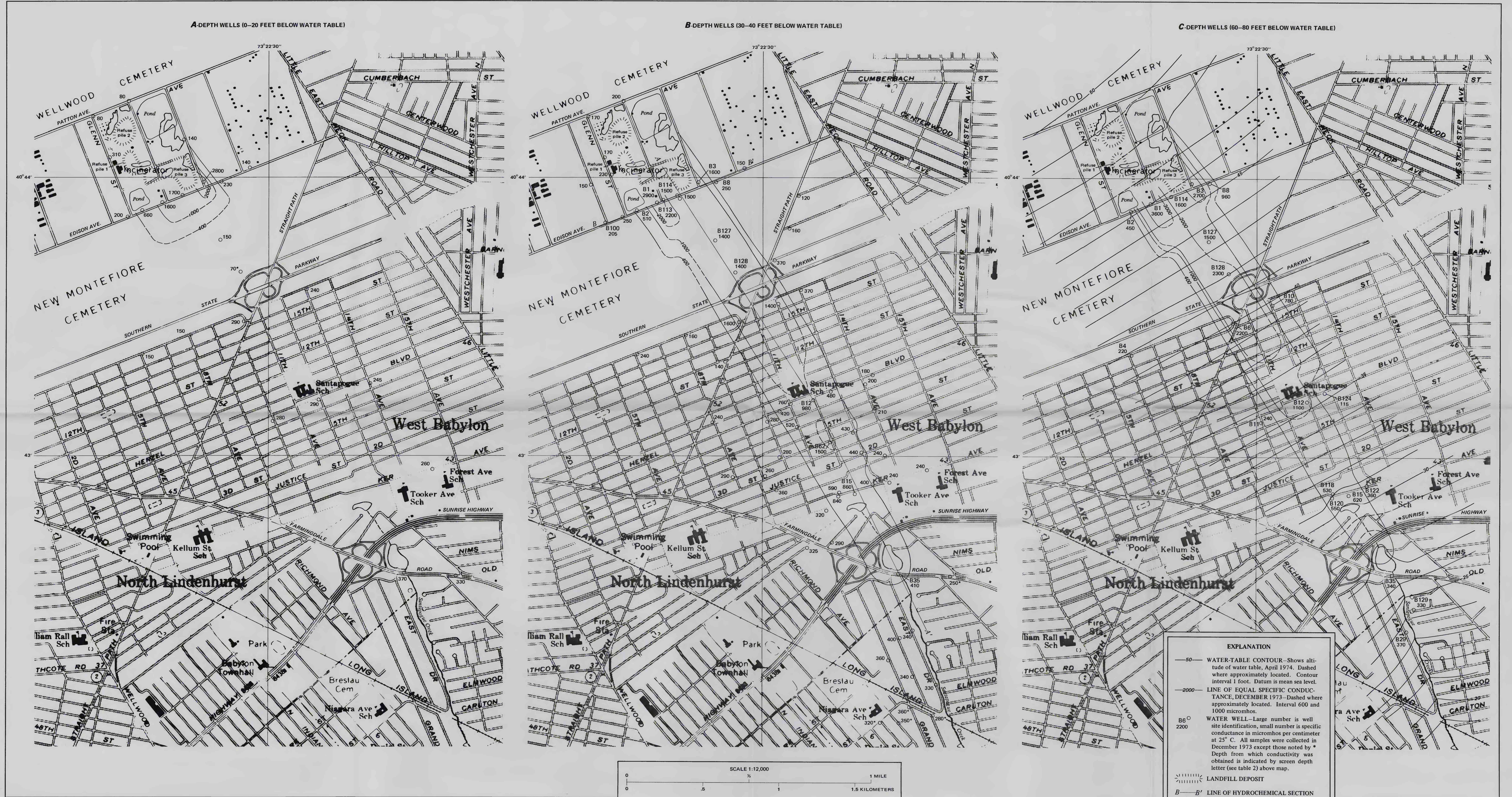
SPECIFIC CONDUCTANCE IN AND NEAR THE PLUME OF LEACHATE-ENRICHED GROUND WATER DOWNGRADIENT FROM BABYLON LANDFILL
