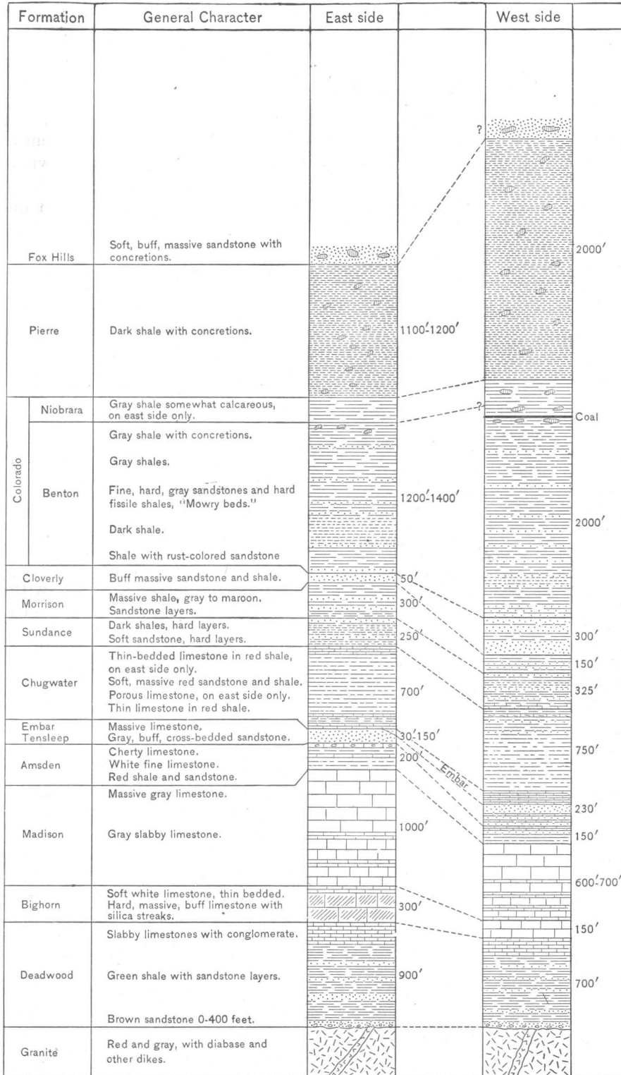
COLUMNAR SECTIONS EAST AND WEST SIDES BIGHORN BASIN By C. A. FISHER
