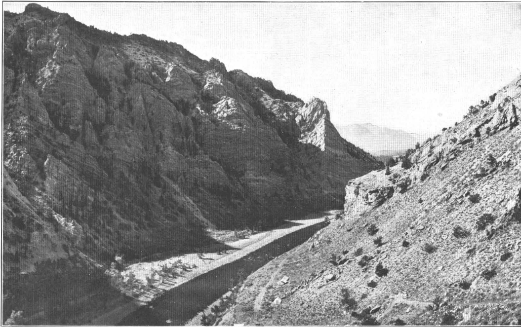
A. MASSIVE BEDS OF MADISON LIMESTONE OVERLAIN BY SOFTER AMSDEN SHALES. Upper end of Shoshone Canyon above dam site.
