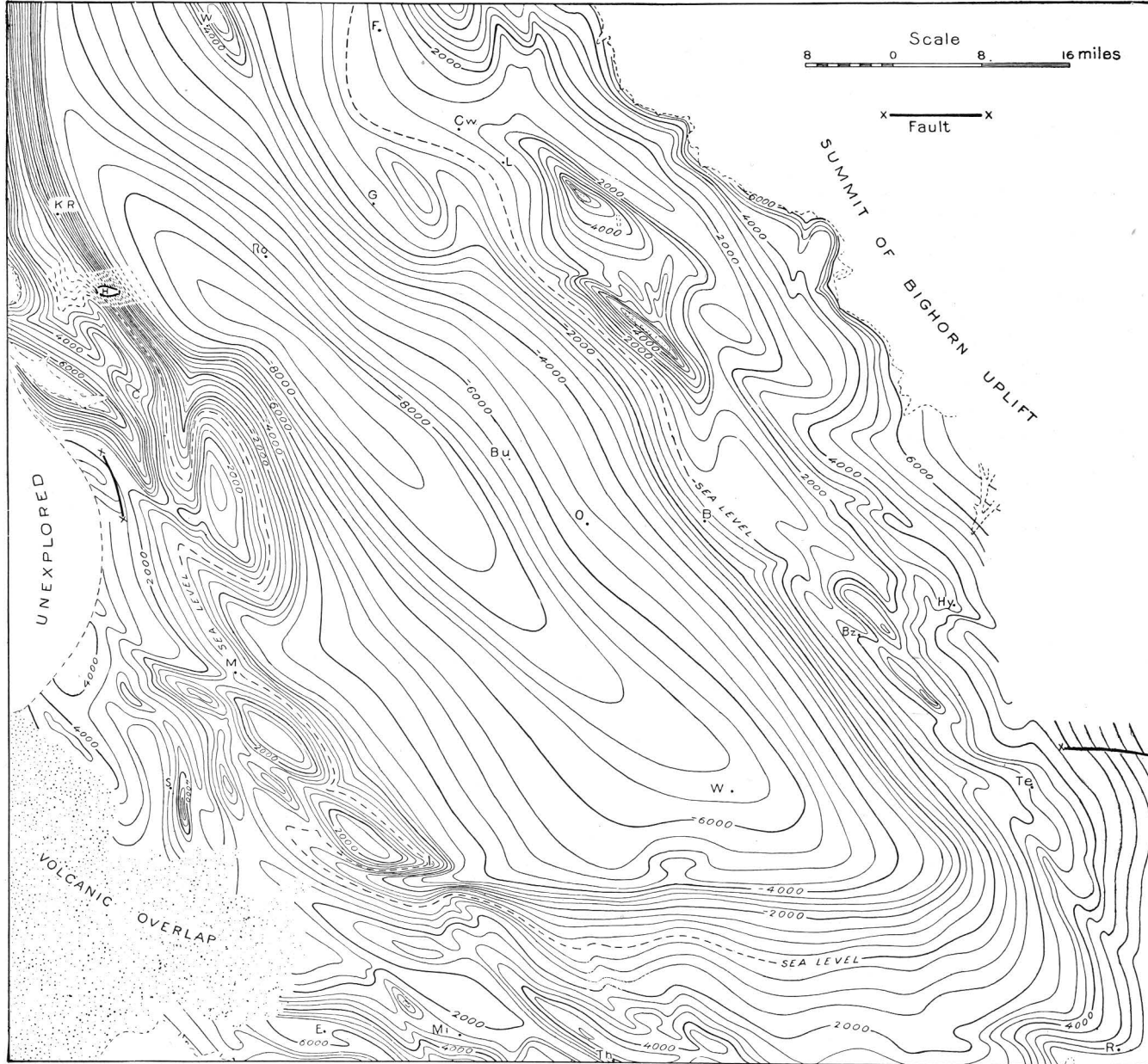
DIAGRAM OF STRUCTURE OF THE BIGHORN BASIN, WYOMING.
