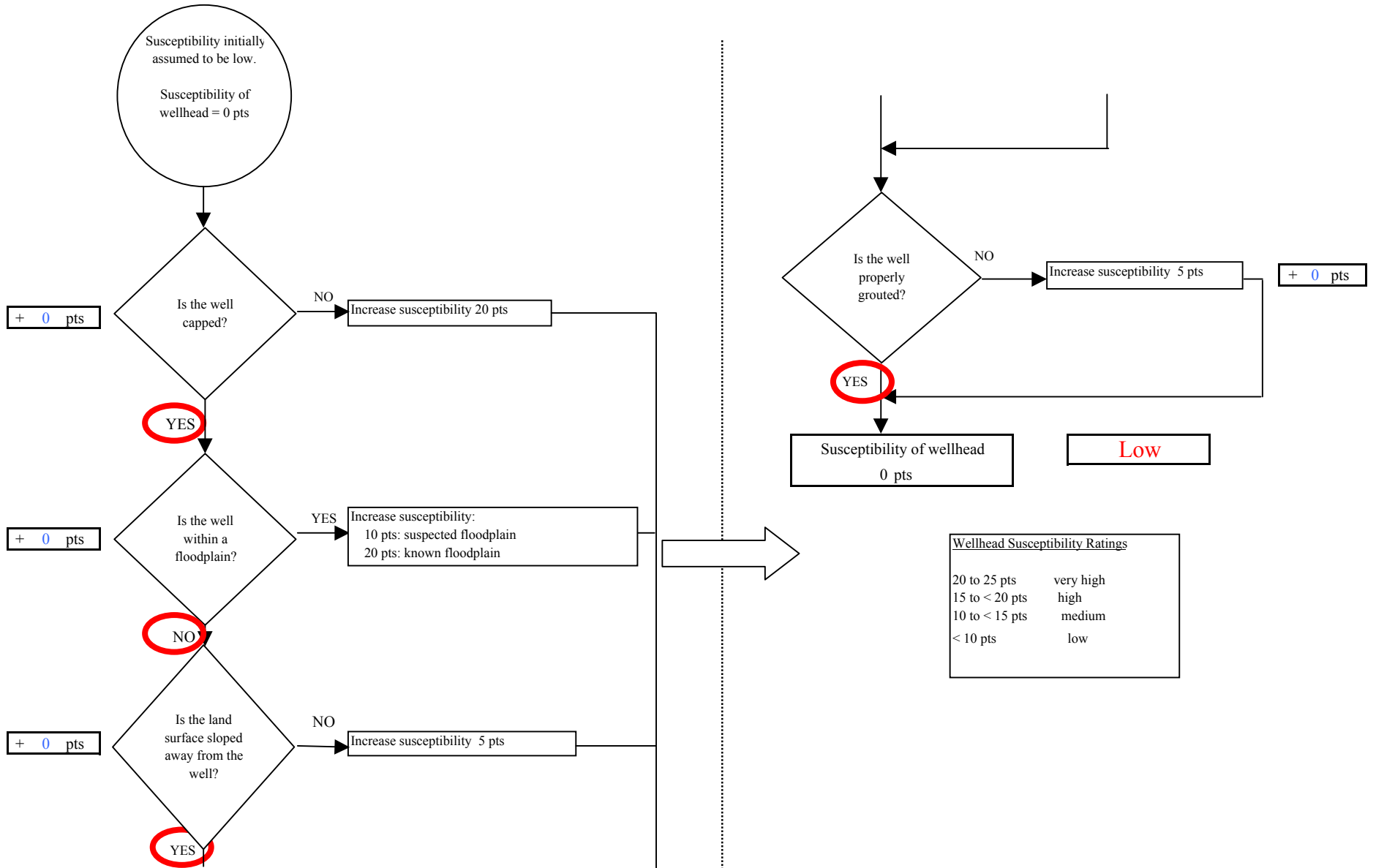
Chart 1. Susceptibility of the wellhead - Valley Lanes
