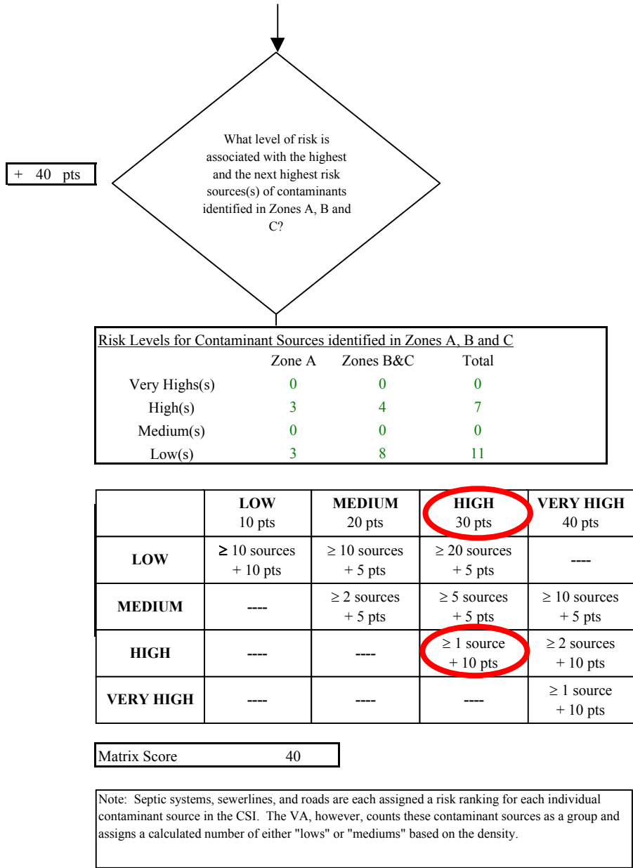
Chart 5. Contaminant risks for Valley Lanes - Nitrates and Nitrites
