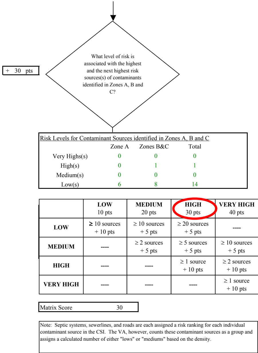
Chart 7. Contaminant risks for Valley Lanes - Volatile Organic Chemicals
