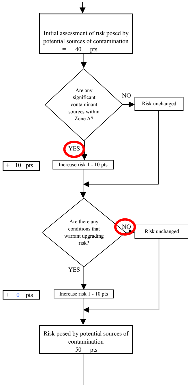
Chart 3. Contaminant risks for Valley Lanes - Bacteria & Viruses
