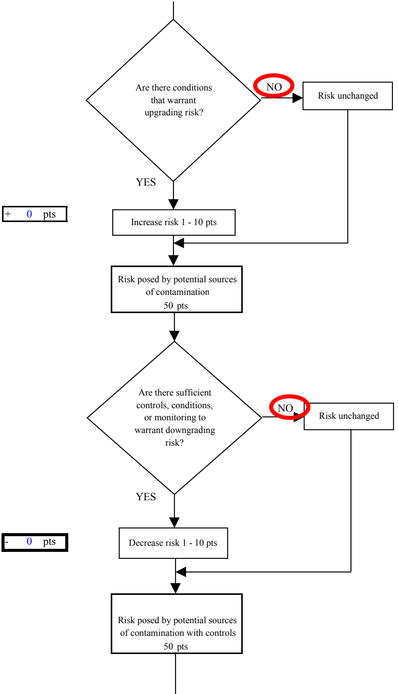
Chart 5. Contaminant risks for Valley Lanes - Nitrates and Nitrites
