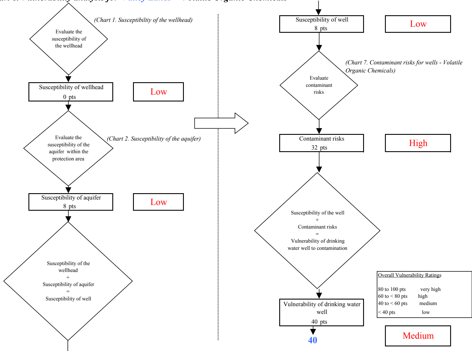
Chart 8. Vulnerability analysis for Valley Lanes - Volatile Organic Chemicals
