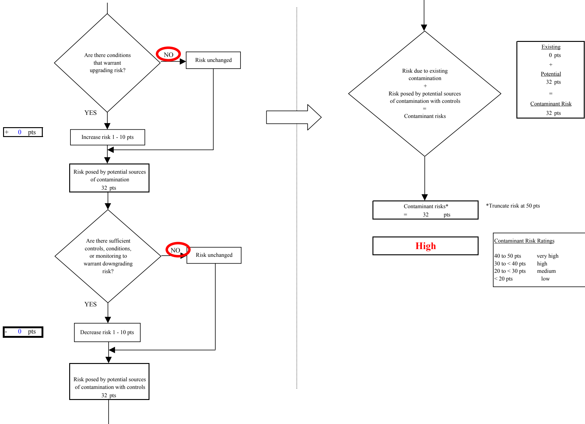
Chart 7. Contaminant risks for Valley Lanes - Volatile Organic Chemicals
