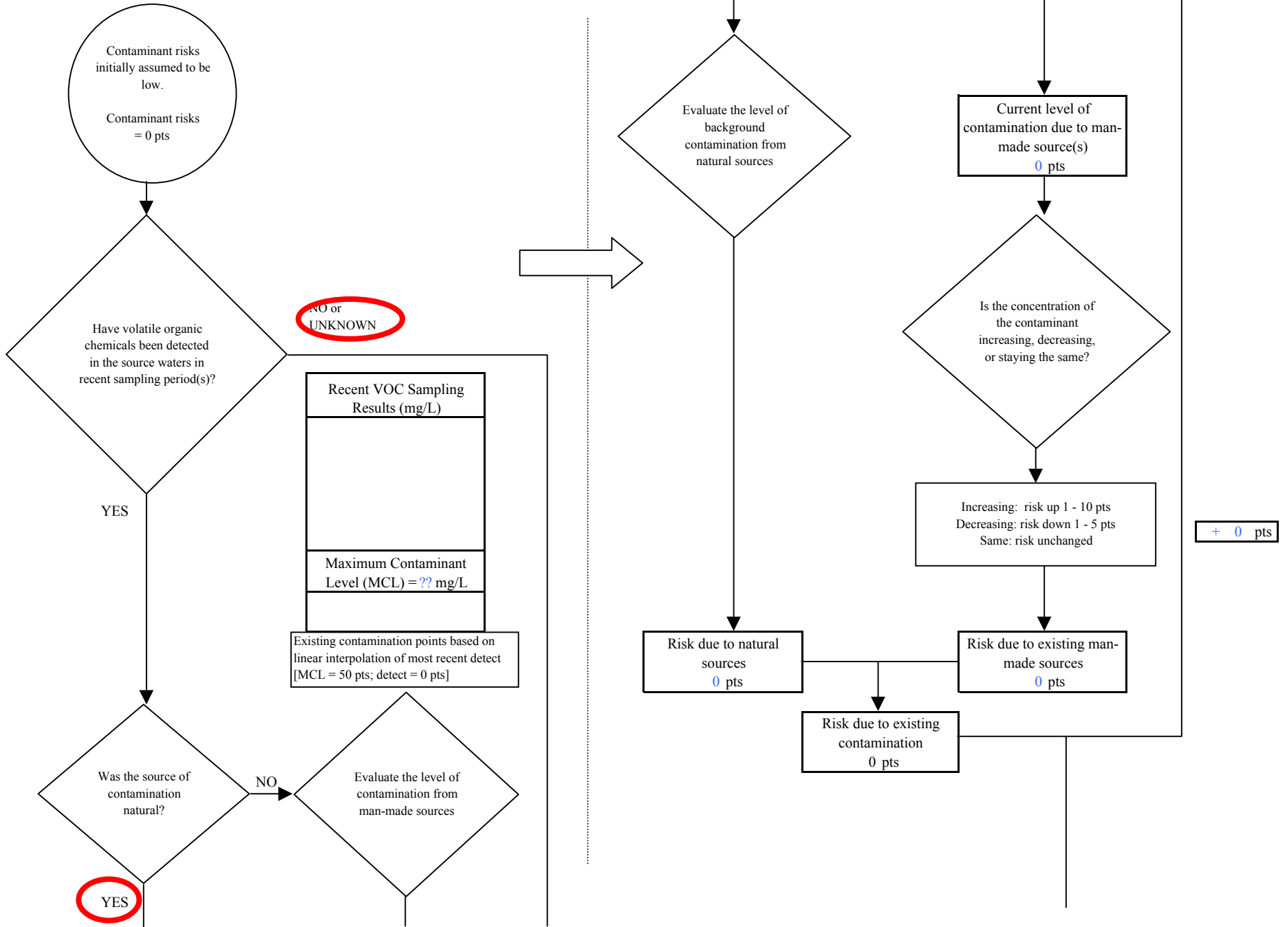
Chart 7. Contaminant risks for Valley Lanes - Volatile Organic Chemicals
