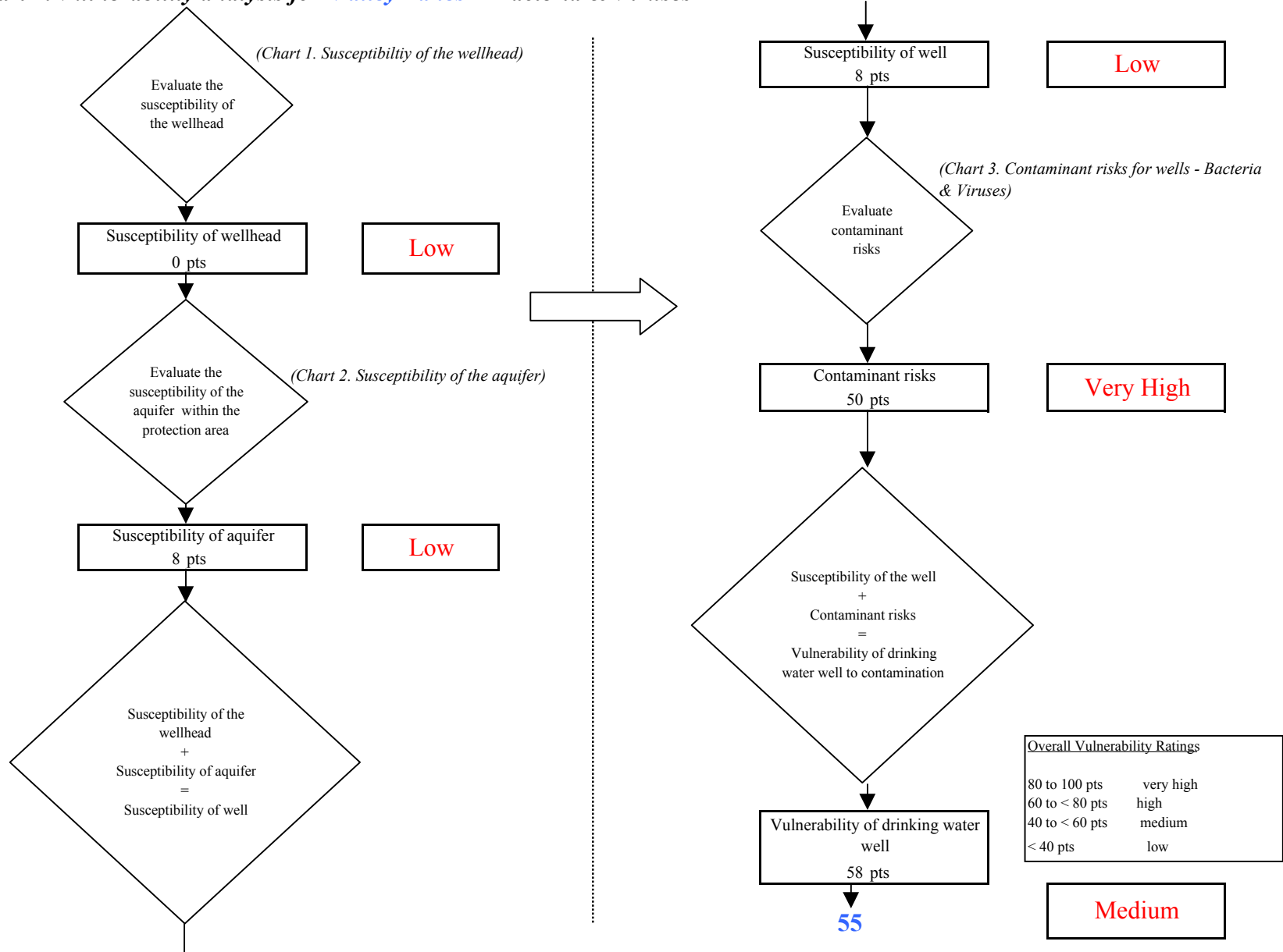
Chart 4. Vulnerability analysis for Valley Lanes - Bacteria & Viruses
