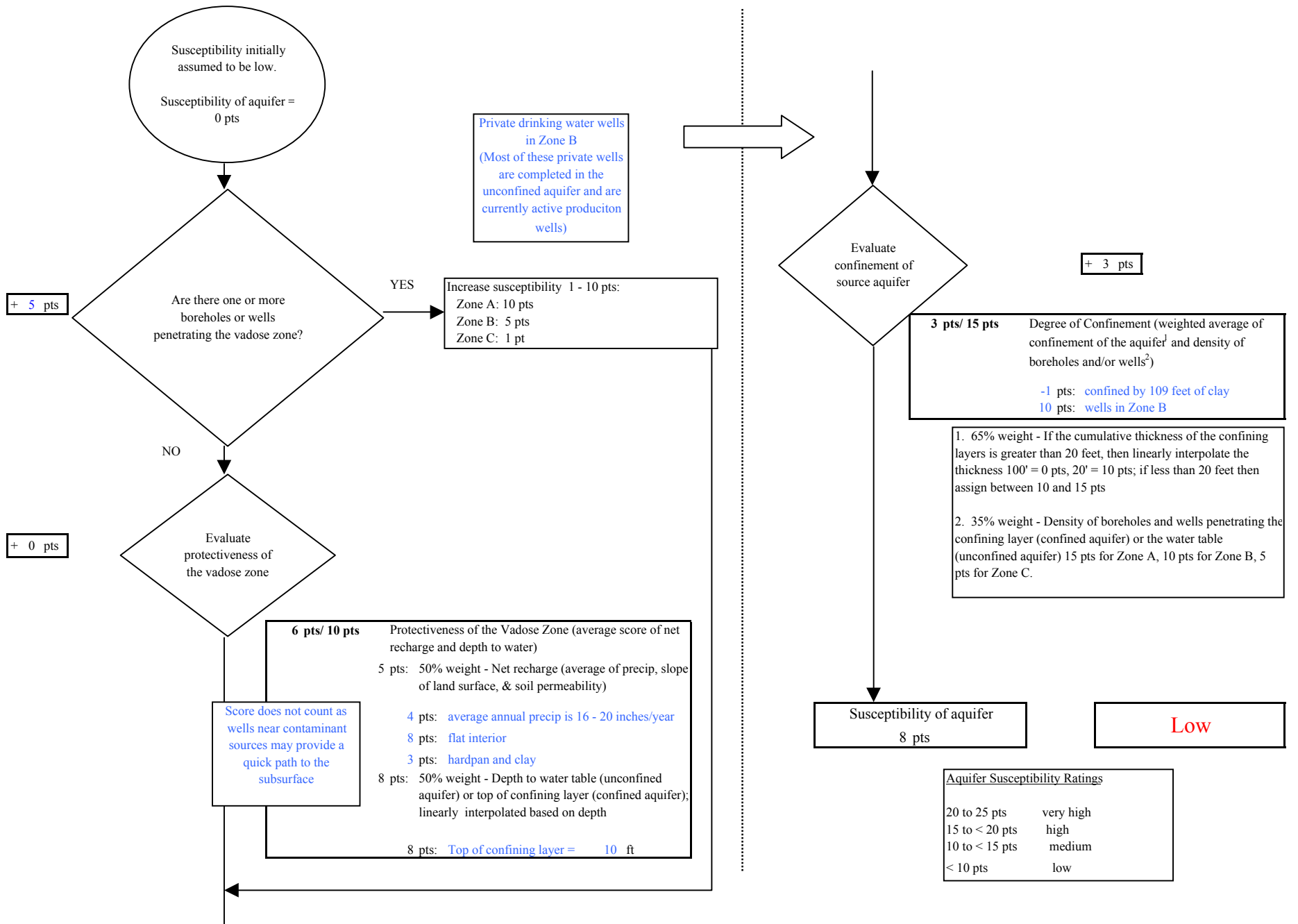
Chart 2. Susceptibility of the aquifer - Valley Lanes
