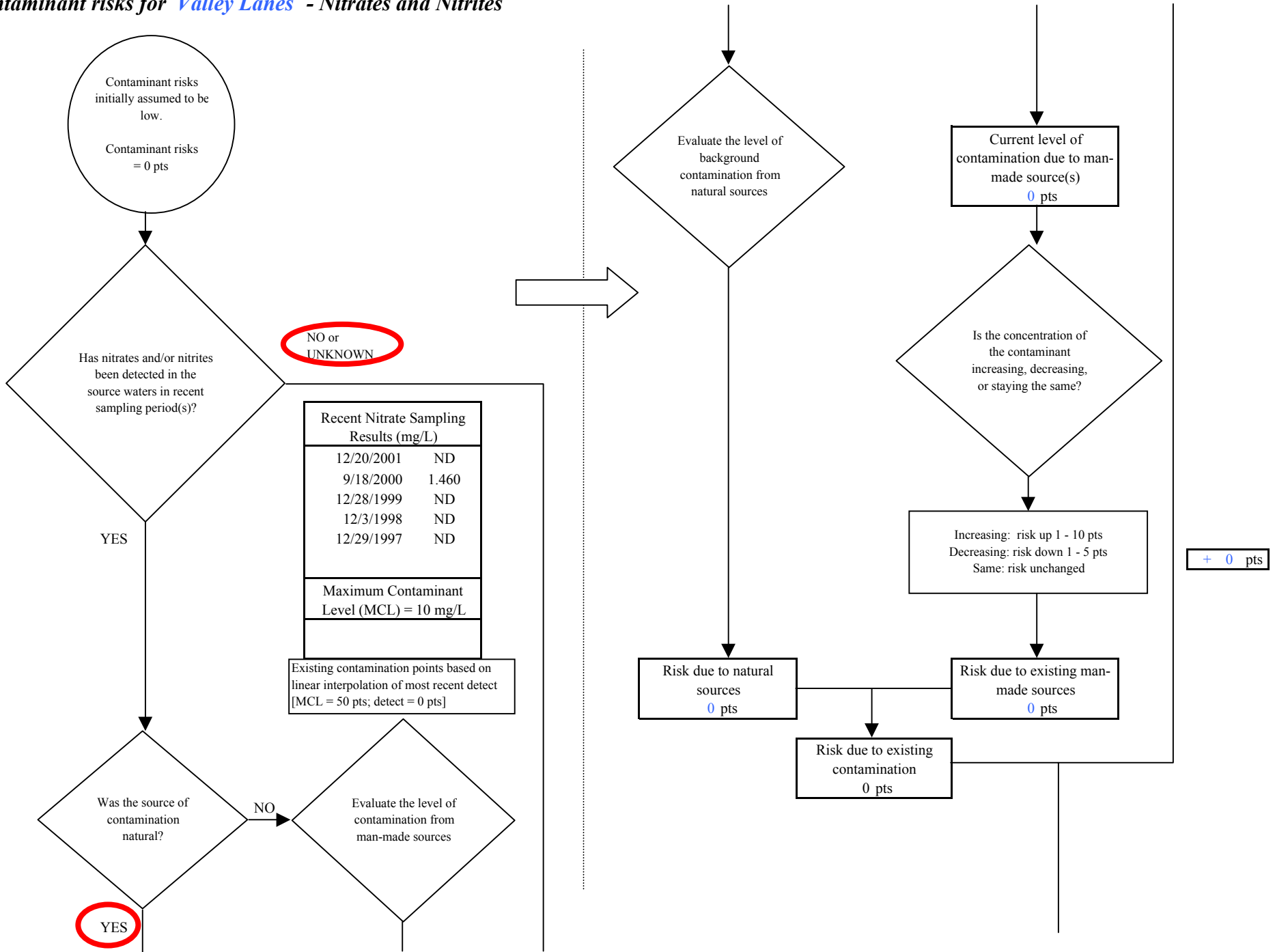
Chart 5. Contaminant risks for Valley Lanes - Nitrates and Nitrites
