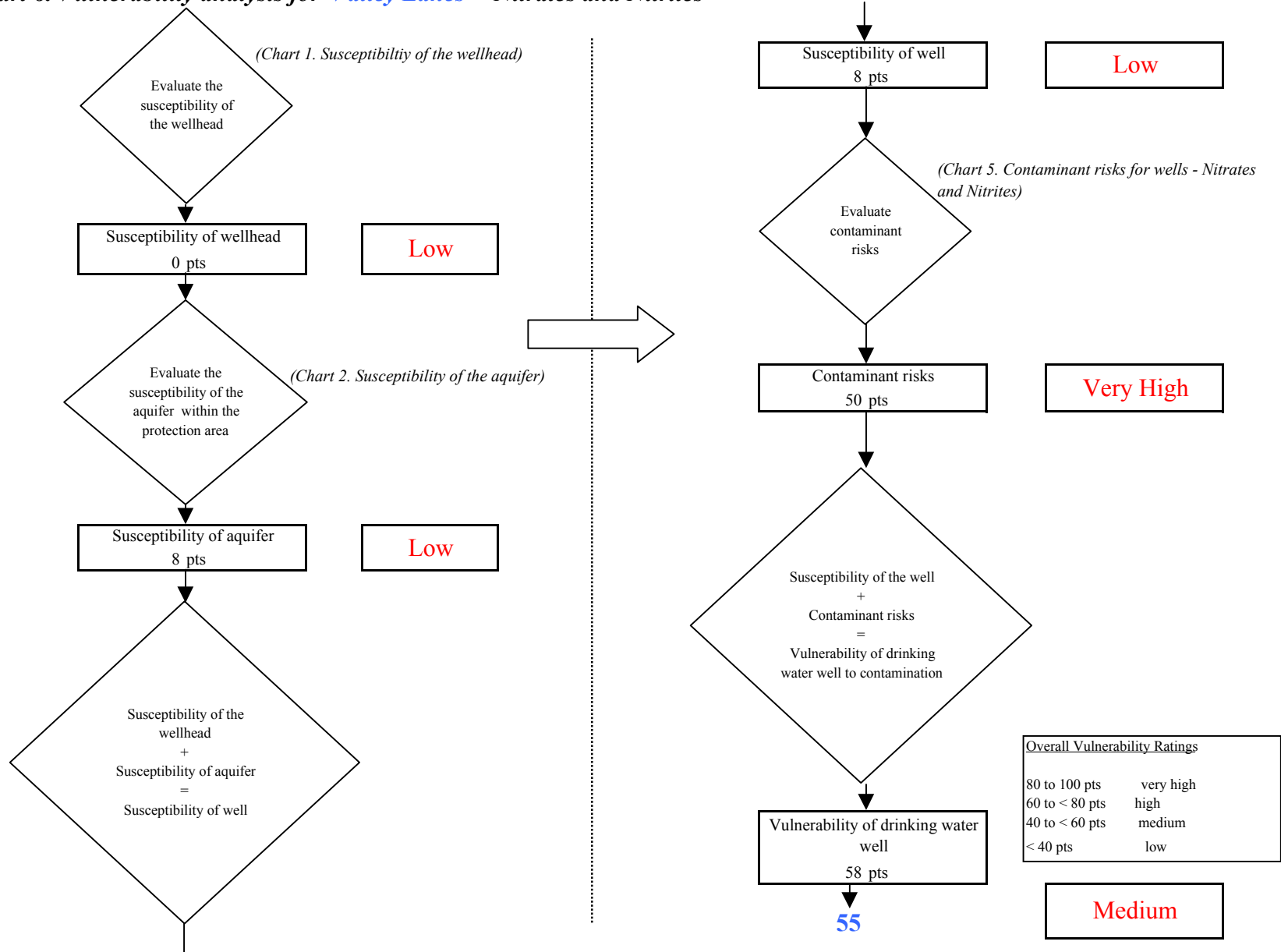
Chart 6. Vulnerability analysis for Valley Lanes - Nitrates and Nitrites
