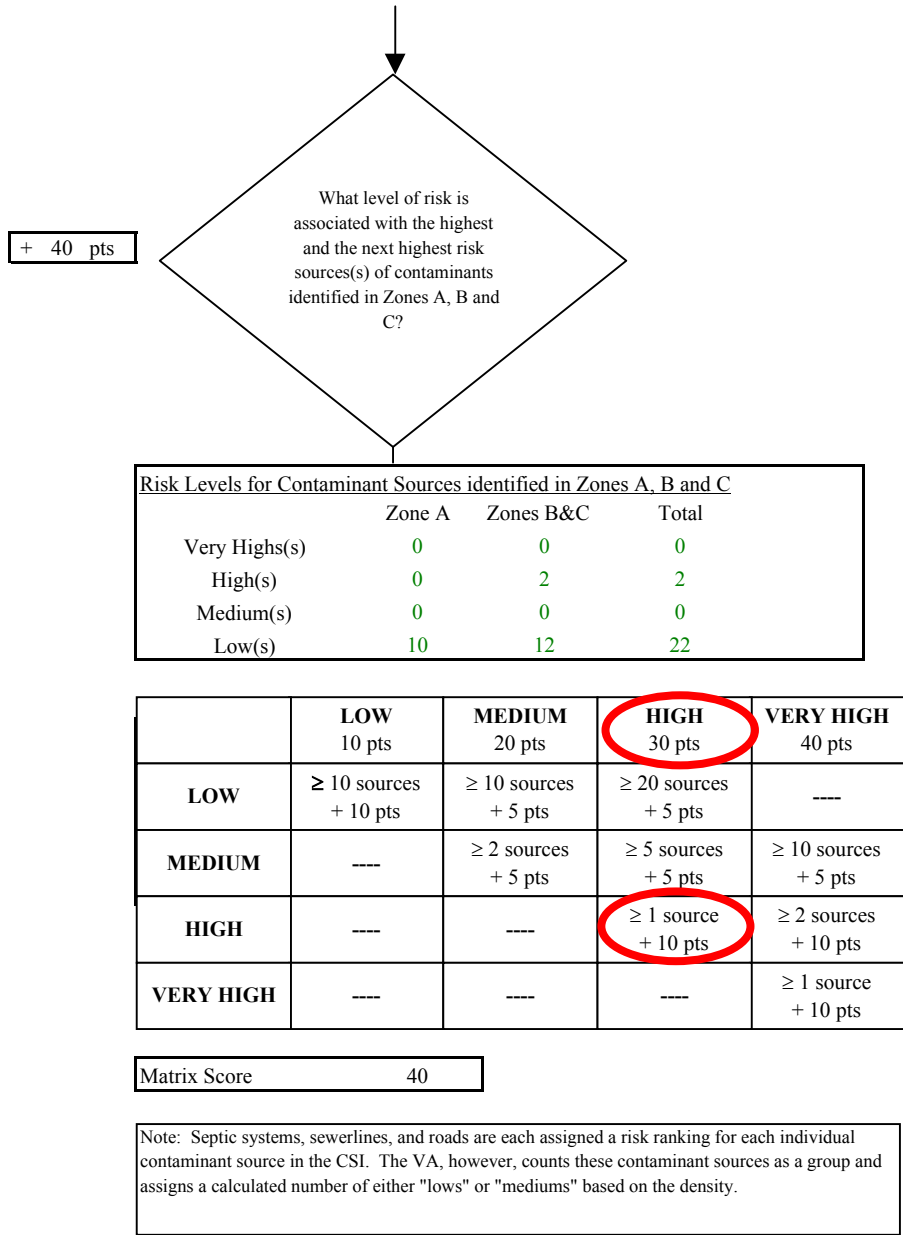
Chart 5. Contaminant risks for Sheena May Estates - Nitrates and Nitrites
