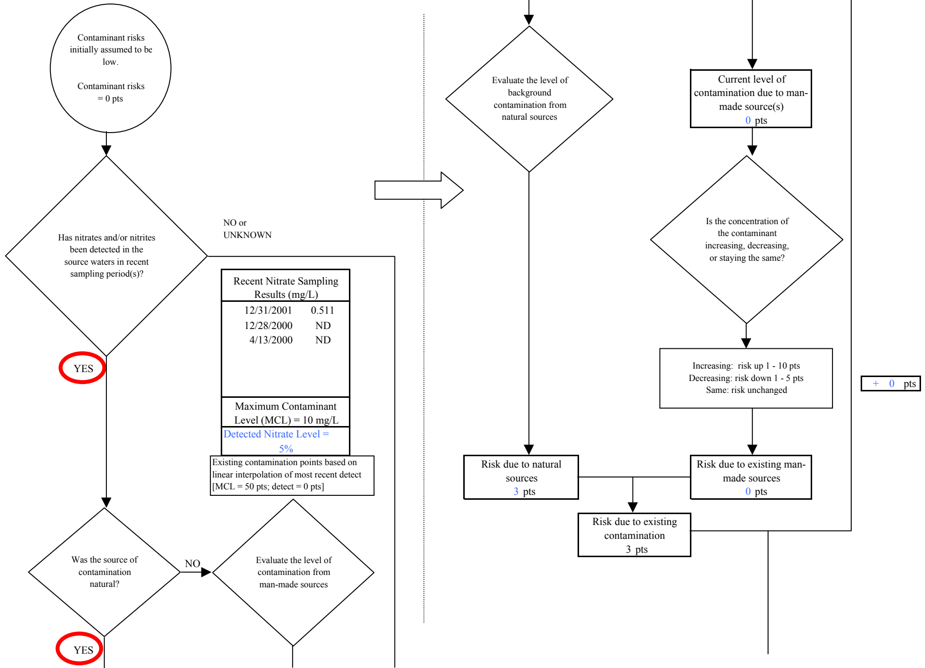
Chart 5. Contaminant risks for Sheena May Estates - Nitrates and Nitrites
