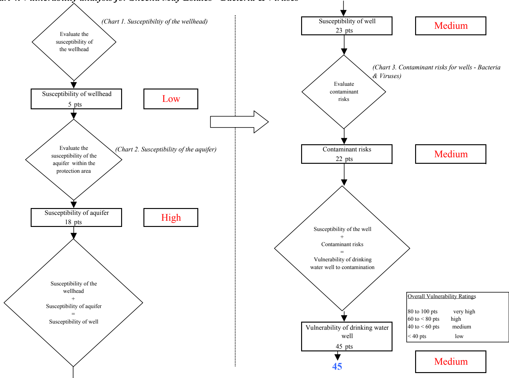
Chart 4. Vulnerability analysis for Sheena May Estates - Bacteria & Viruses
