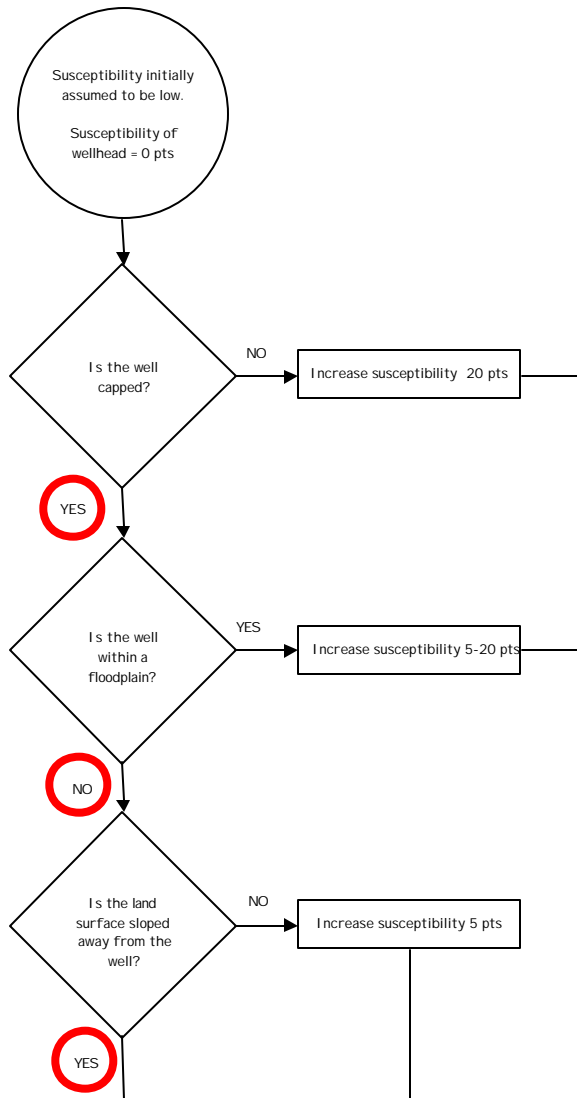
Chart 1. Susceptibility of the wellhead – Nye Ford Repair Shop
