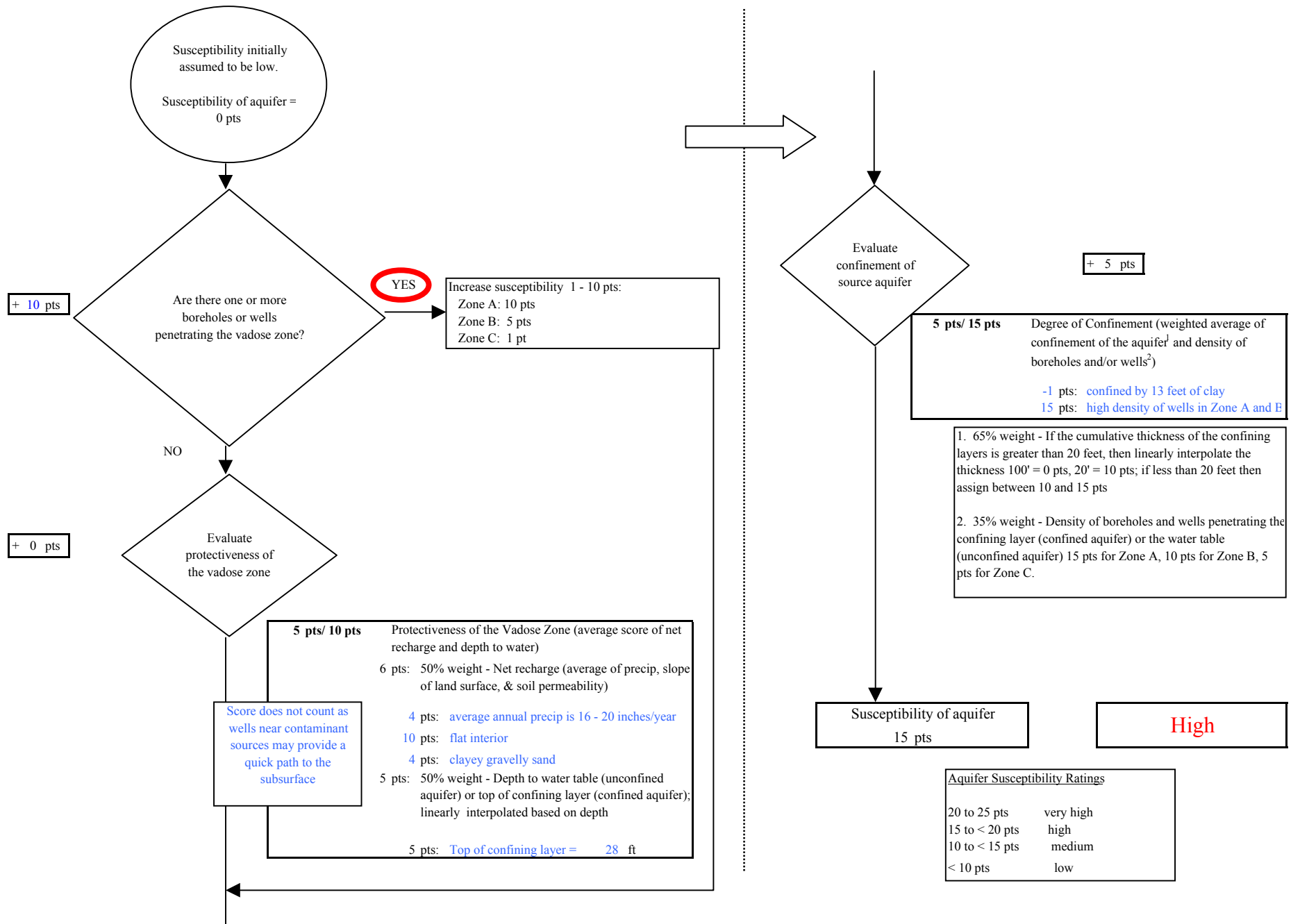
Chart 2. Susceptibility of the aquifer - Nugens Ranch
