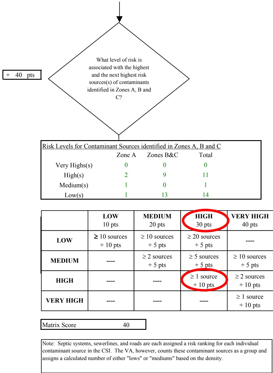
Chart 5. Contaminant risks for Nugens Ranch - Nitrates and Nitrites
