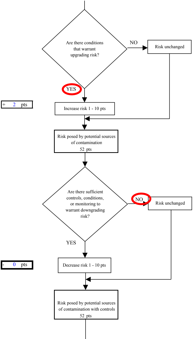
Chart 5. Contaminant risks for Nugens Ranch - Nitrates and Nitrites
