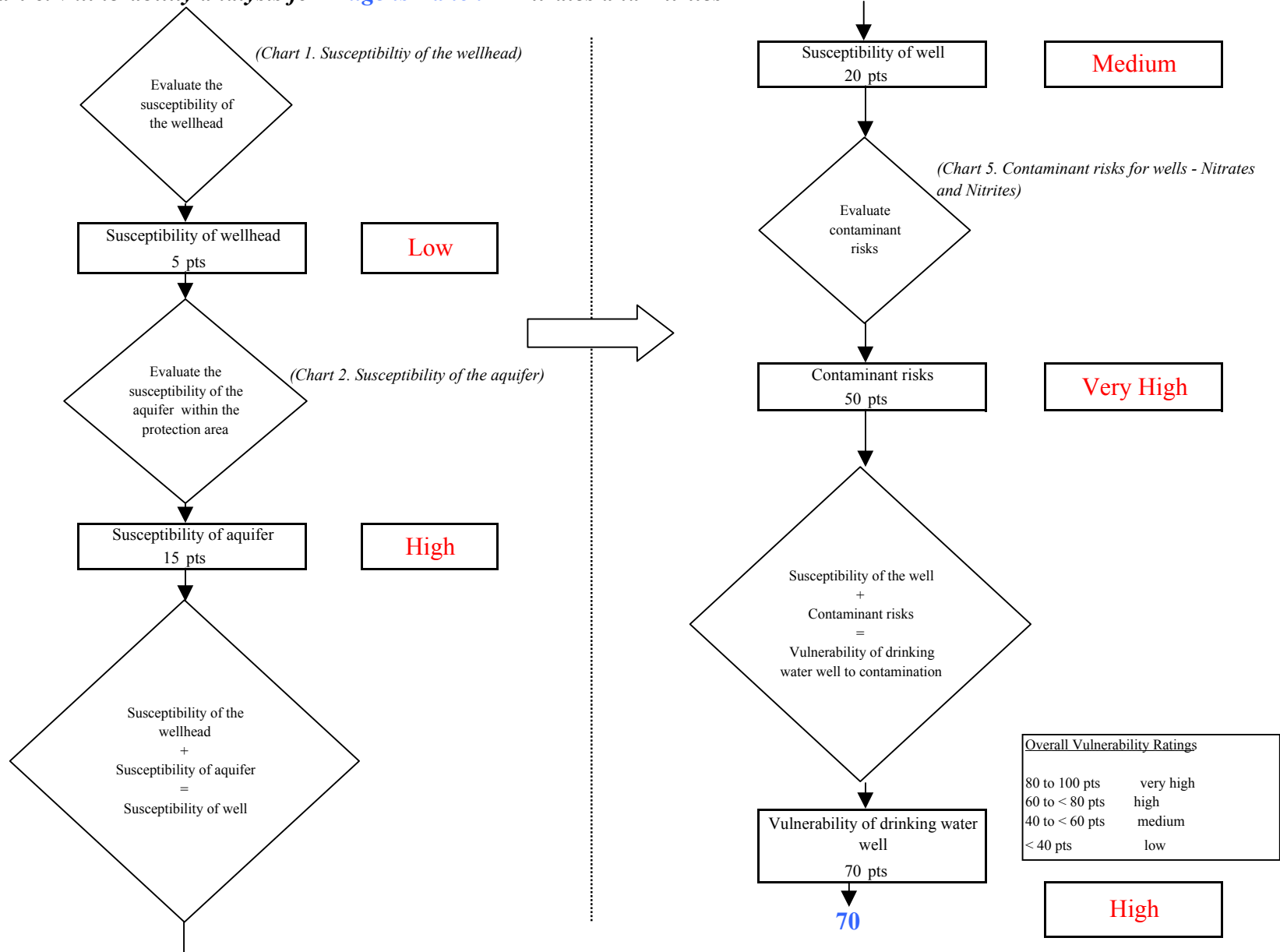
Chart 6. Vulnerability analysis for Nugens Ranch - Nitrates and Nitrites
