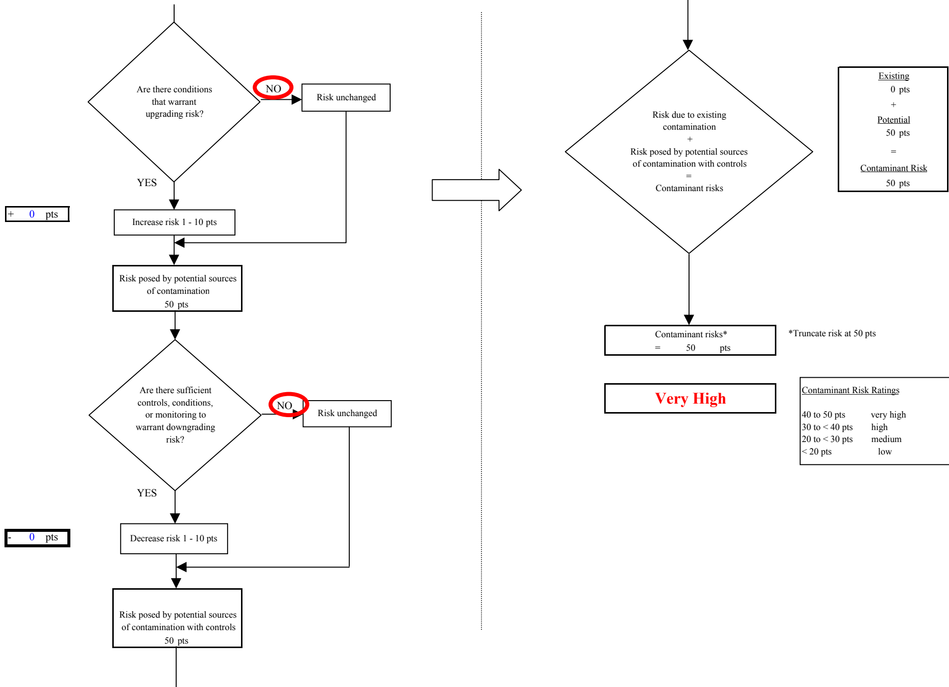
Chart 7. Contaminant risks for Nugens Ranch - Volatile Organic Chemicals
