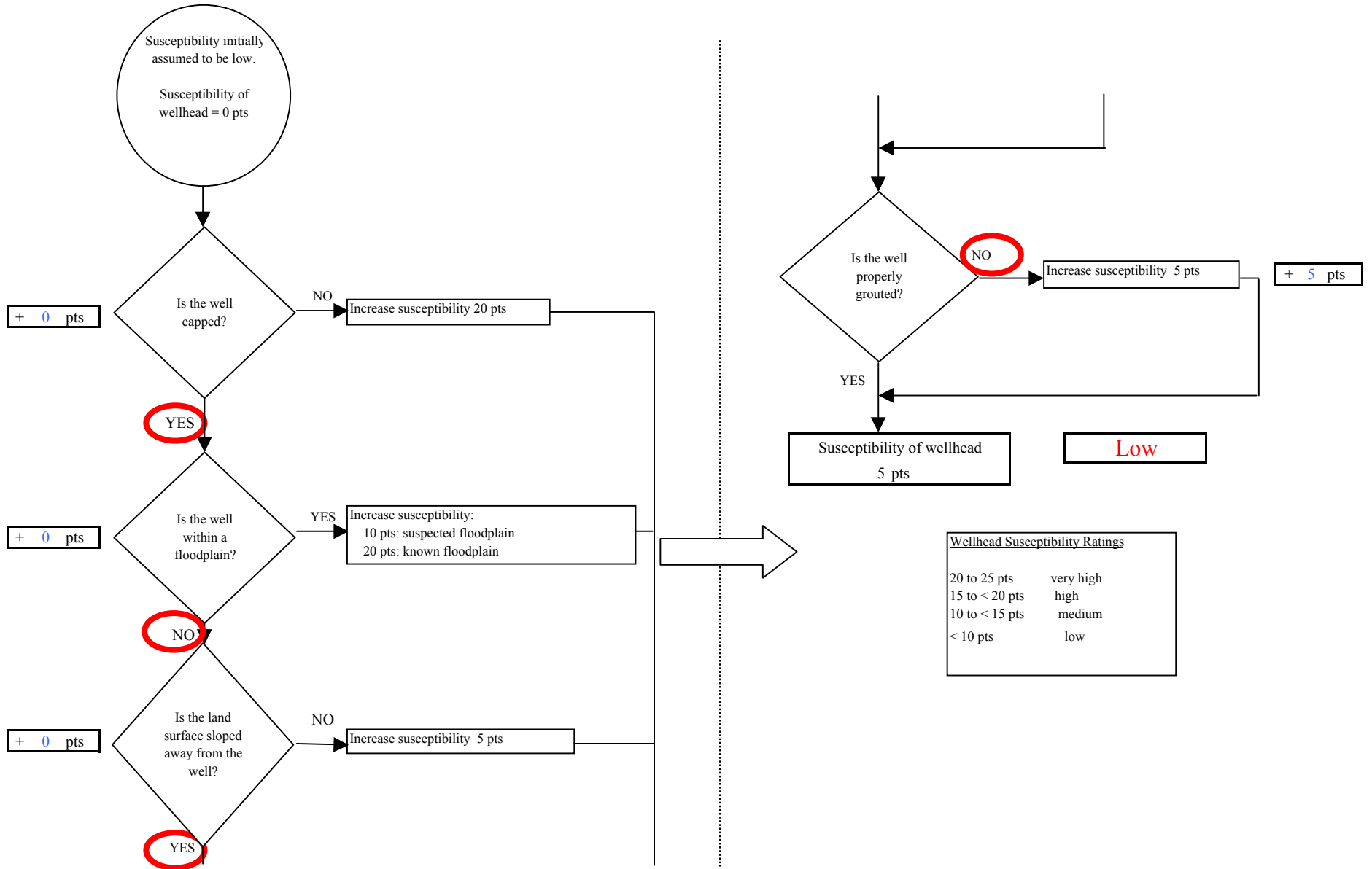
Chart 1. Susceptibility of the wellhead - Nugens Ranch
