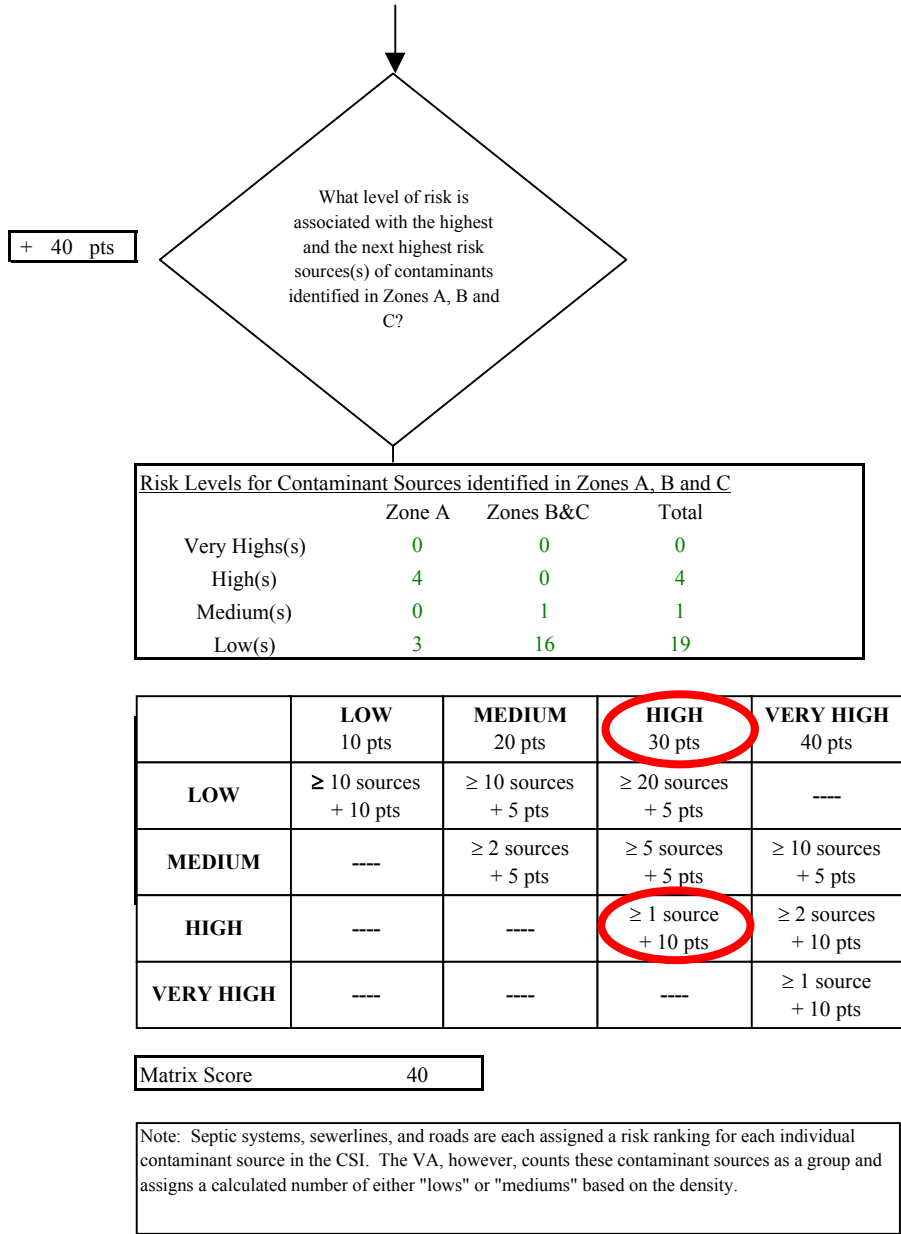
Chart 7. Contaminant risks for Nugens Ranch - Volatile Organic Chemicals
