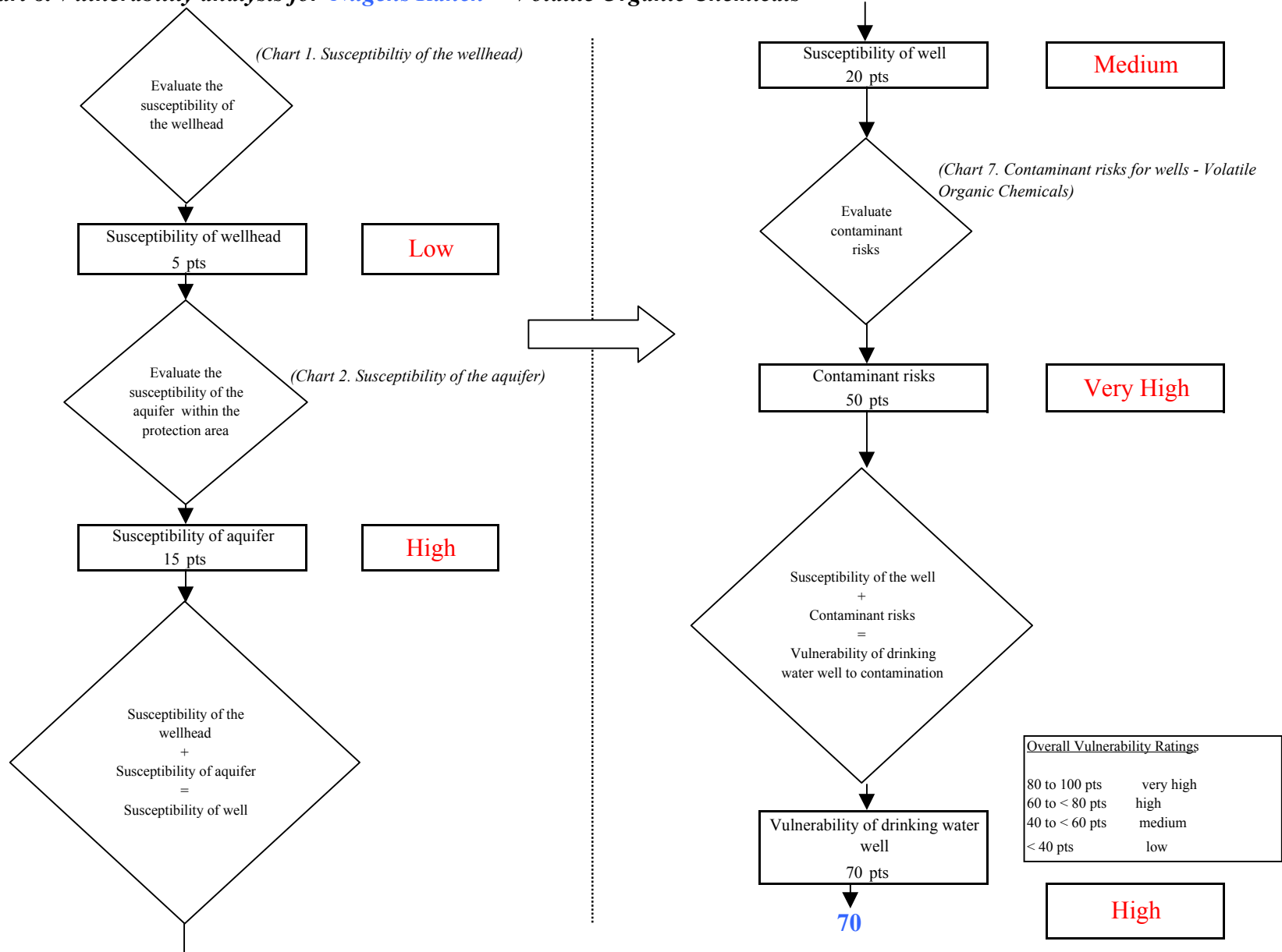
Chart 8. Vulnerability analysis for Nugens Ranch - Volatile Organic Chemicals
