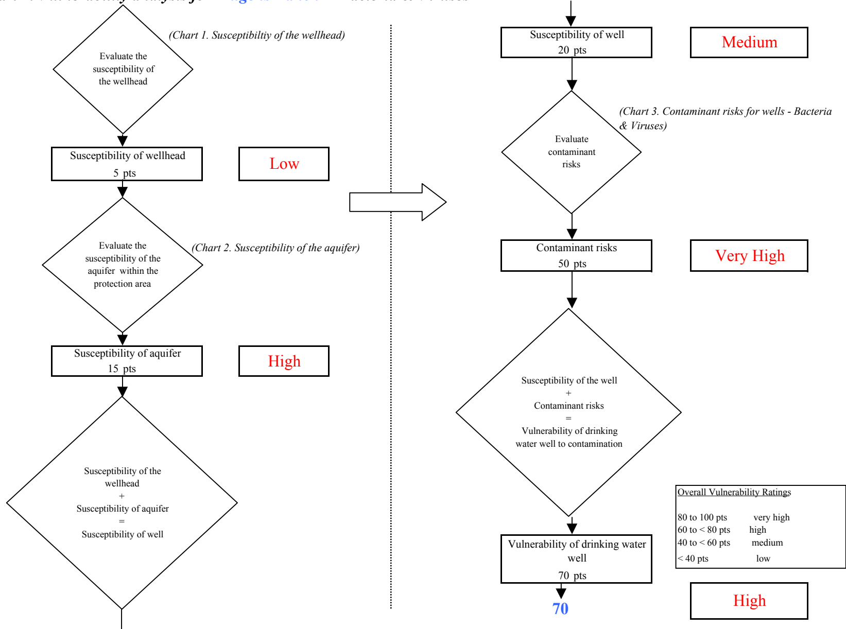
Chart 4. Vulnerability analysis for Nugens Ranch - Bacteria & Viruses
