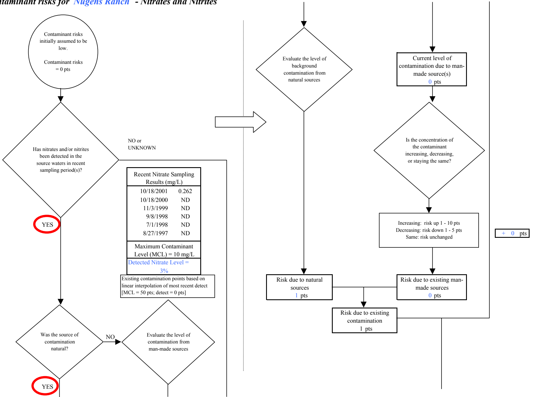
Chart 5. Contaminant risks for Nugens Ranch - Nitrates and Nitrites
