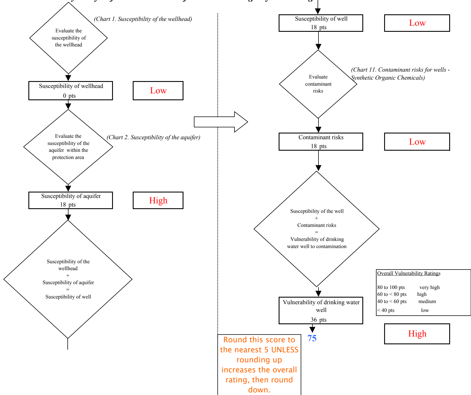
Chart 12. Vulnerability analysis for North Fork Professional Building - Synthetic Organic Chemicals
