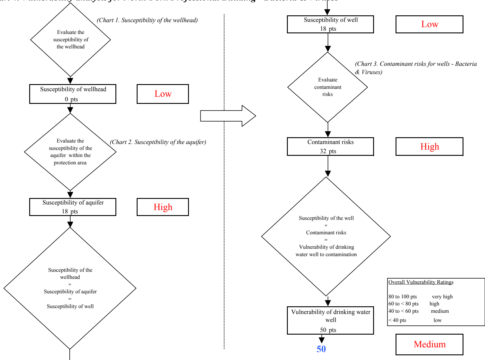
Chart 4. Vulnerability analysis for North Fork Professional Building - Bacteria & Viruses
