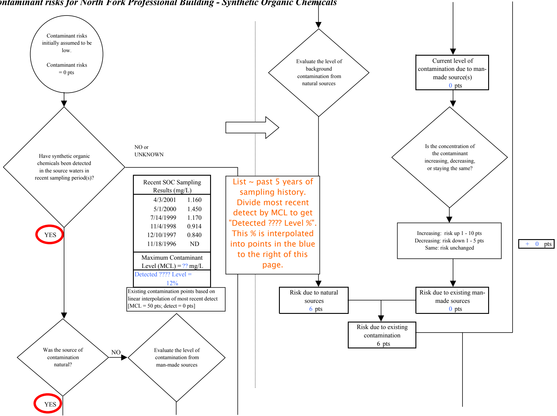
Chart 11. Contaminant risks for North Fork Professional Building - Synthetic Organic Chemicals
