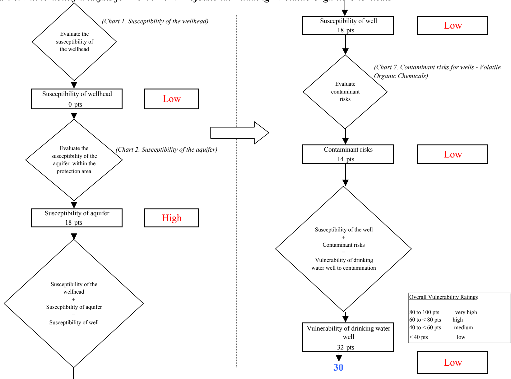
Chart 8. Vulnerability analysis for North Fork Professional Building - Volatile Organic Chemicals
