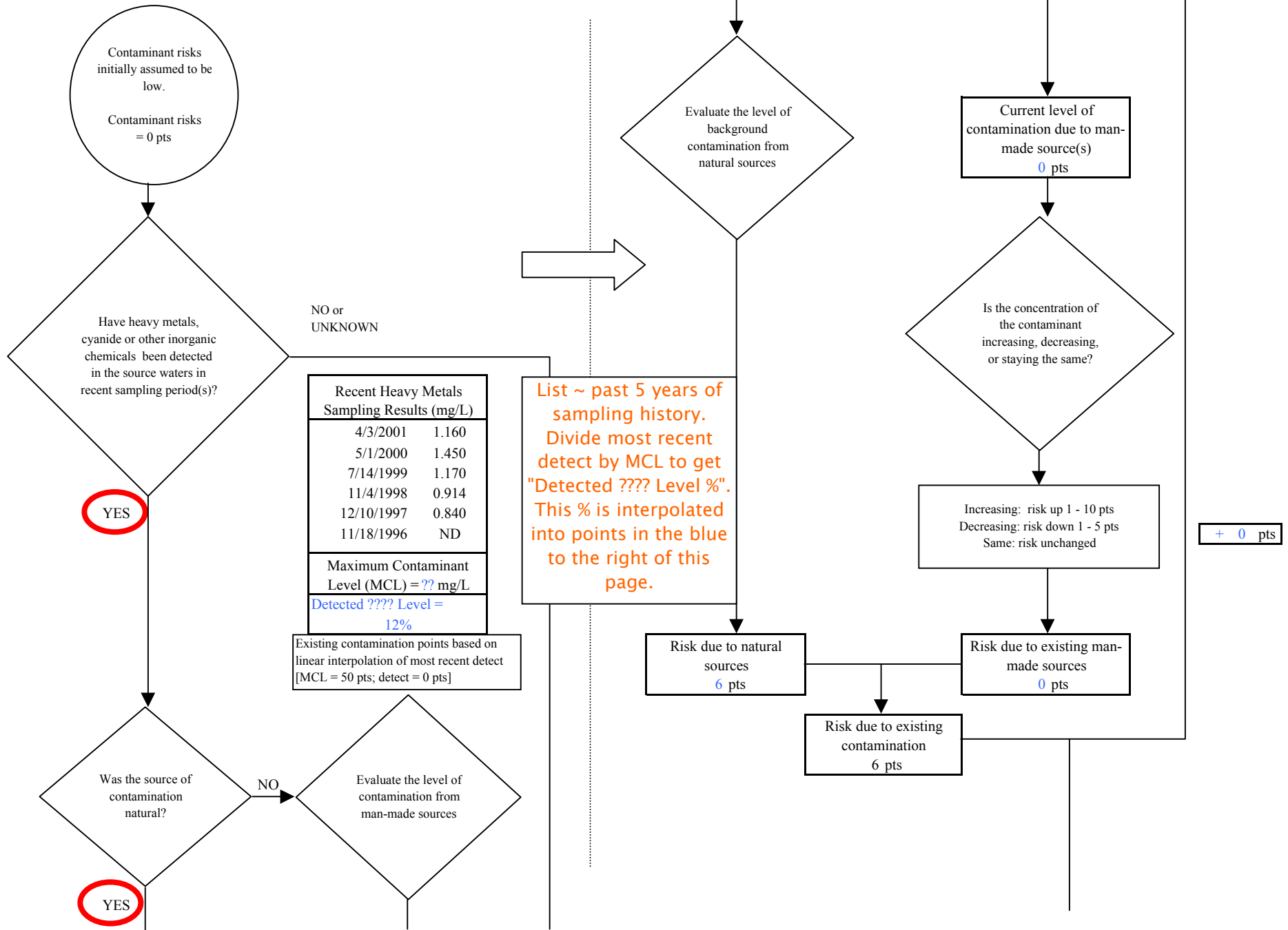
Chart 9. Contaminant risks for North Fork Professional Building - Heavy Metals, Cyanide and Other Inorganic Chemicals
