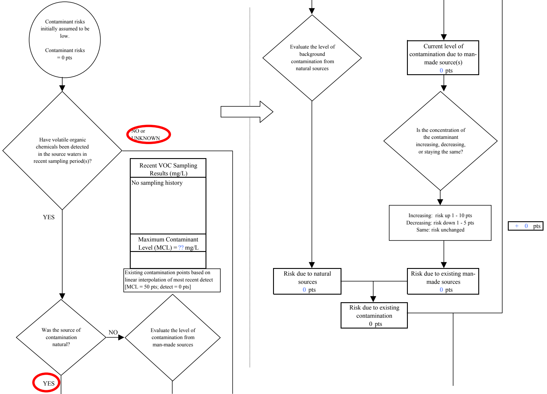
Chart 7. Contaminant risks for North Fork Professional Building - Volatile Organic Chemicals
