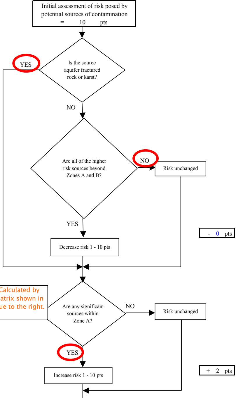
Chart 9. Contaminant risks for North Fork Professional Building - Heavy Metals, Cyanide and Other Inorganic Chemicals
