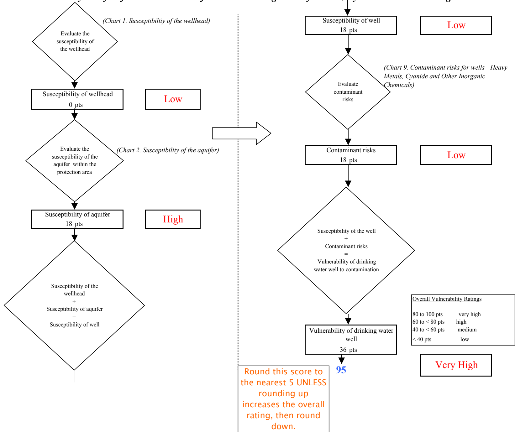
Chart 10. Vulnerability analysis for North Fork Professional Building - Heavy Metals, Cyanide and Other Inorganic Chemicals
