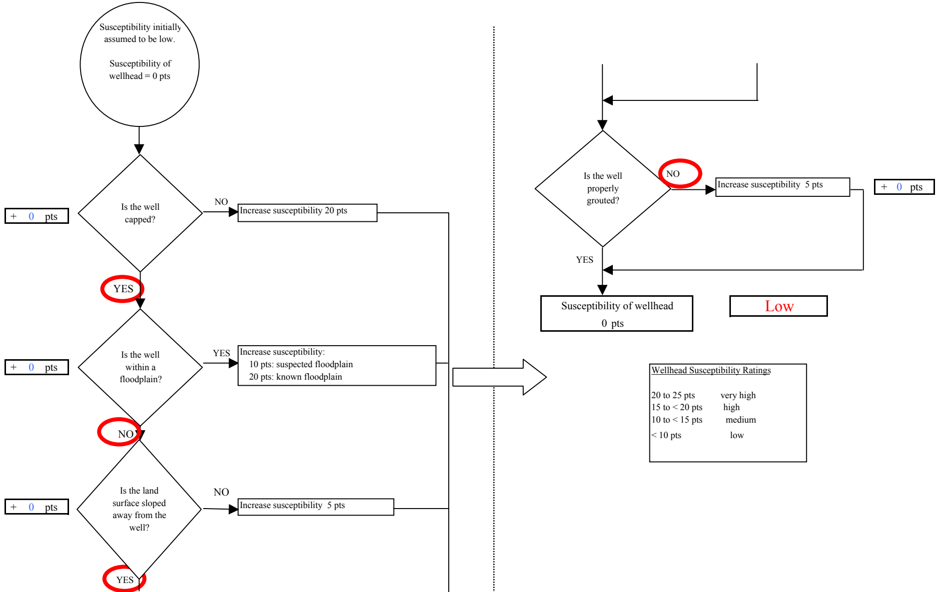
Chart 1. Susceptibility of the wellhead - North Fork Professional Building
