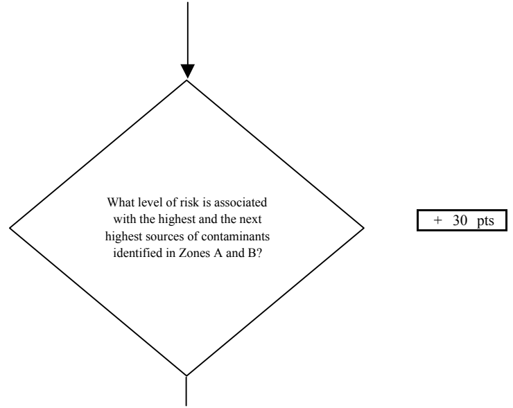
Chart 3. Contaminant risks for North Fork Professional Building - Bacteria & Viruses
