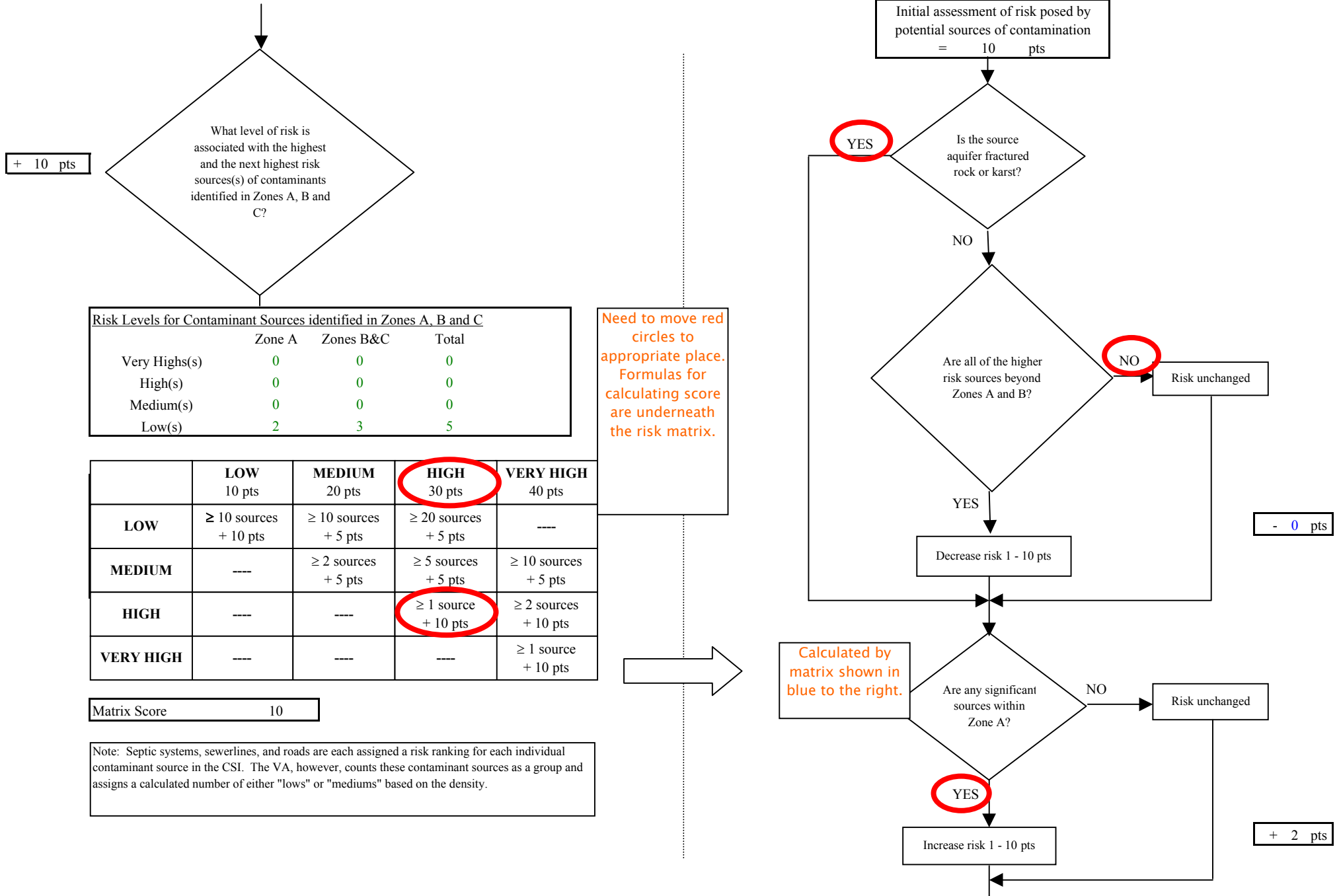
Chart 11. Contaminant risks for North Fork Professional Building - Synthetic Organic Chemicals
