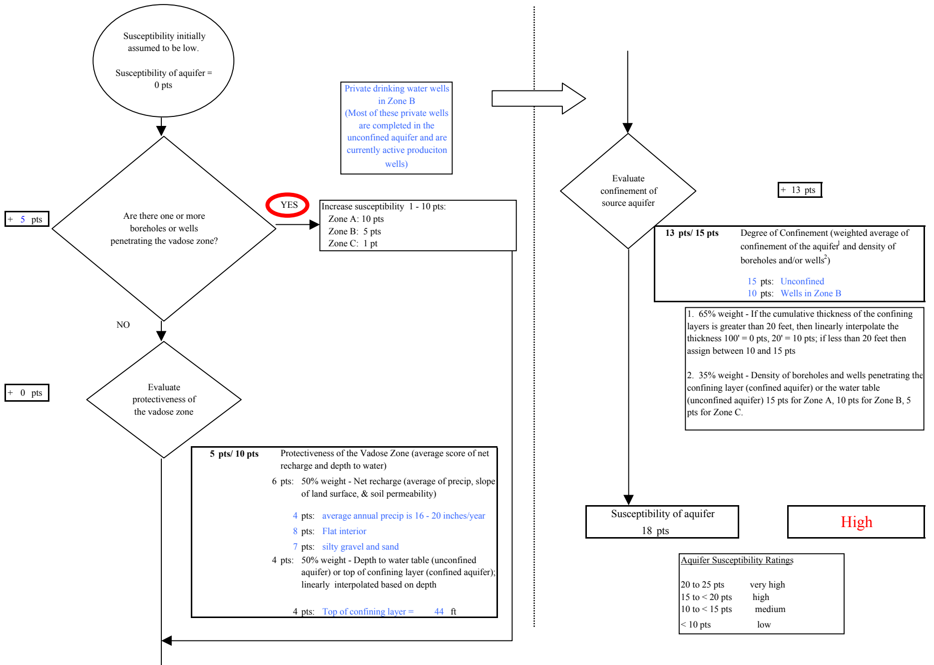
Chart 2. Susceptibility of the aquifer - North Fork Professional Building
