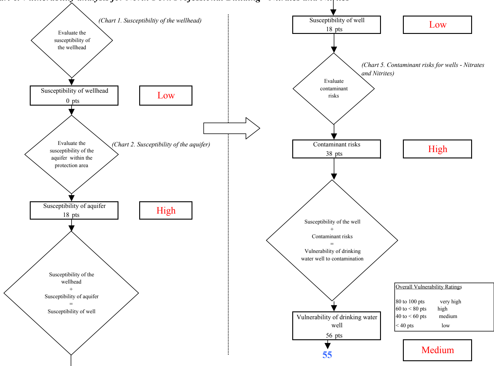
Chart 6. Vulnerability analysis for North Fork Professional Building - Nitrates and Nitrites
