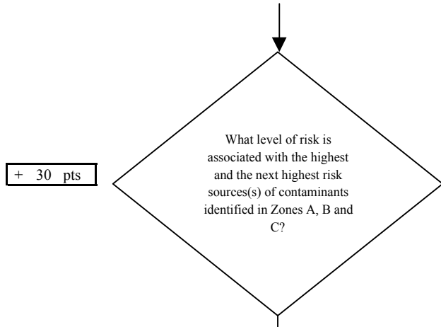
Chart 5. Contaminant risks for North Fork Professional Building - Nitrates and Nitrites
