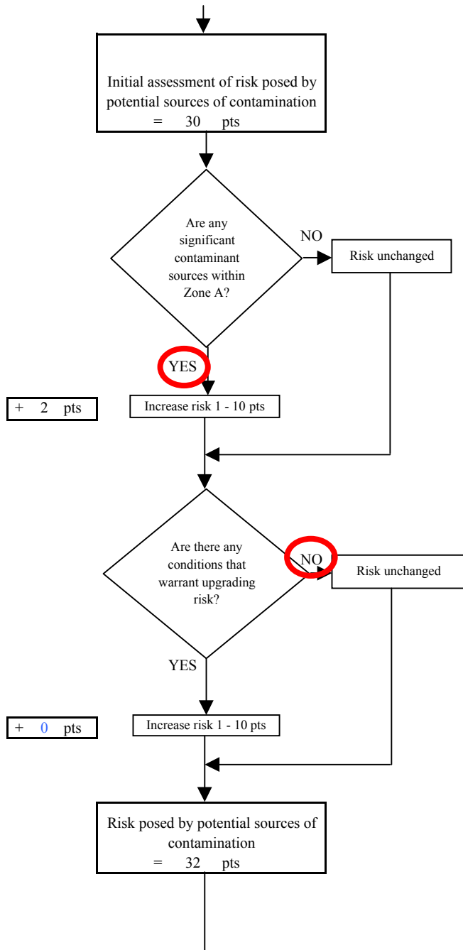
Chart 3. Contaminant risks for North Fork Professional Building - Bacteria & Viruses
