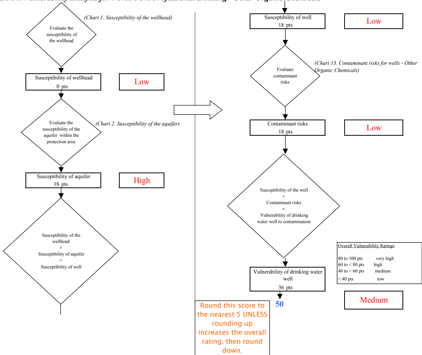
Chart 14. Vulnerability analysis for North Fork Professional Building - Other Organic Chemicals
