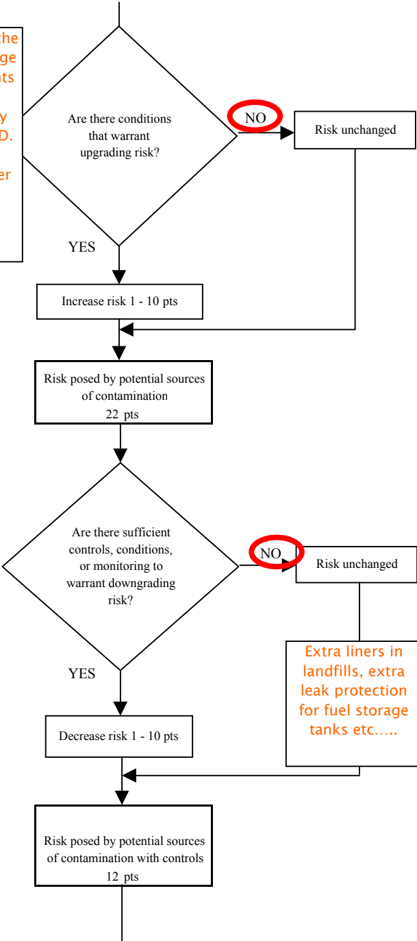
Chart 11. Contaminant risks for North Fork Professional Building - Synthetic Organic Chemicals
