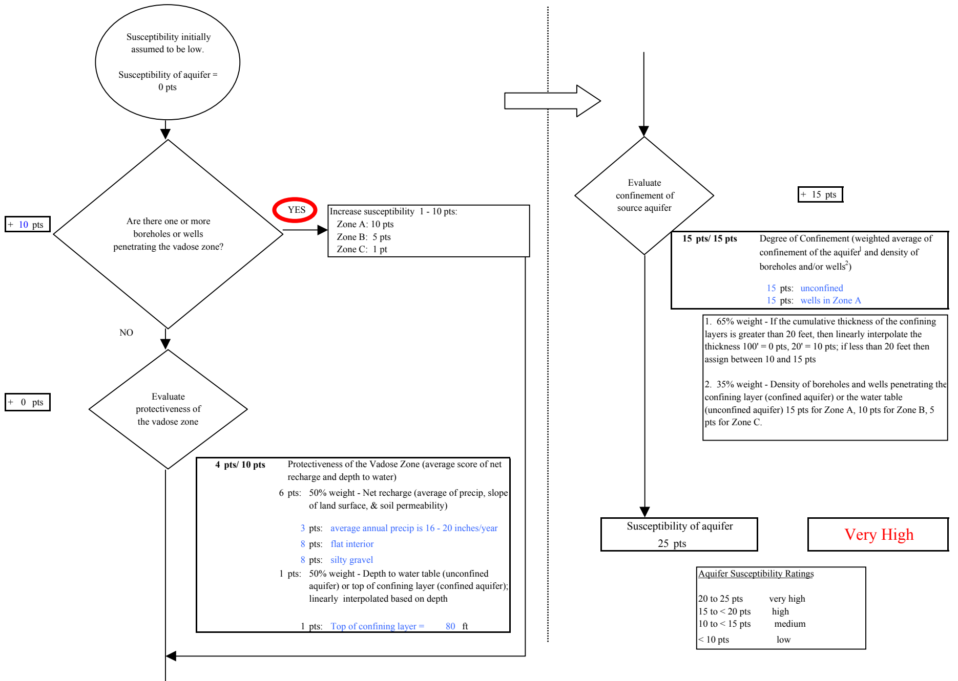
Chart 2. Susceptibility of the aquifer - Wasilla First United Methodist Church
