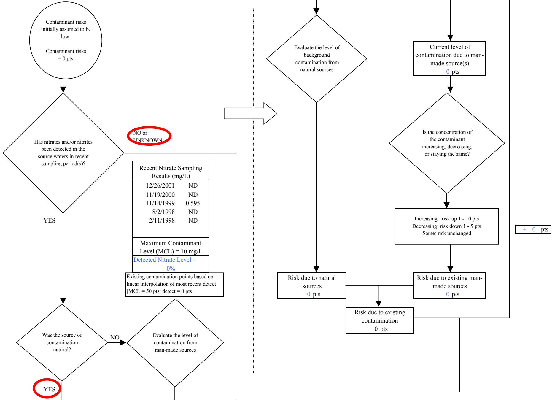
Chart 5. Contaminant risks for Wasilla First United Methodist Church - Nitrates and Nitrites
