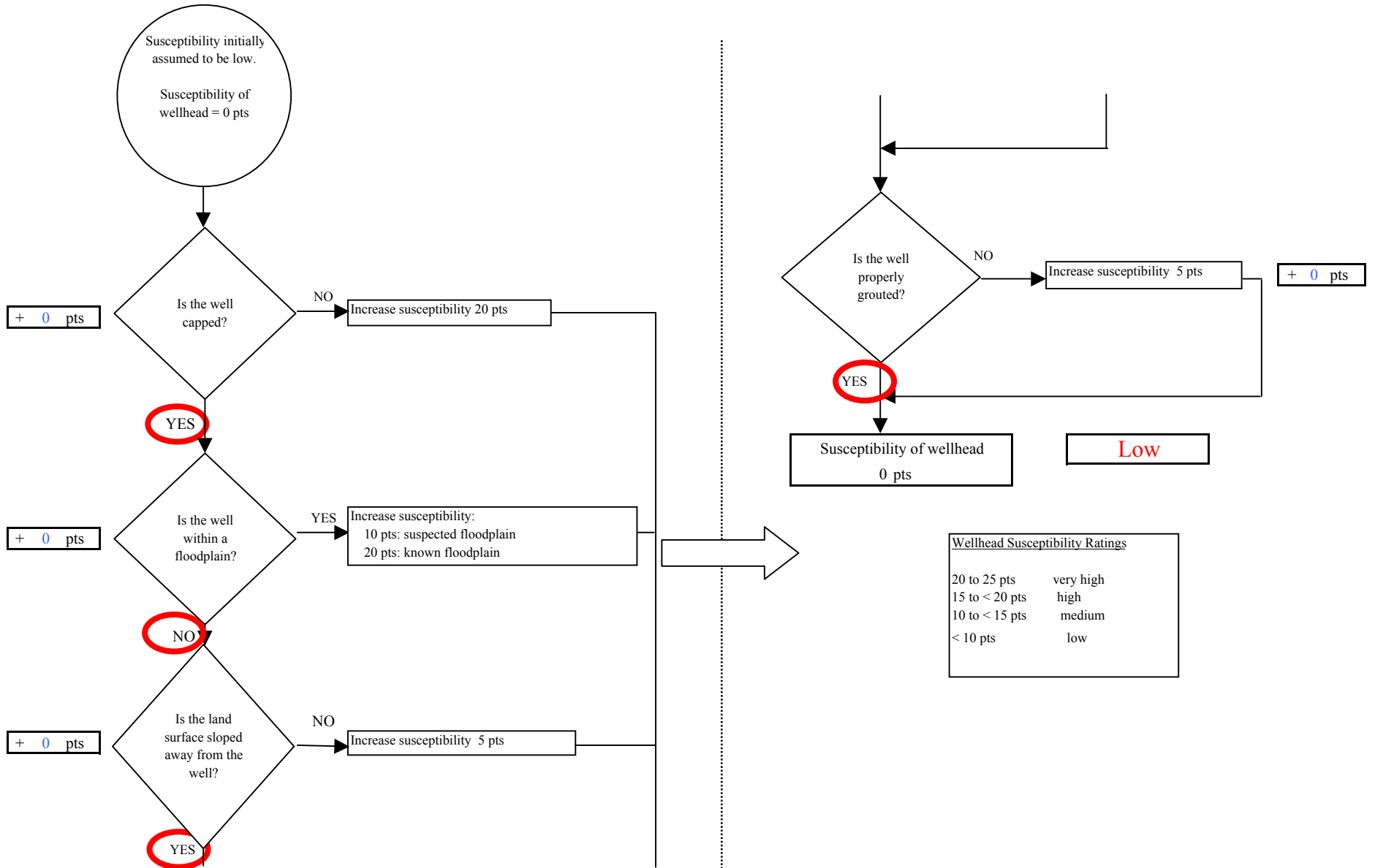
Chart 1. Susceptibility of the wellhead - Wasilla First United Methodist Church
