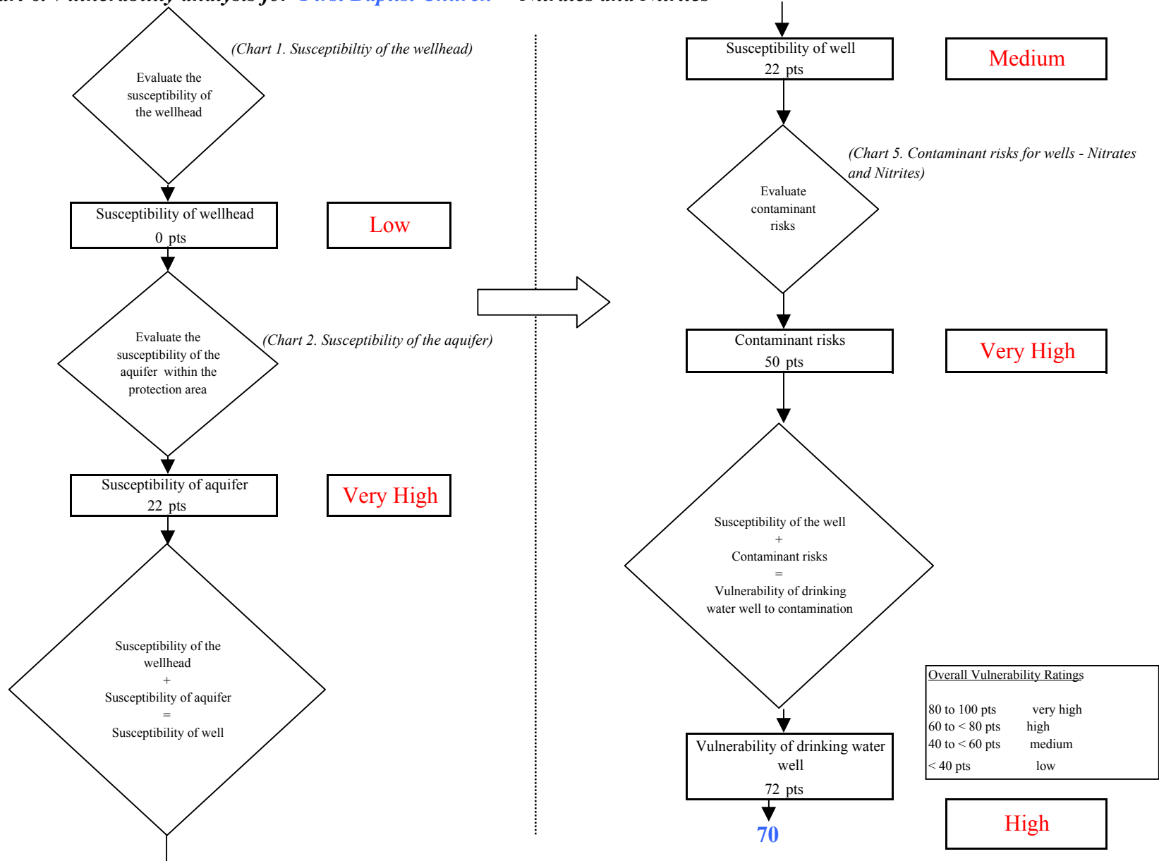
Chart 6. Vulnerability analysis for First Baptist Church - Nitrates and Nitrites
