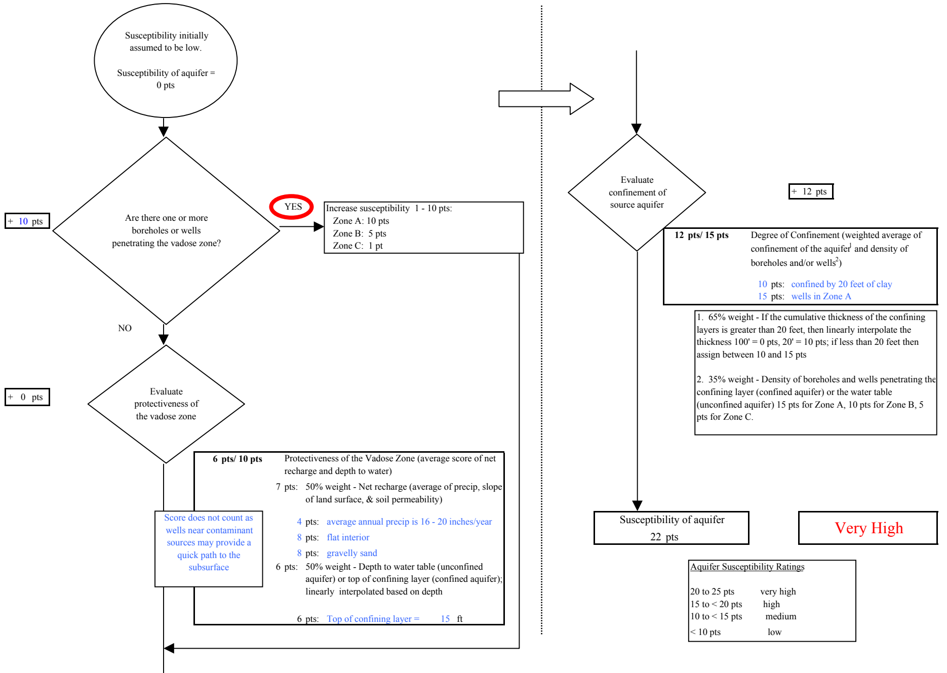
Chart 2. Susceptibility of the aquifer - First Baptist Church
