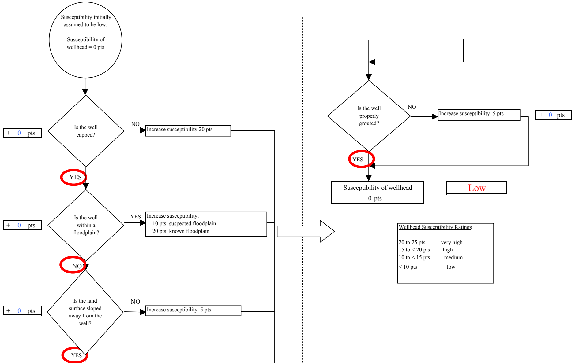
Chart 1. Susceptibility of the wellhead - First Baptist Church
