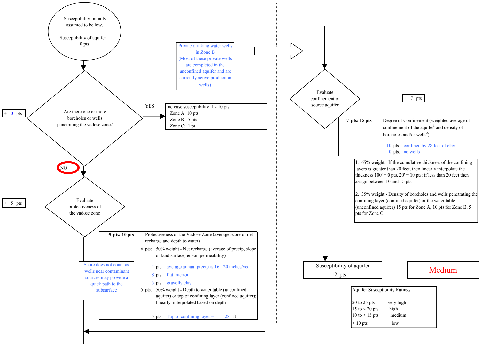
Chart 2. Susceptibility of the aquifer - Camp Togowoods
