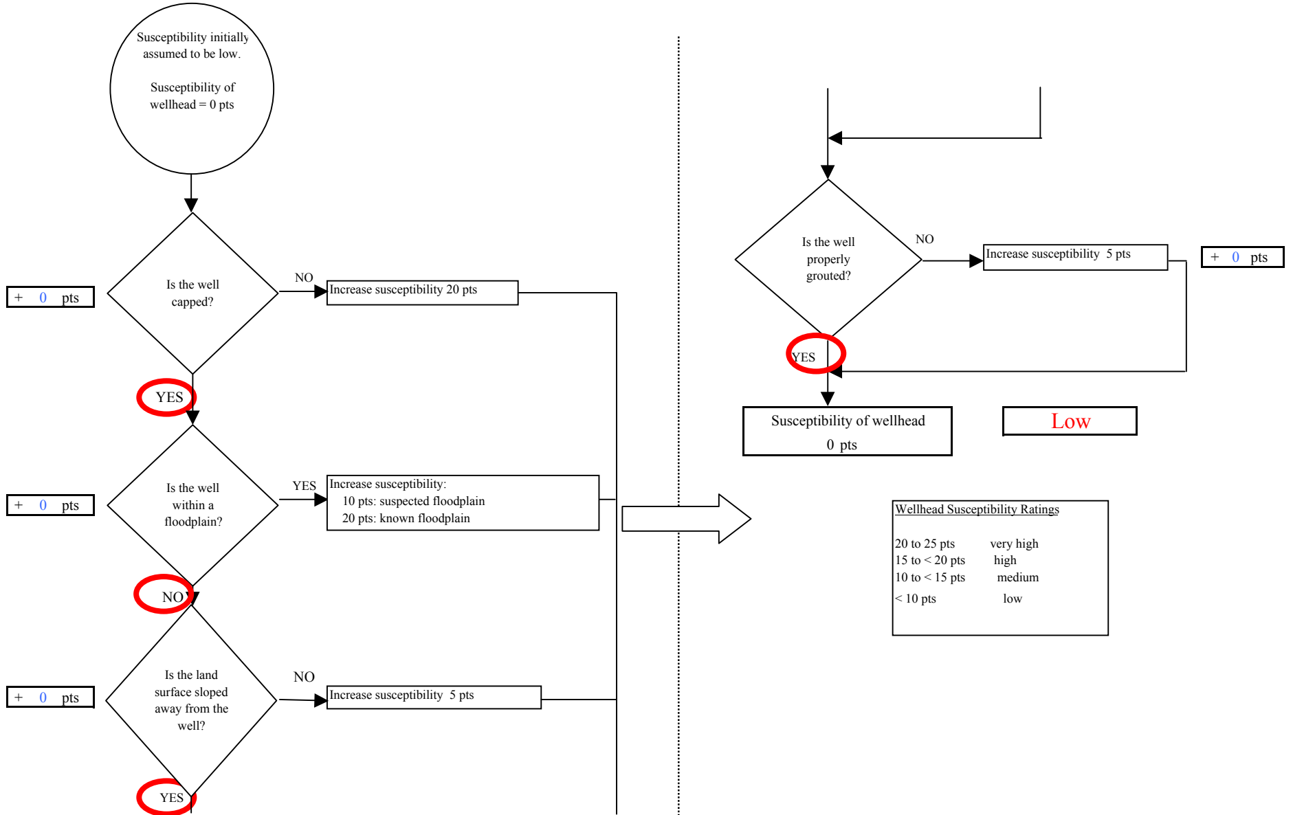
Chart 1. Susceptibility of the wellhead - Alcantra National Guard
