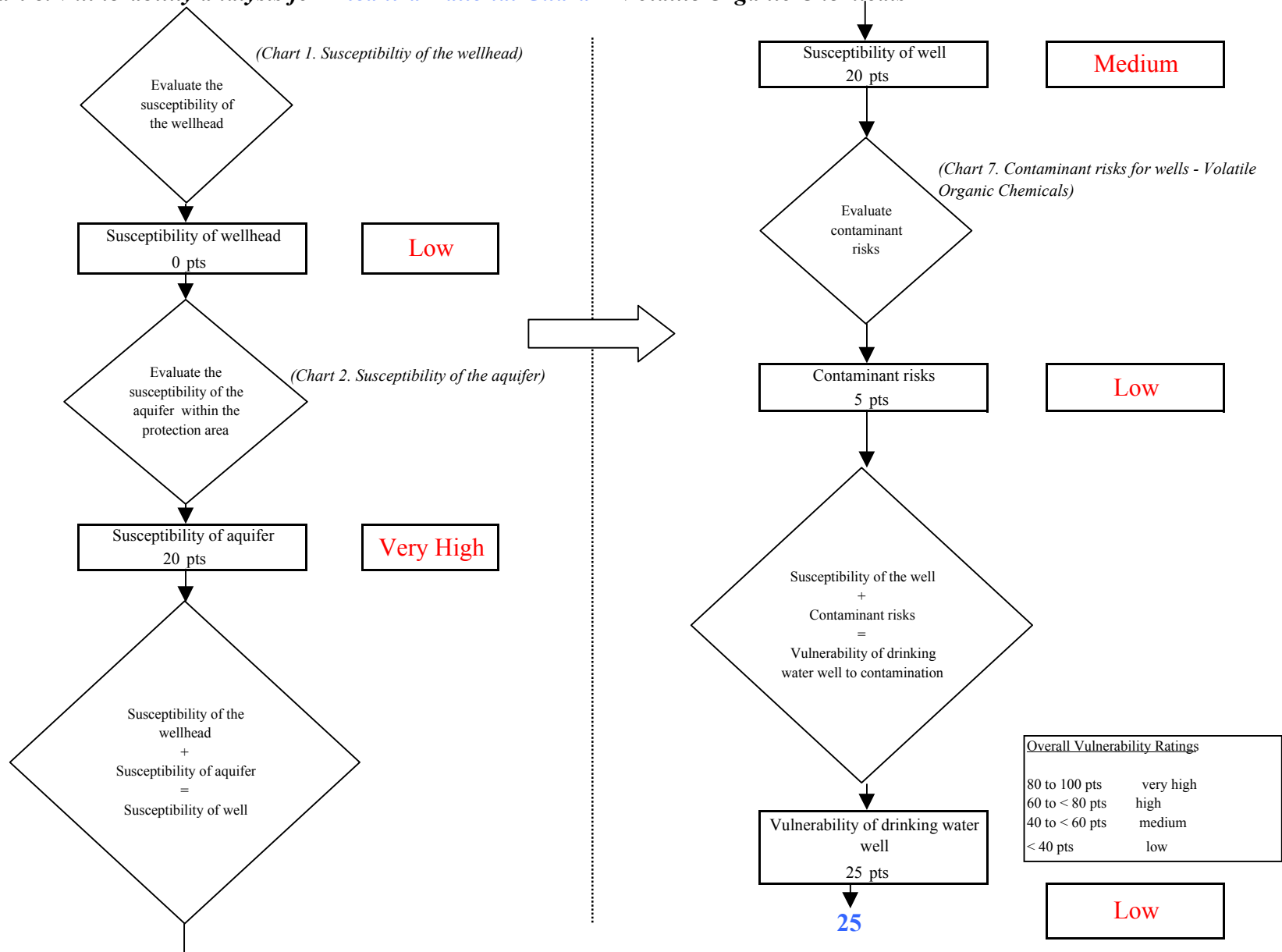
Chart 8. Vulnerability analysis for Alcantra National Guard - Volatile Organic Chemicals
