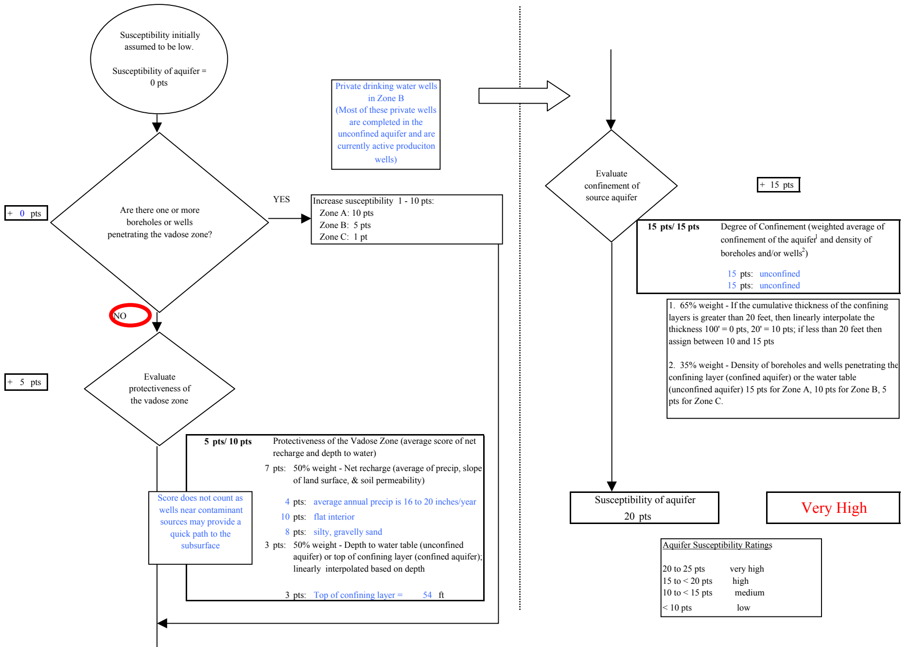
Chart 2. Susceptibility of the aquifer - Alcantra National Guard
