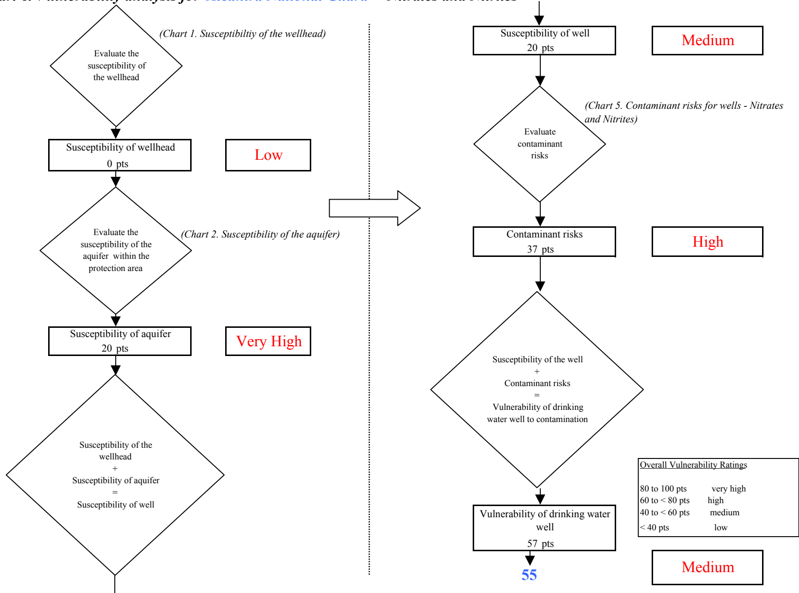
Chart 6. Vulnerability analysis for Alcantra National Guard - Nitrates and Nitrites
