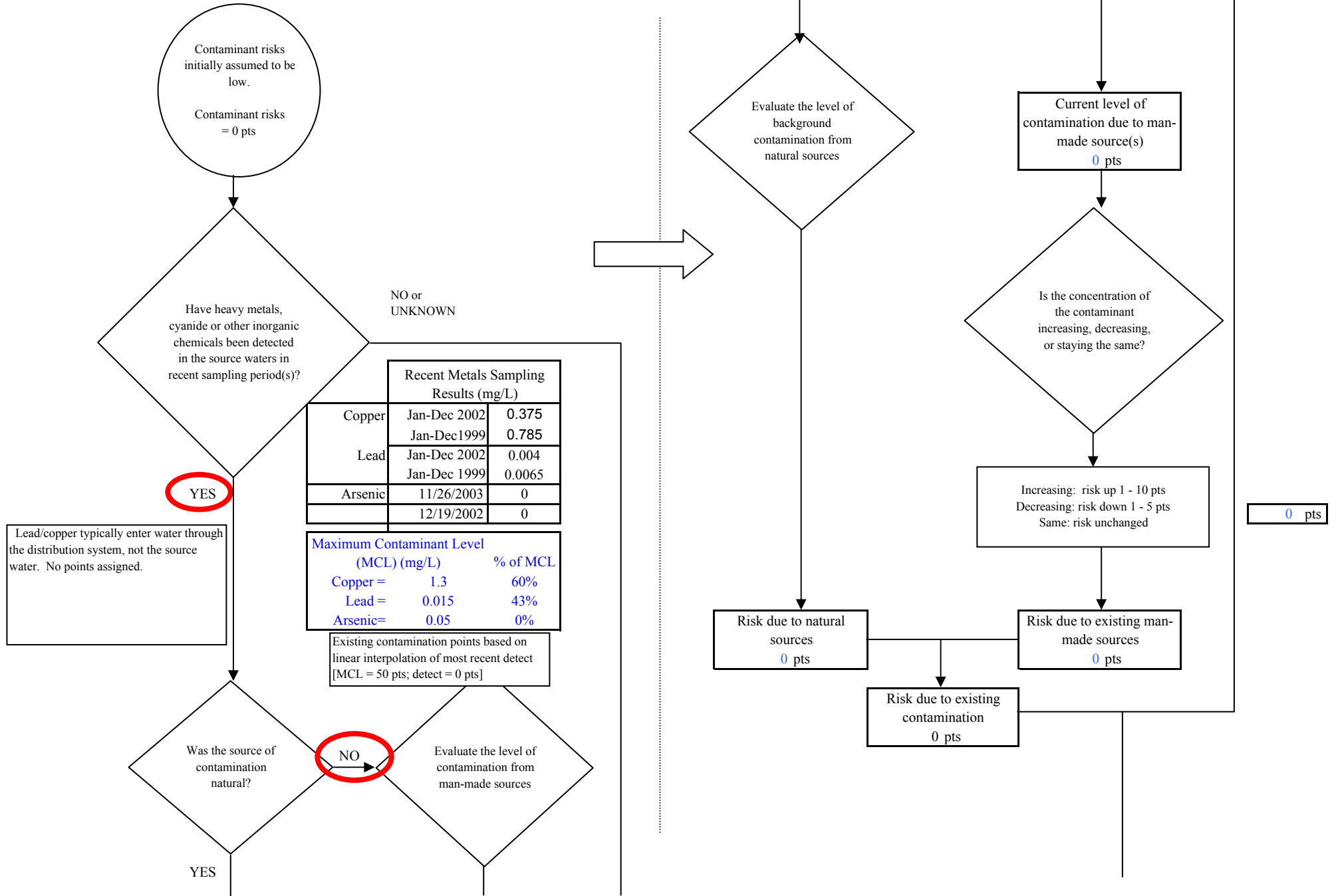
Chart 8. Contaminant risks for Alyeska Pipeline Service Co VMT East - Heavy Metals, Cyanide and Other Inorganic Chemicals
