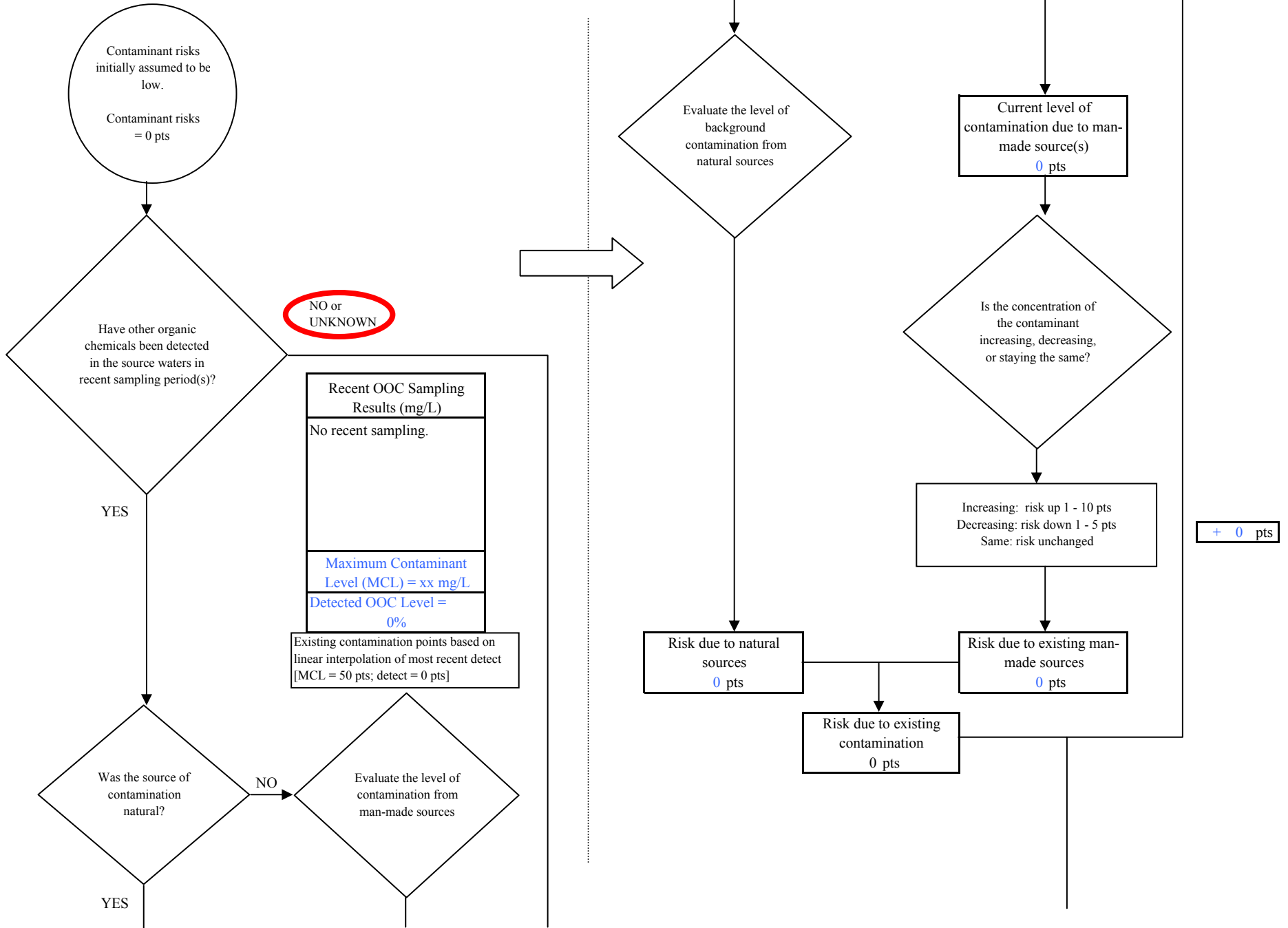
Chart 12. Contaminant risks for Alyeska Pipeline Service Co VMT East - Other Organic Chemicals
