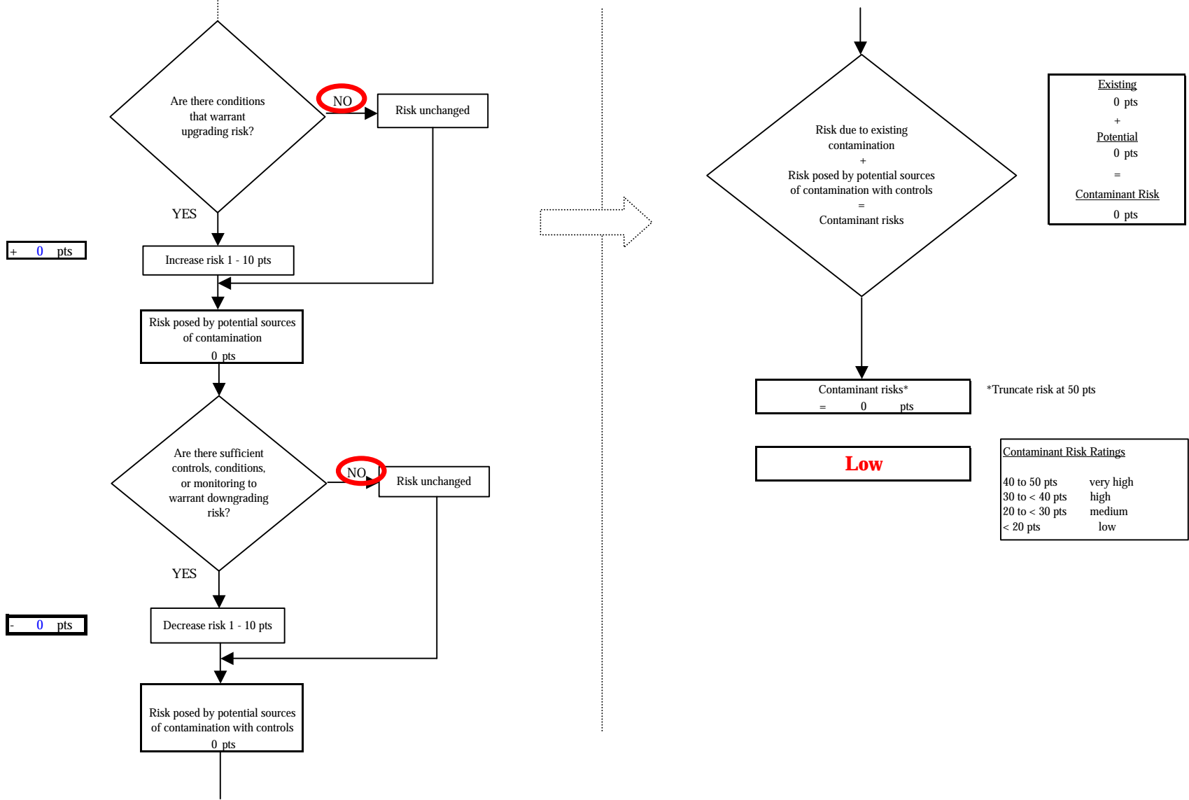
Chart 7. Contaminant risks for McHugh Creek (215647.001) - Volatile Organic Chemicals
