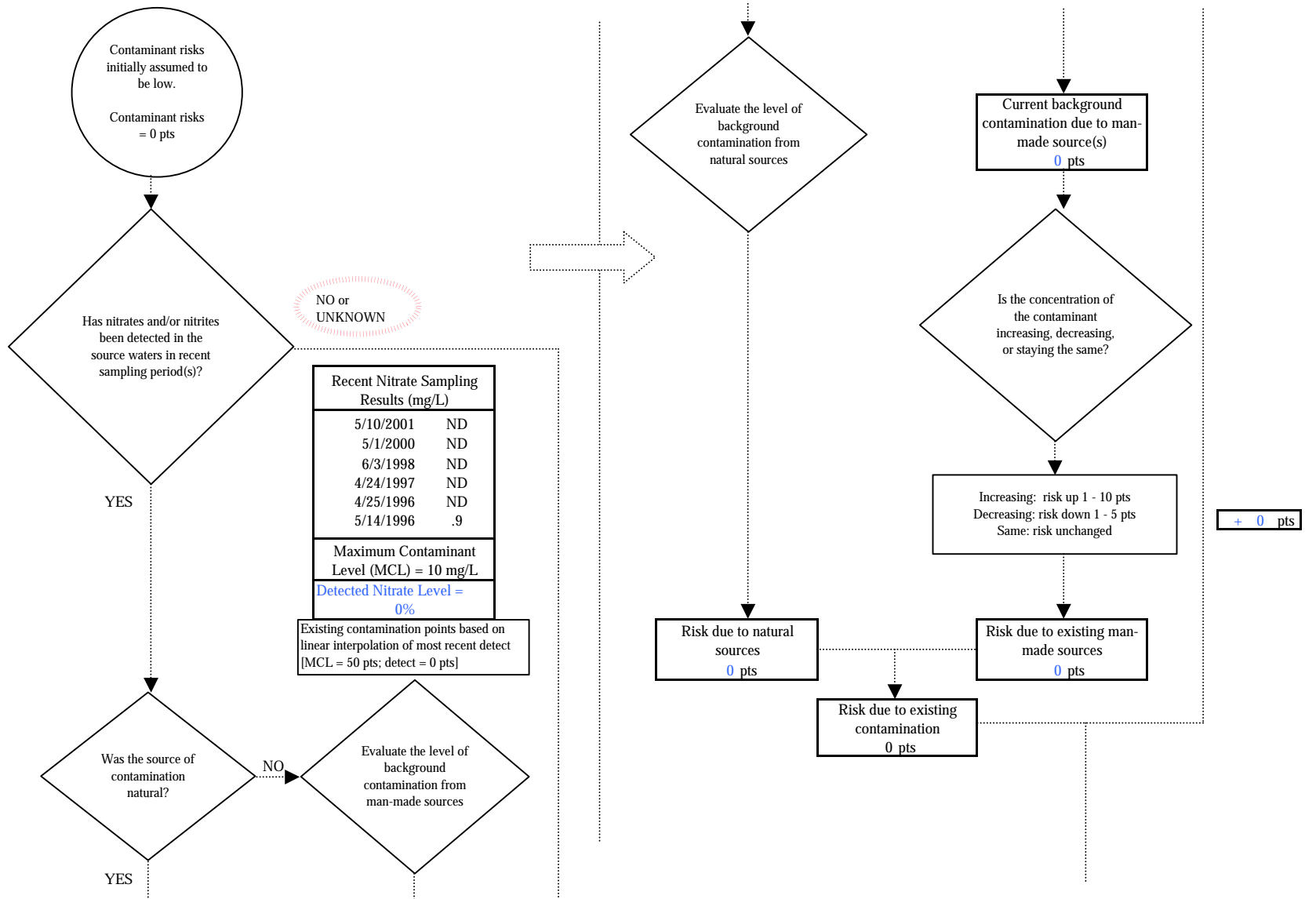
Chart 5. Contaminant risks for McHugh Creek (215647.001) - Nitrates and Nitrites
