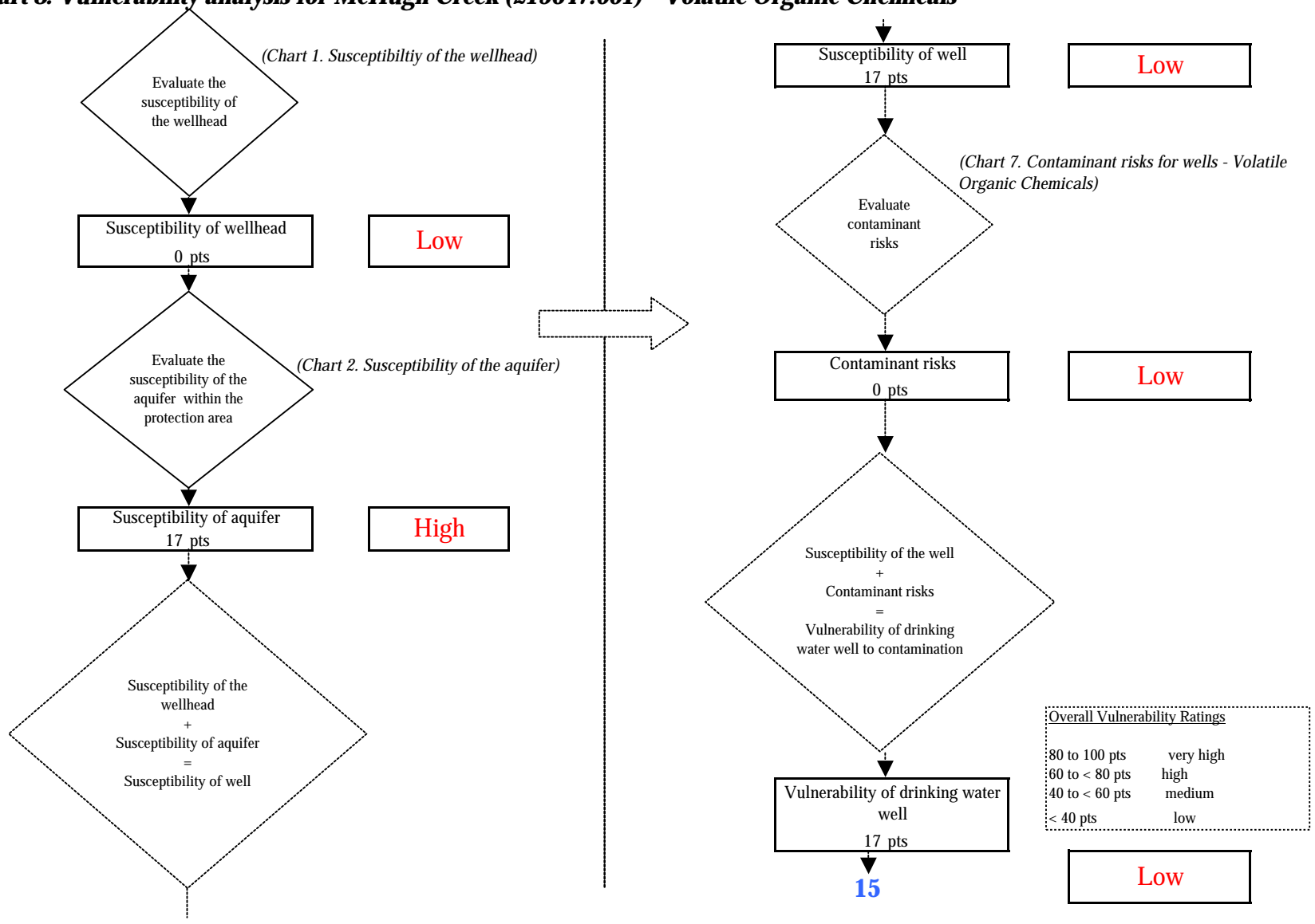
Chart 8. Vulnerability analysis for McHugh Creek (215647.001) - Volatile Organic Chemicals
