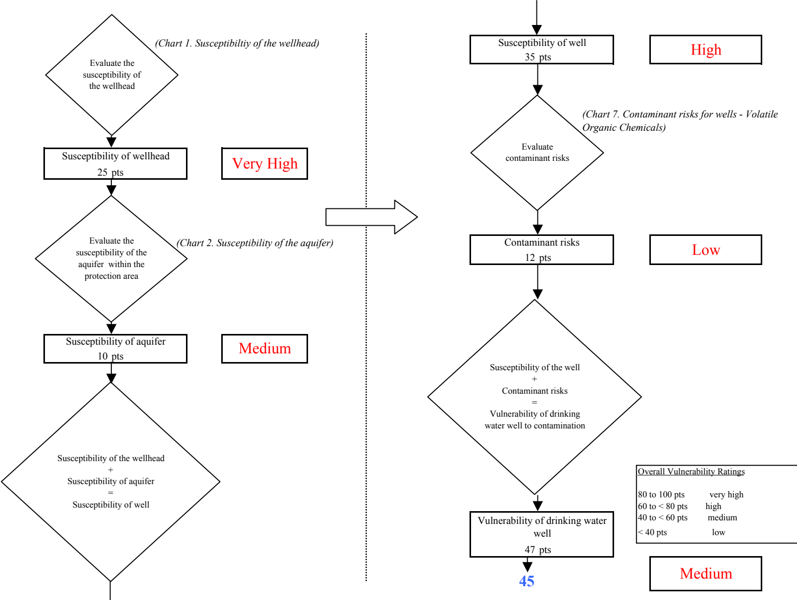
Chart 8. Vulnerability analysis for Abundant Life Assembly of God (245024.001) - Volatile Organic Chemicals
