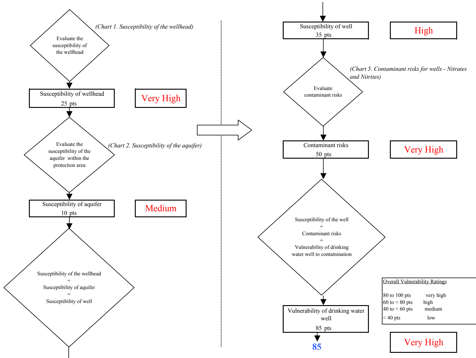
Chart 6. Vulnerability analysis for Abundant Life Assembly of God (245024.001) - Nitrates and Nitrites
