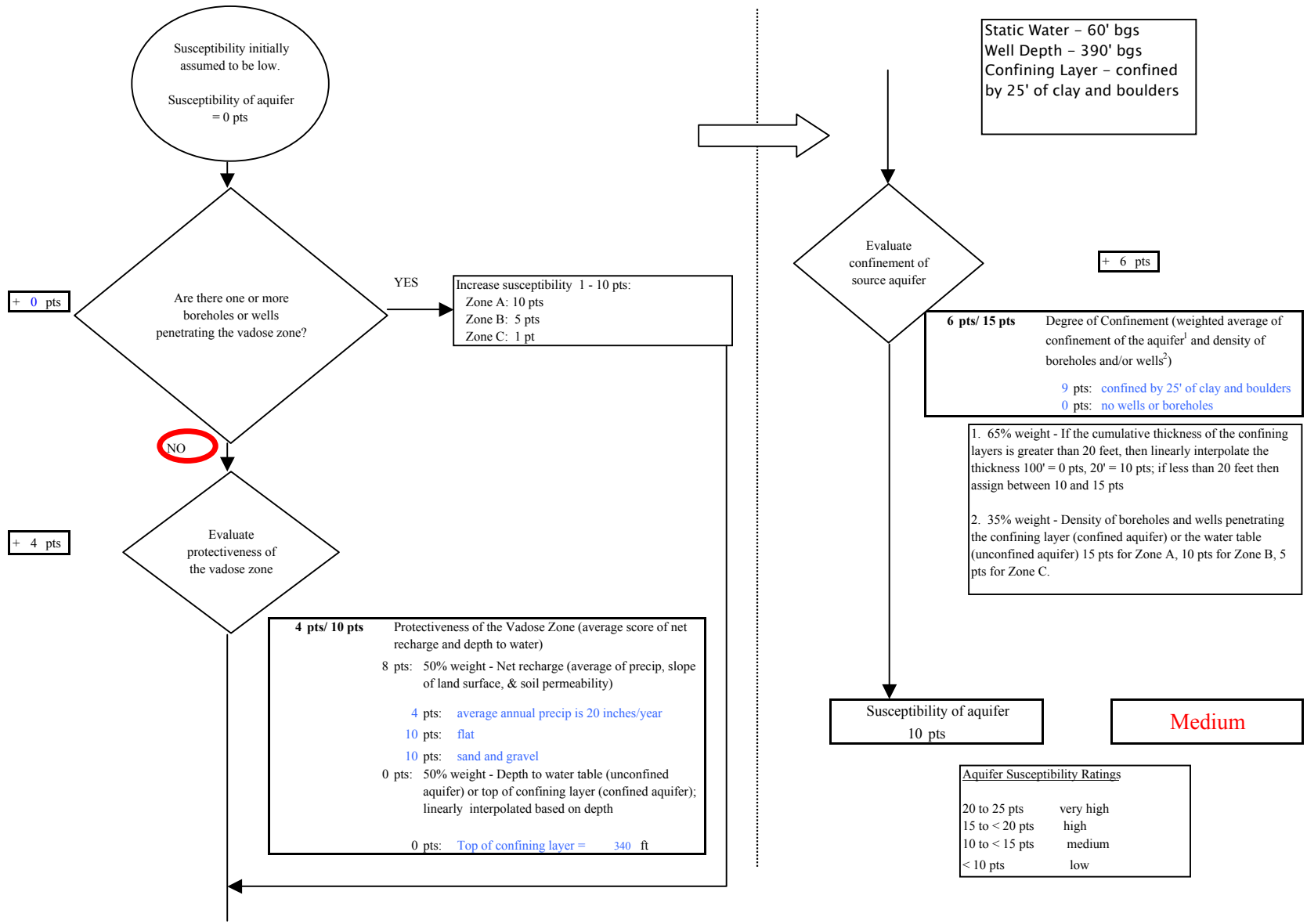
Chart 2. Susceptibility of the aquifer - Abundant Life Assembly of God (245024.001)
