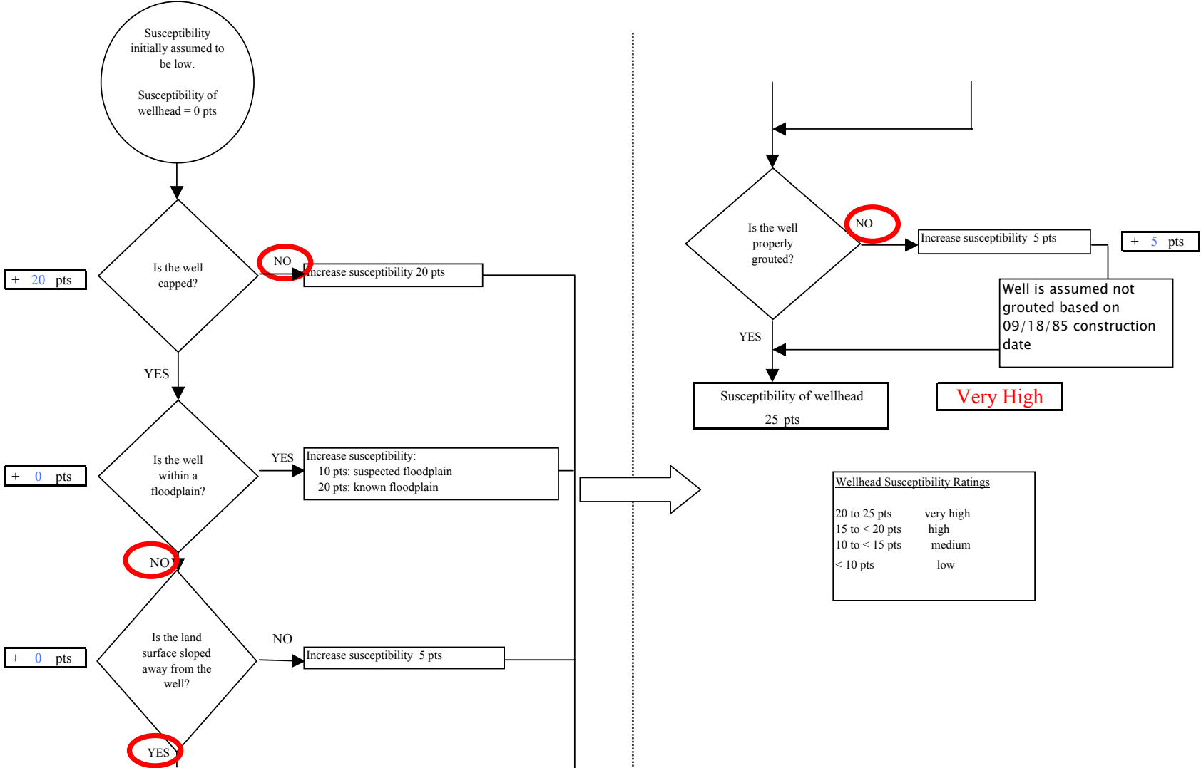
Chart 1. Susceptibility of the wellhead - Abundant Life Assembly of God (245024.001)
