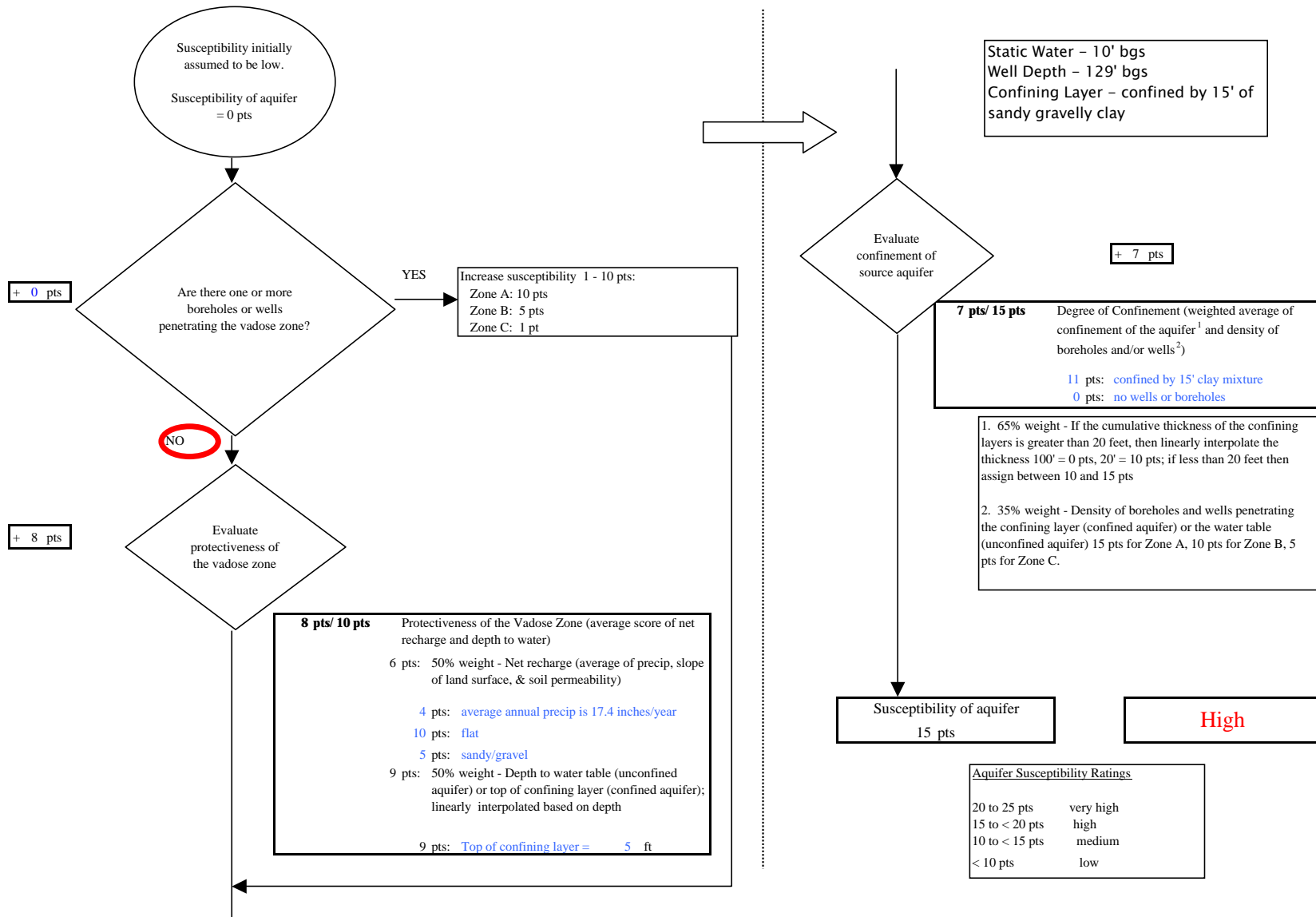
Chart 2. Susceptibility of the aquifer - Kenai Wilderness Lodge (247238.001)
