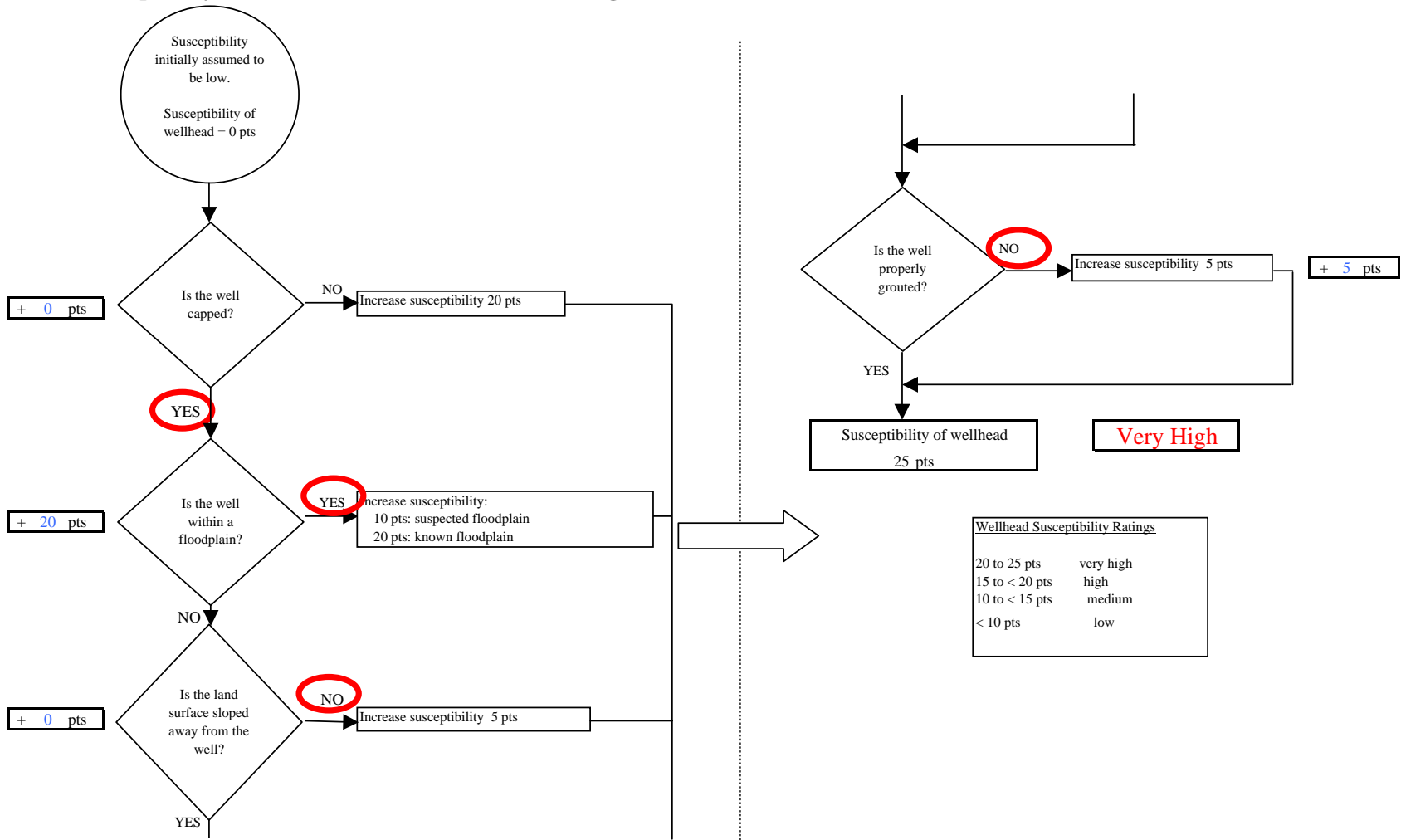
Chart 1. Susceptibility of the wellhead - Kenai Wilderness Lodge (247238.001)
