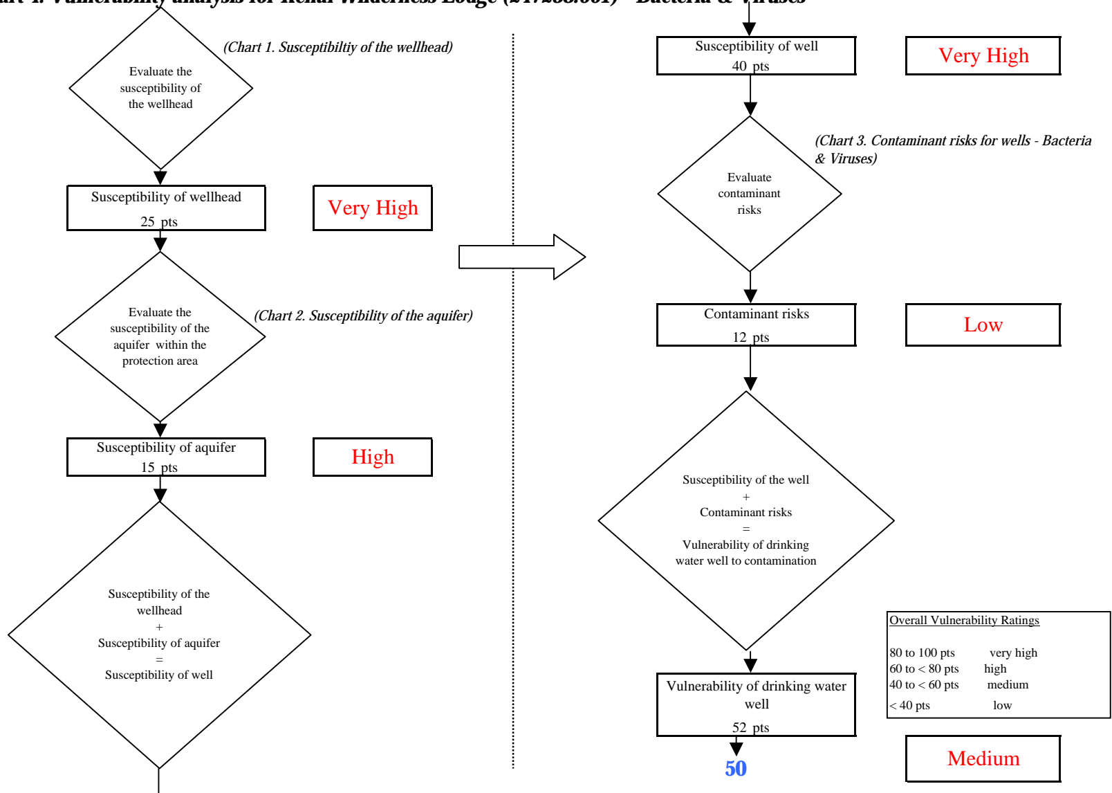
Chart 4. Vulnerability analysis for Kenai Wilderness Lodge (247238.001) - Bacteria & Viruses
