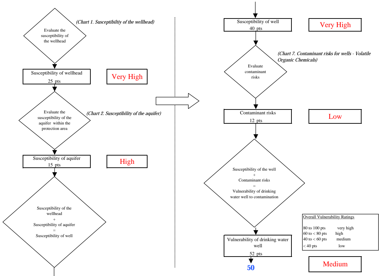
Chart 8. Vulnerability analysis for Kenai Wilderness Lodge (247238.001) - Volatile Organic Chemicals
