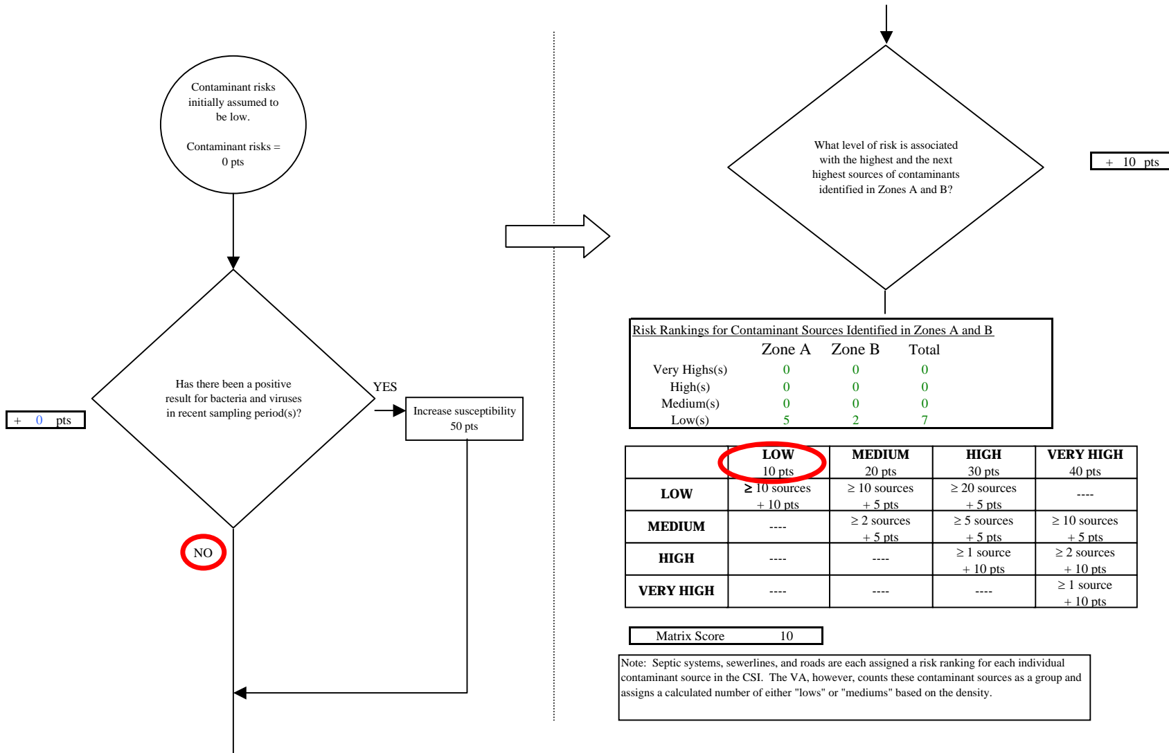
Chart 3. Contaminant risks for Kenai Wilderness Lodge (247238.001) - Bacteria & Viruses
