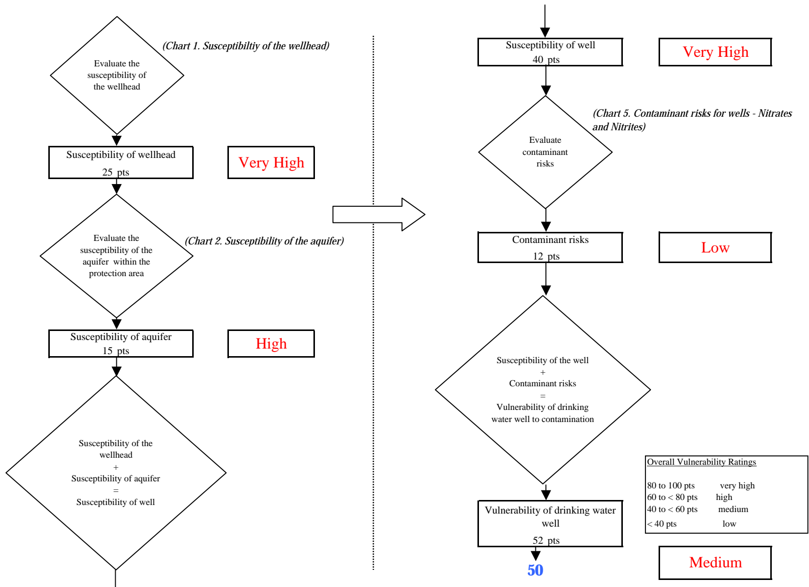
Chart 6. Vulnerability analysis for Kenai Wilderness Lodge (247238.001) - Nitrates and Nitrites
