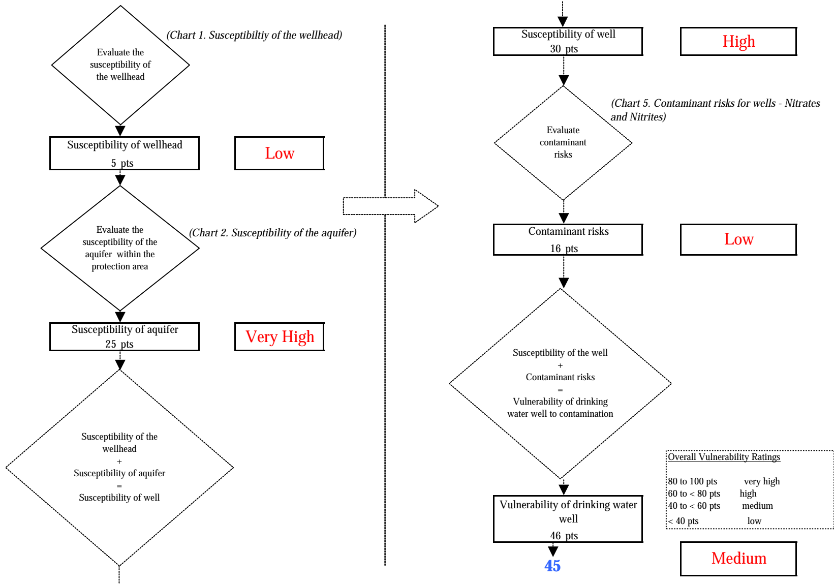
Chart 6. Vulnerability analysis for Upper Skilak Lake West (247872.001) - Nitrates and Nitrites
