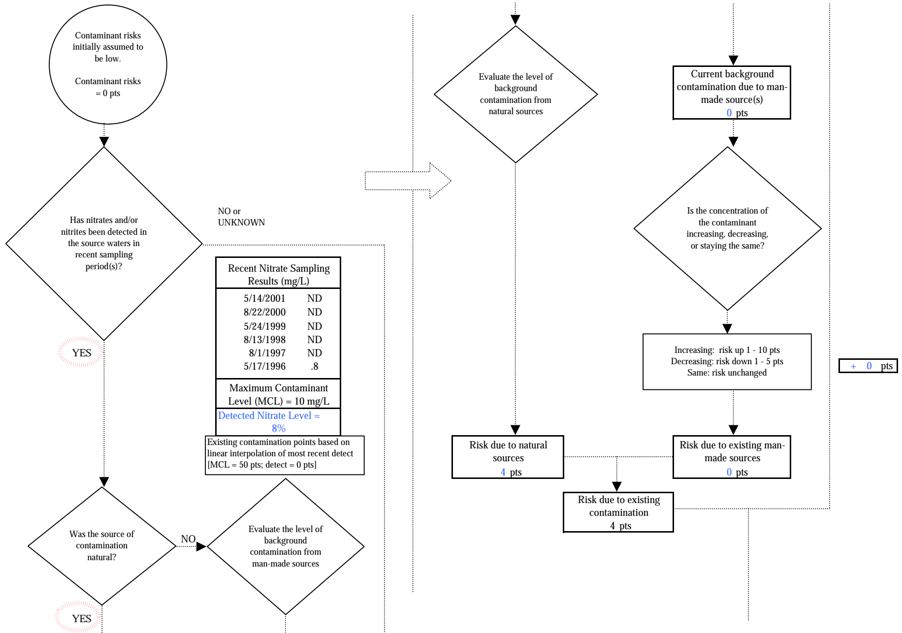
Chart 5. Contaminant risks for Upper Skilak Lake West (247872.001) - Nitrates and Nitrites
