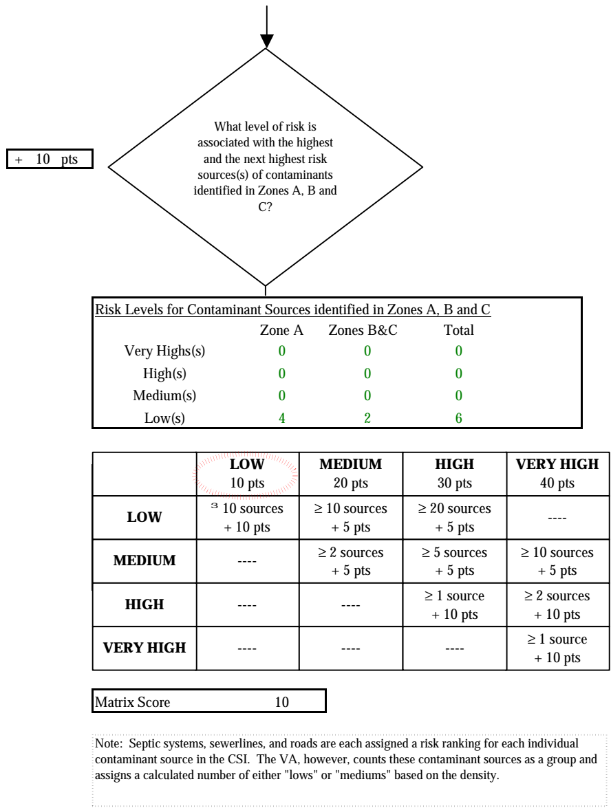
Chart 5. Contaminant risks for Upper Skilak Lake West (247872.001) - Nitrates and Nitrites
