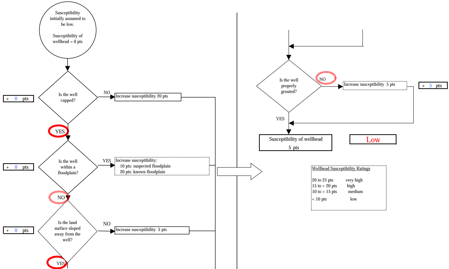
Chart 1. Susceptibility of the wellhead - Upper Skilak Lake West (247872.001)
