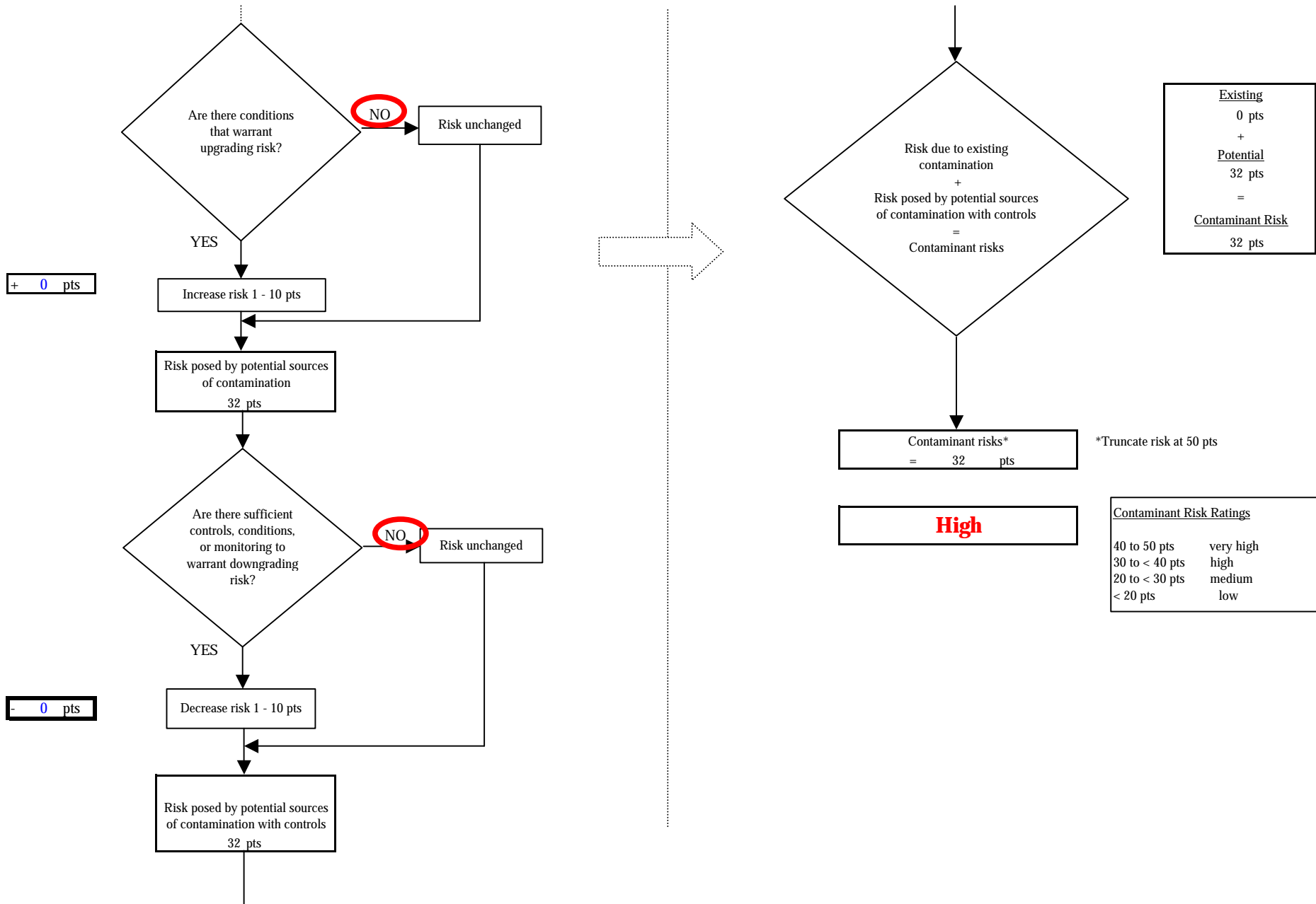
Chart 7. Contaminant risks for Upper Skilak Lake West (247872.001) - Volatile Organic Chemicals
