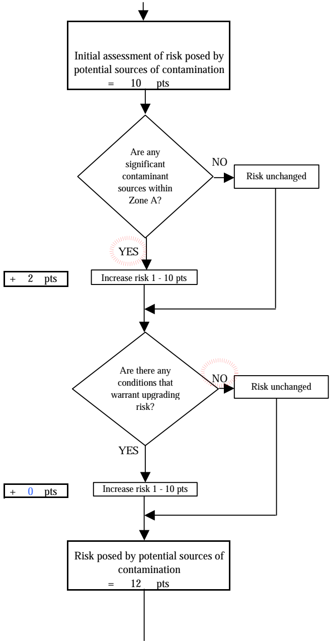
Chart 3. Contaminant risks for Upper Skilak Lake West (247872.001) - Bacteria & Viruses
