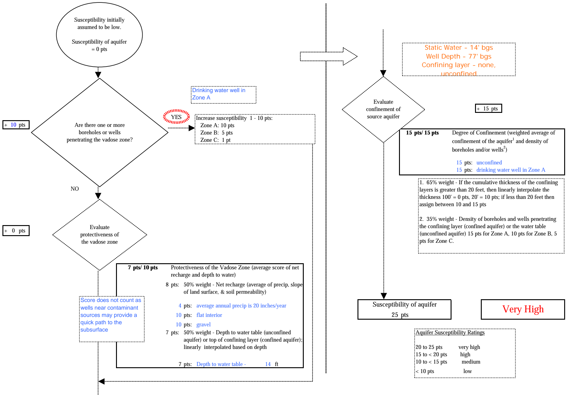
Chart 2. Susceptibility of the aquifer - Upper Skilak Lake West (247872.001)
