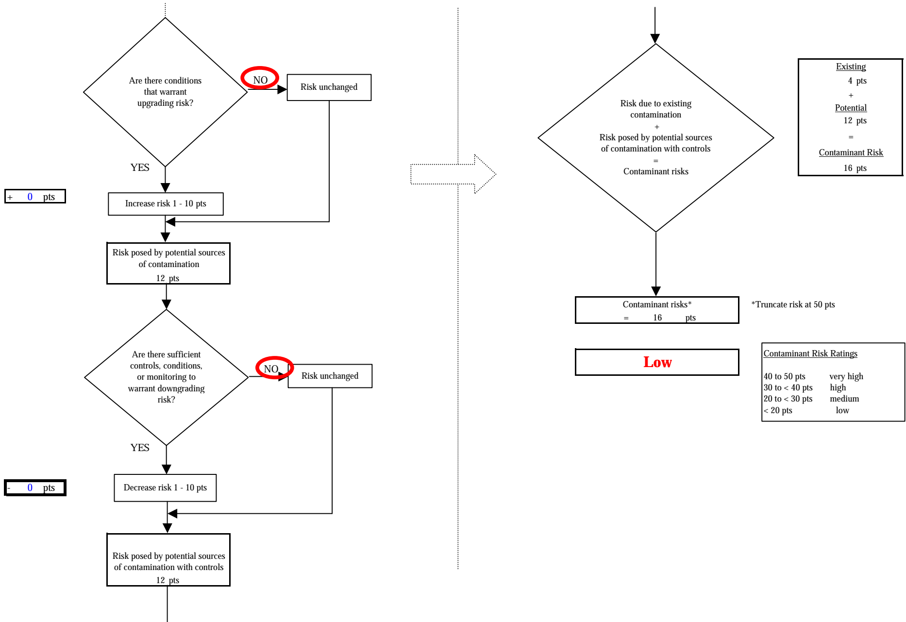
Chart 5. Contaminant risks for Upper Skilak Lake West (247872.001) - Nitrates and Nitrites
