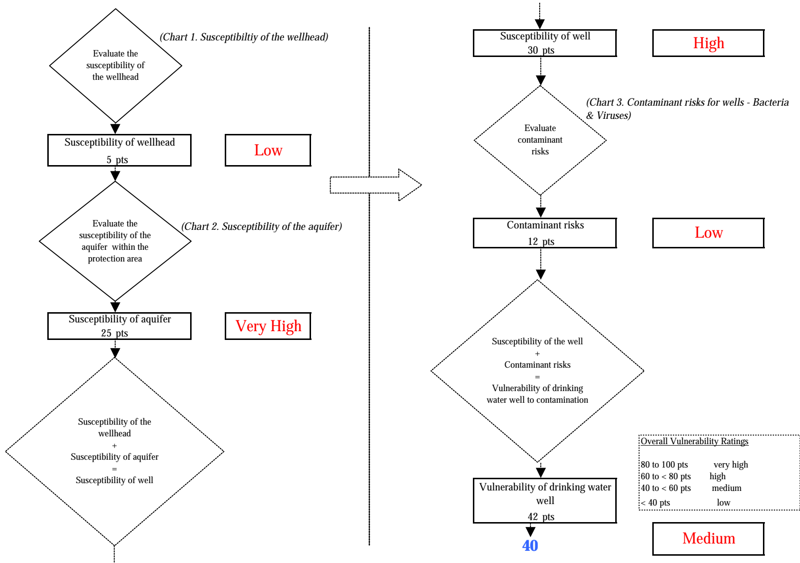
Chart 4. Vulnerability analysis for Upper Skilak Lake West (247872.001) - Bacteria & Viruses
