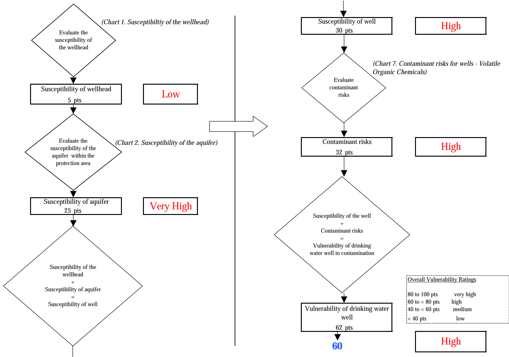
Chart 8. Vulnerability analysis for Upper Skilak Lake West (247872.001) - Volatile Organic Chemicals
