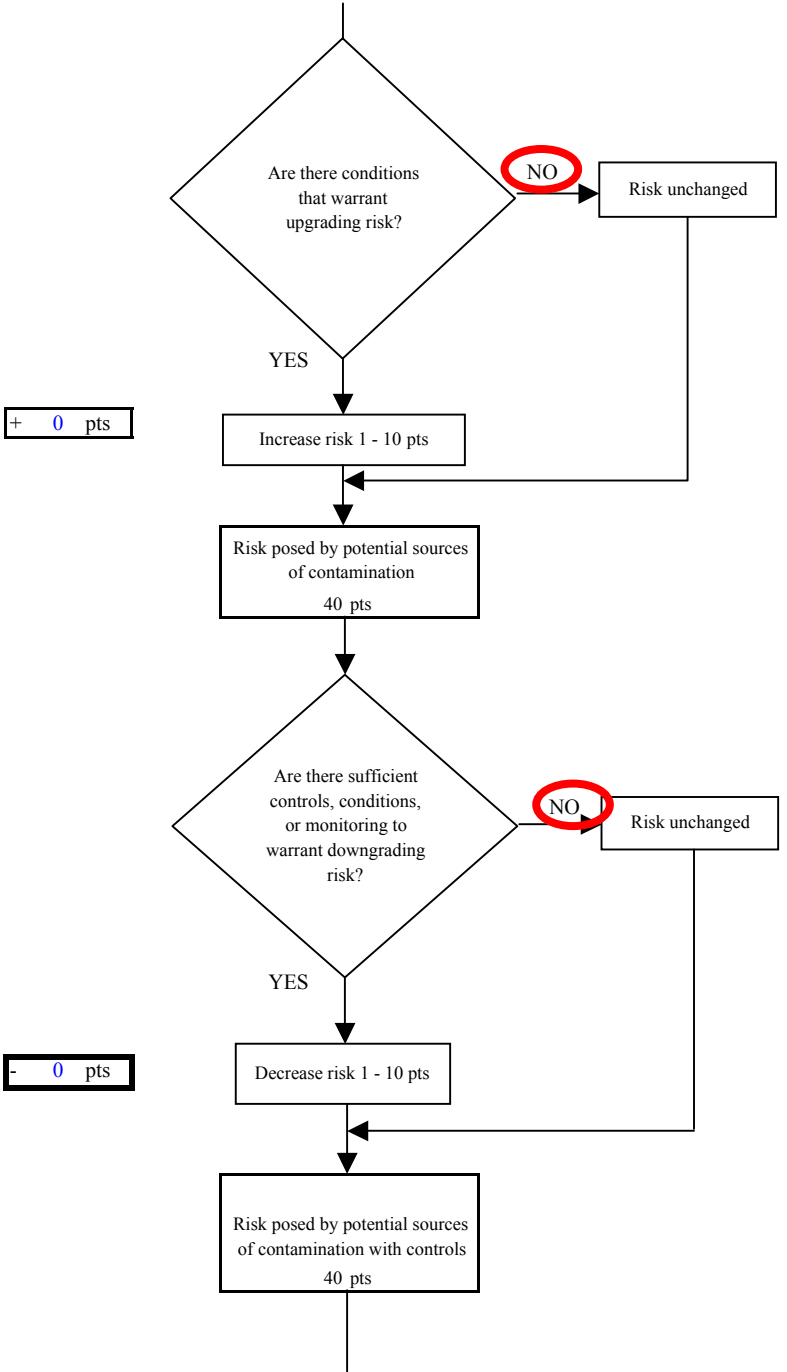
Chart 5. Contaminant risks for Lowell Point Condos - Nitrates and Nitrites
