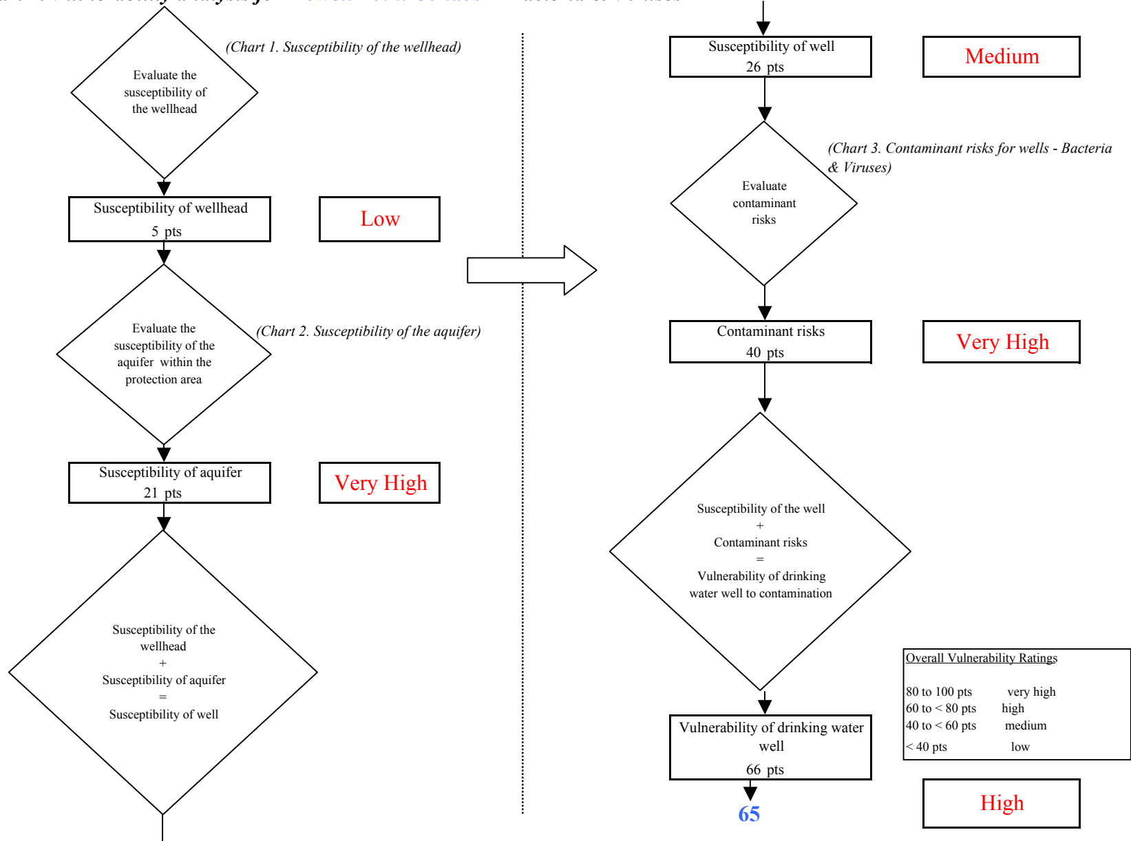
Chart 4. Vulnerability analysis for Lowell Point Condos - Bacteria & Viruses
