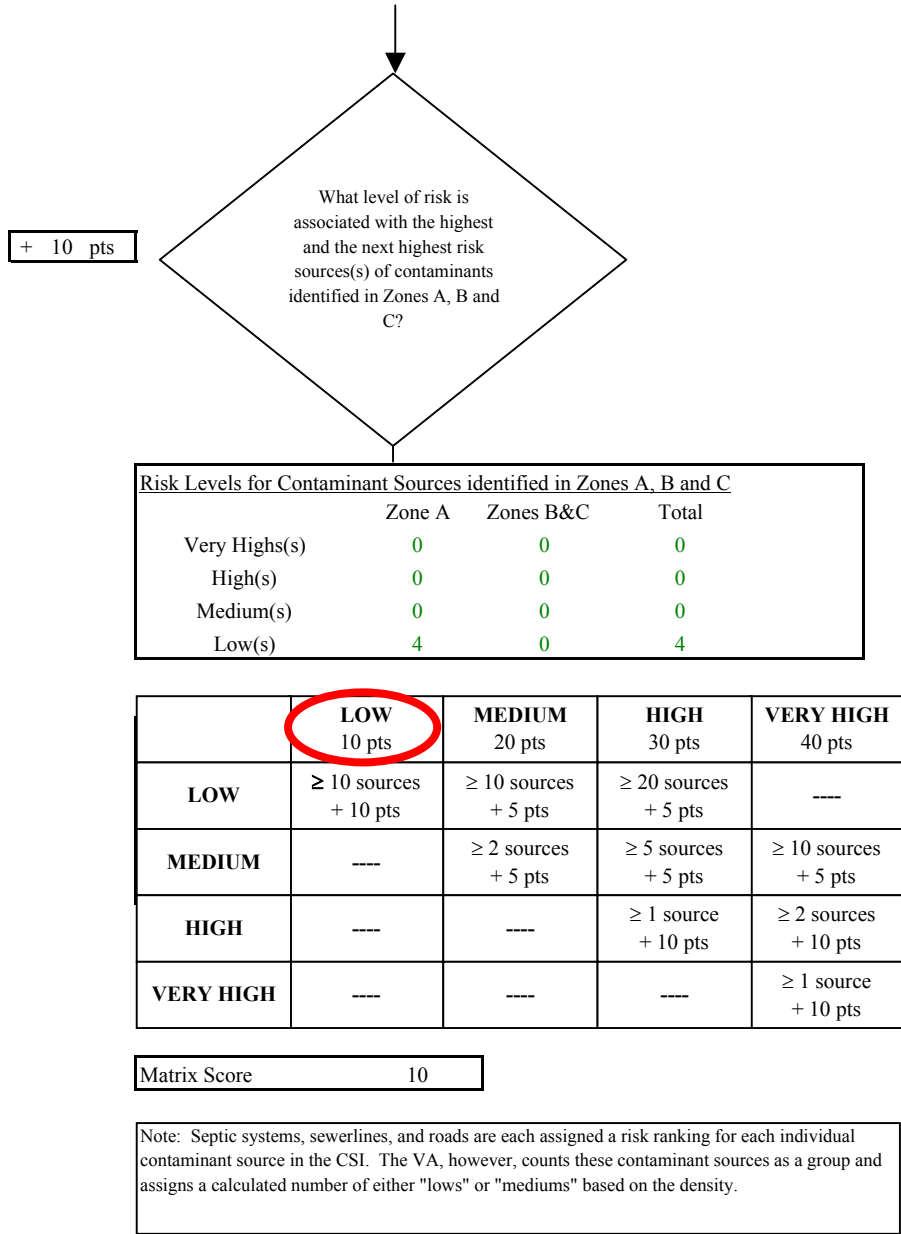
Chart 7. Contaminant risks for Lowell Point Condos - Volatile Organic Chemicals
