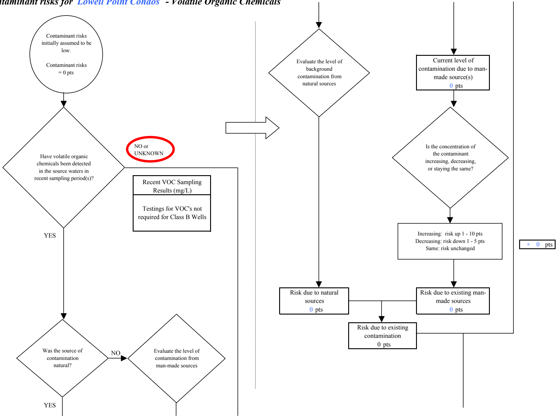
Chart 7. Contaminant risks for Lowell Point Condos - Volatile Organic Chemicals
