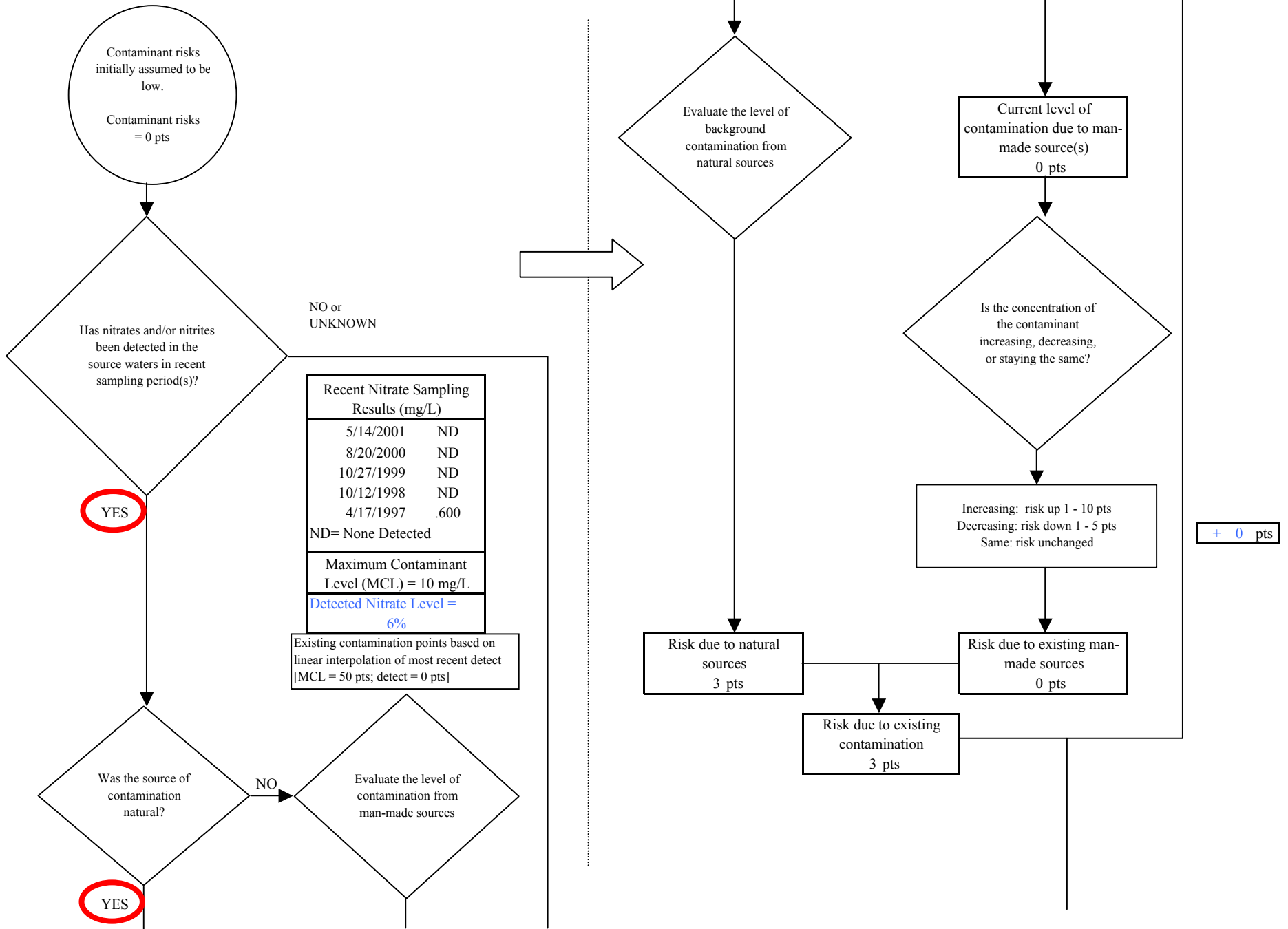
Chart 5. Contaminant risks for Lowell Point Condos - Nitrates and Nitrites
