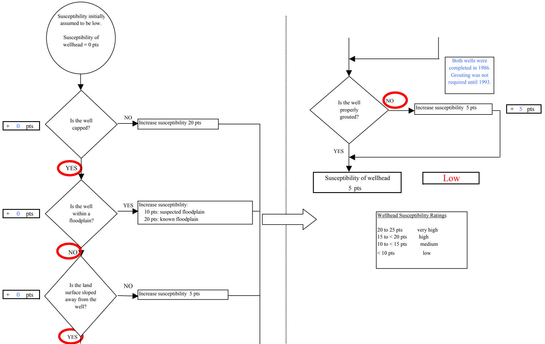
Chart 1. Susceptibility of the wellhead - Lowell Point Condos
