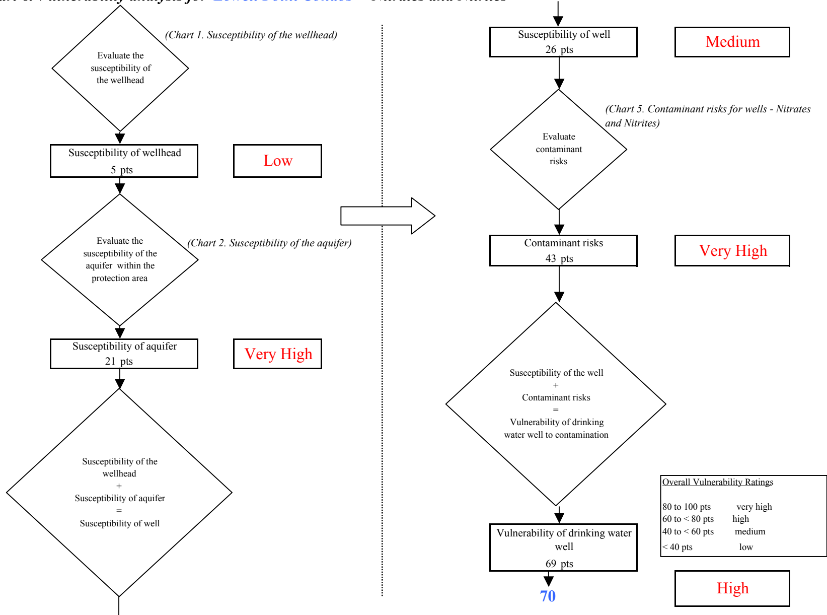
Chart 6. Vulnerability analysis for Lowell Point Condos - Nitrates and Nitrites
