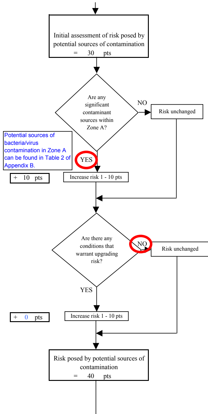
Chart 3. Contaminant risks for Lowell Point Condos - Bacteria & Viruses
