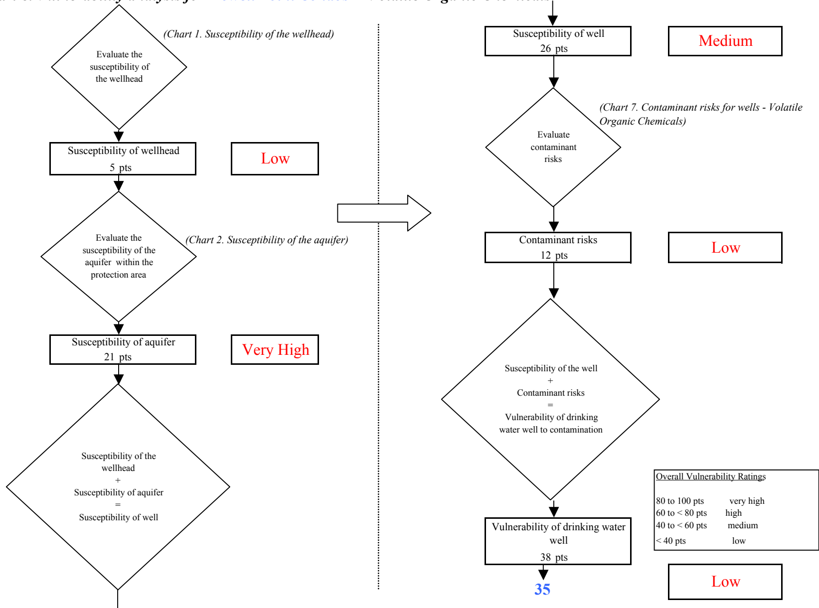
Chart 8. Vulnerability analysis for Lowell Point Condos - Volatile Organic Chemicals
