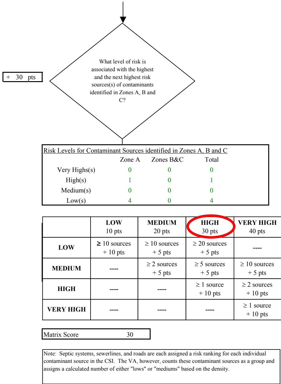
Chart 5. Contaminant risks for Lowell Point Condos - Nitrates and Nitrites
