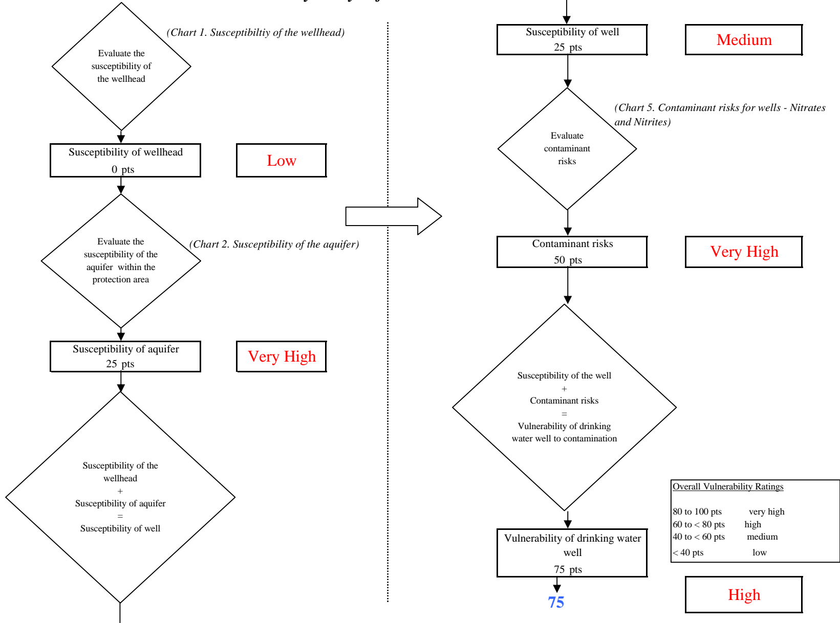
Chart 6. Vulnerability Analysis for Forks Roadhouse - Nitrates and Nitrites
