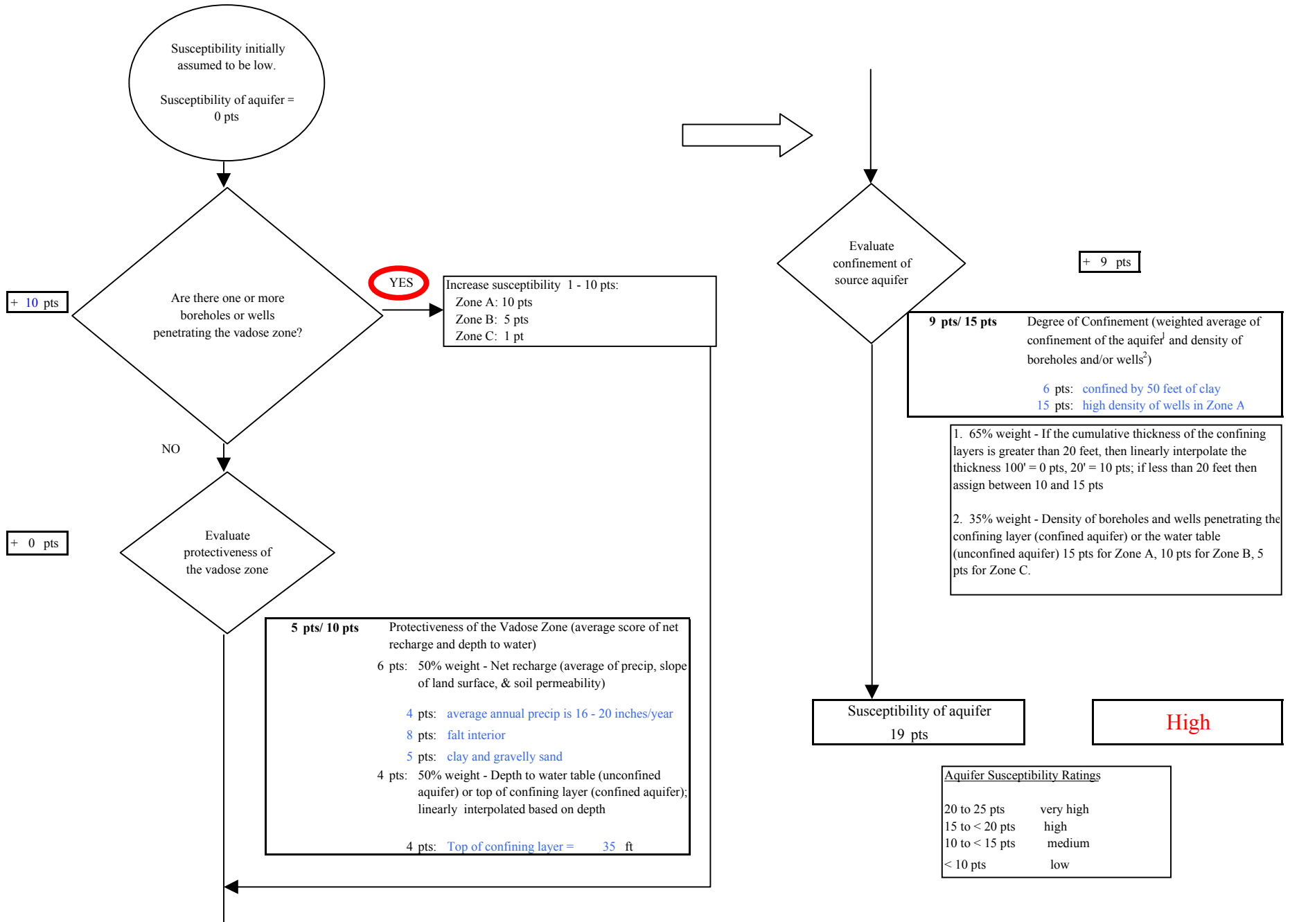
Chart 2. Susceptibility of the aquifer - Valley Baptist Tabernacle
