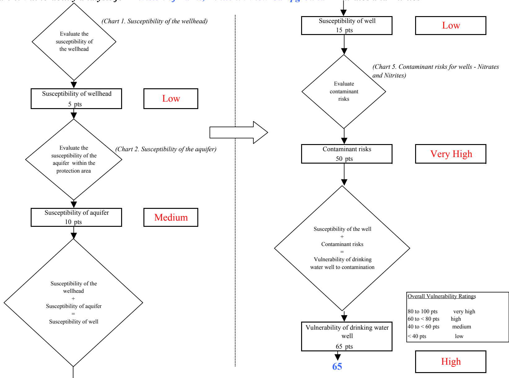
Chart 6. Vulnerability analysis for Division of Parks, Ninilchik View Campground - Nitrates and Nitrites
