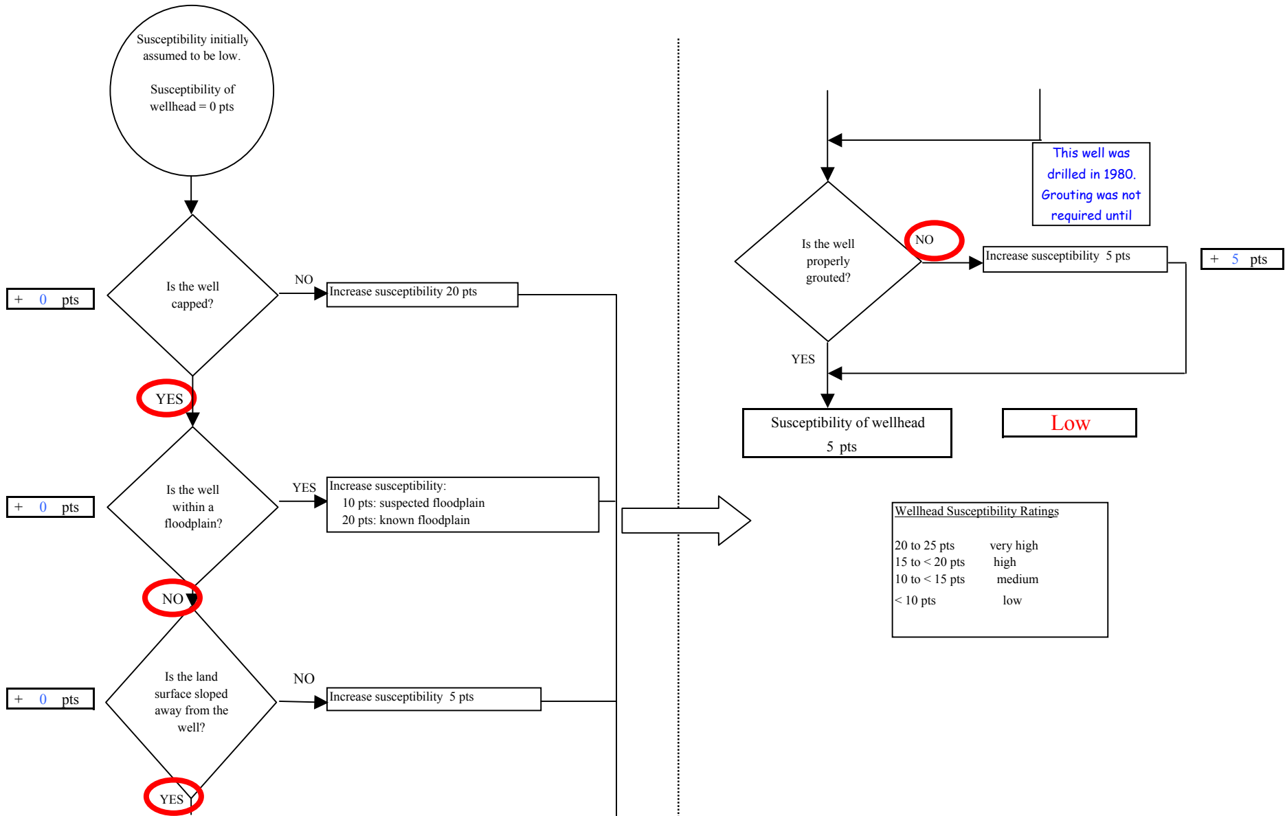
Chart 1. Susceptibility of the wellhead - Division of Parks, Ninilchik View Campground
