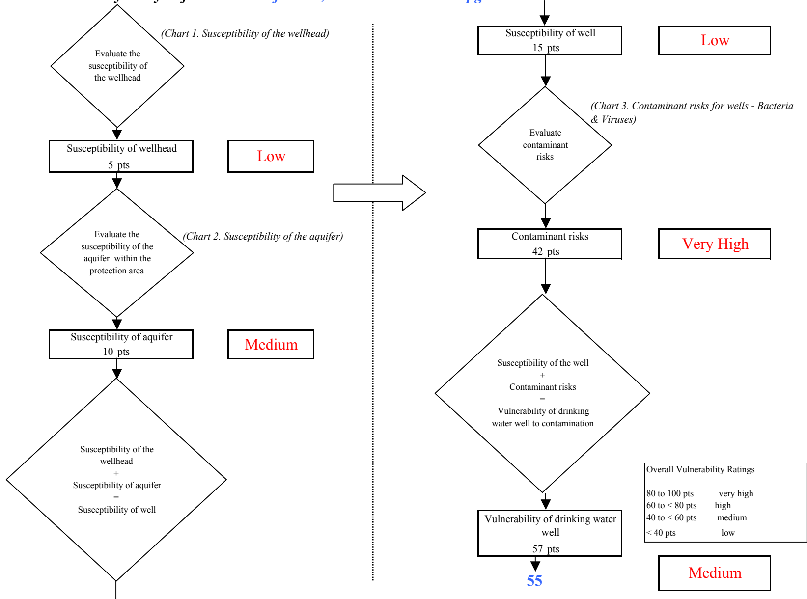
Chart 4. Vulnerability analysis for Division of Parks, Ninilchik View Campground - Bacteria & Viruses
