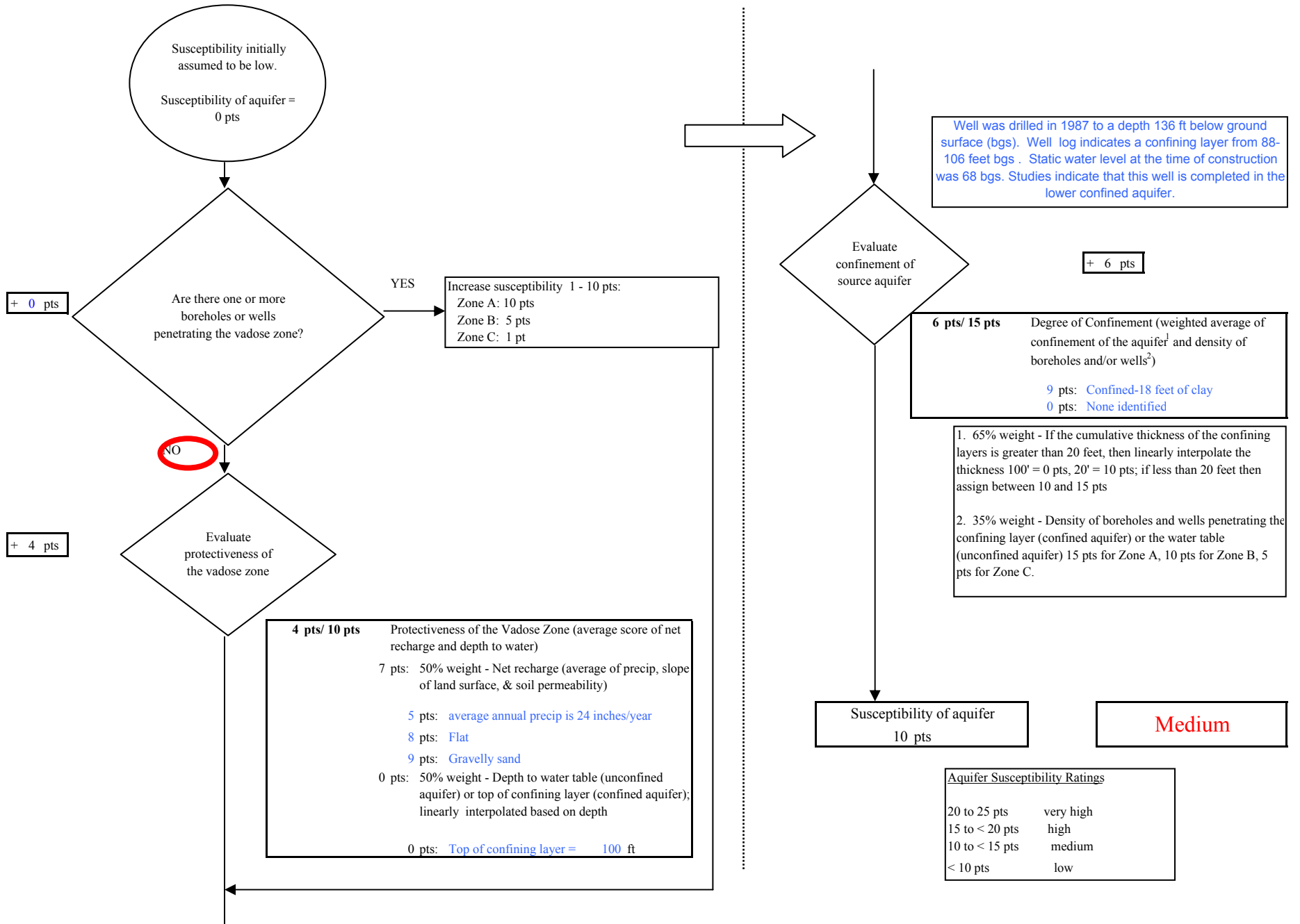
Chart 2. Susceptibility of the aquifer - Tesoro Alaska Petroleum Refinery PWSID 241745.001
