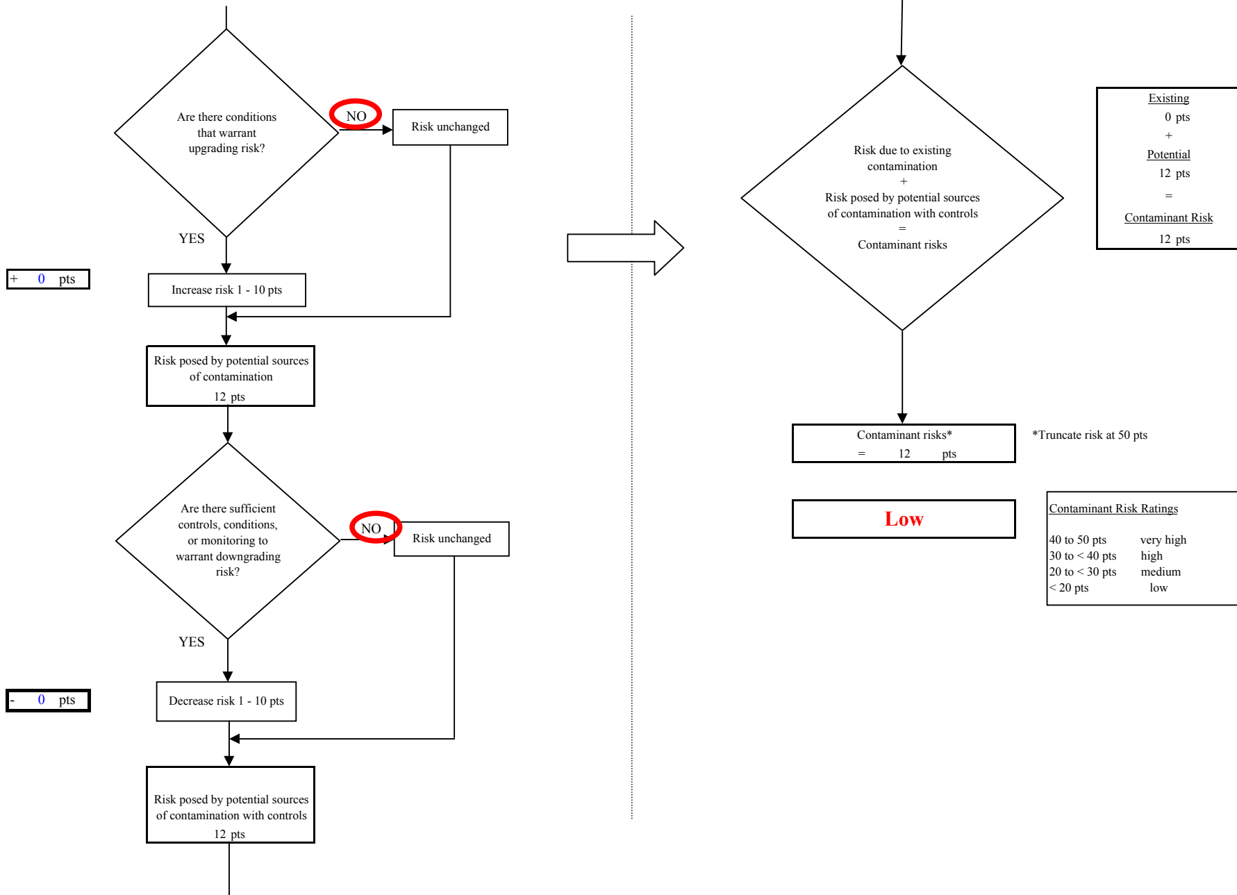
Chart 13. Contaminant risks for Tesoro Alaska Petroleum Refinery PWSID 241745.001 - Other Organic Chemicals
