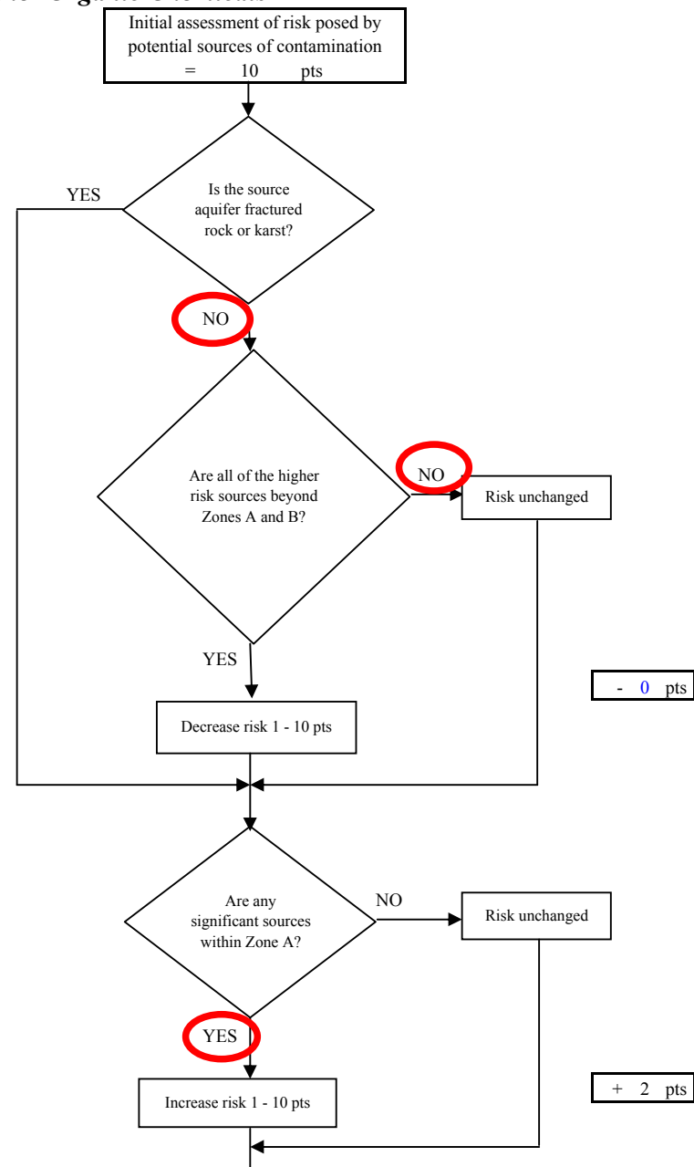
Chart 13. Contaminant risks for Tesoro Alaska Petroleum Refinery PWSID 241745.001 - Other Organic Chemicals
