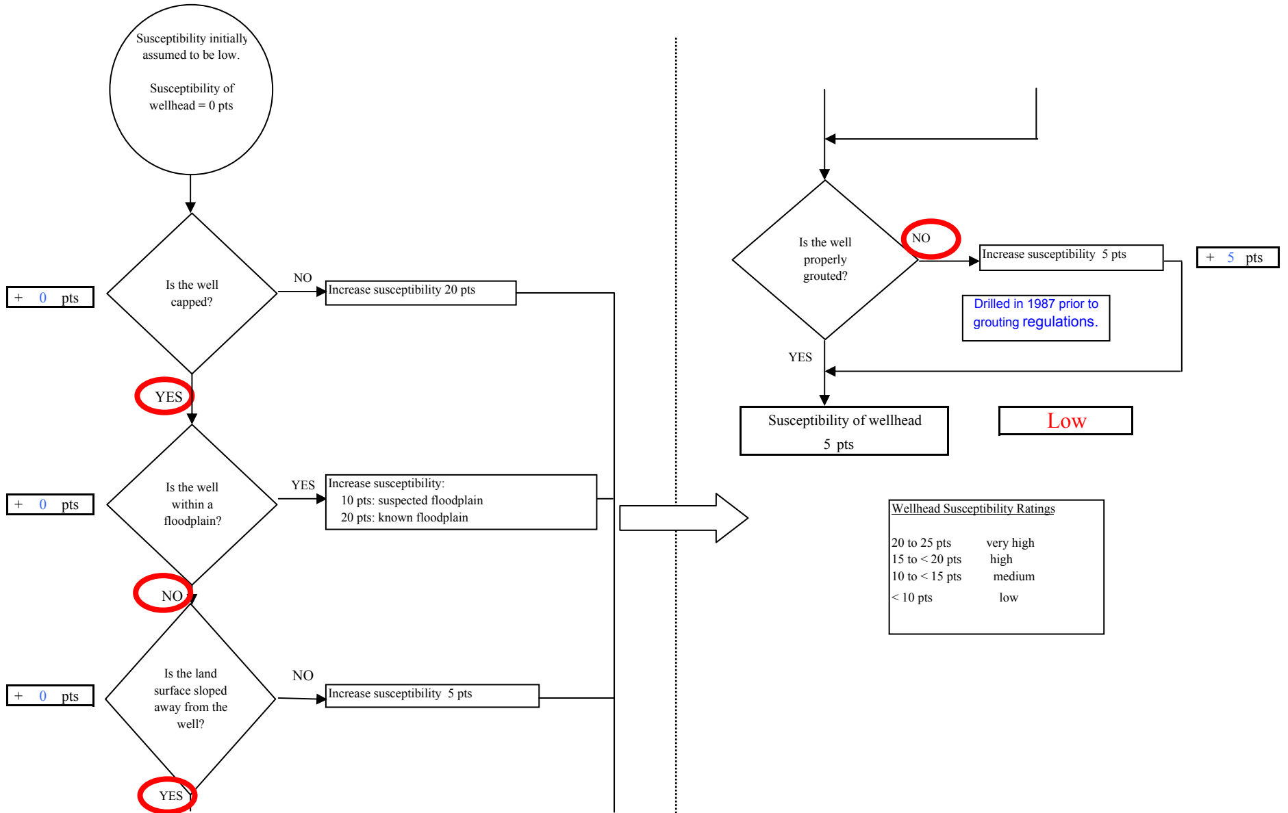
Chart 1. Susceptibility of the wellhead - Tesoro Alaska Petroleum Refinery PWSID 241745.001
