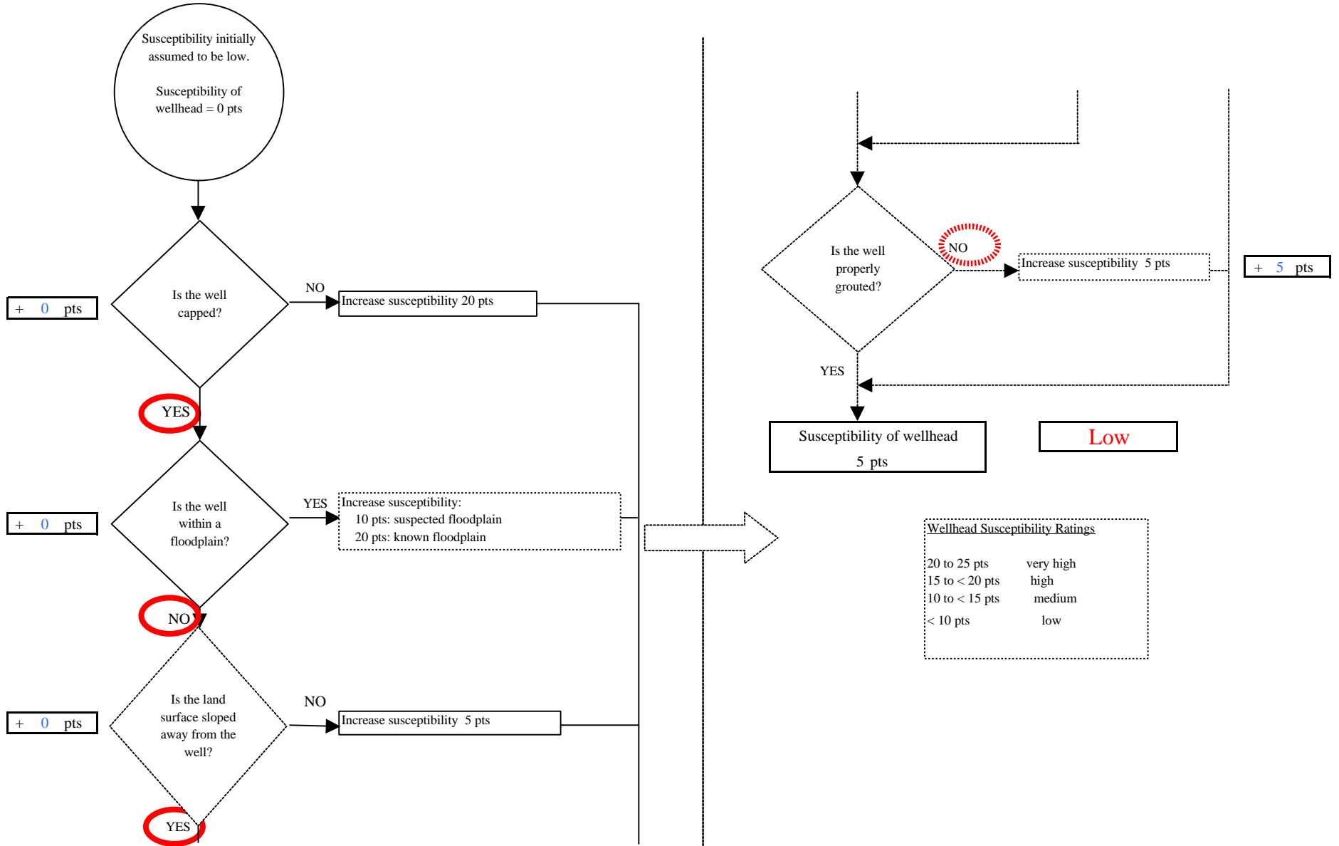
Chart 1. Susceptibility of the wellhead - Sourdough Cabins
