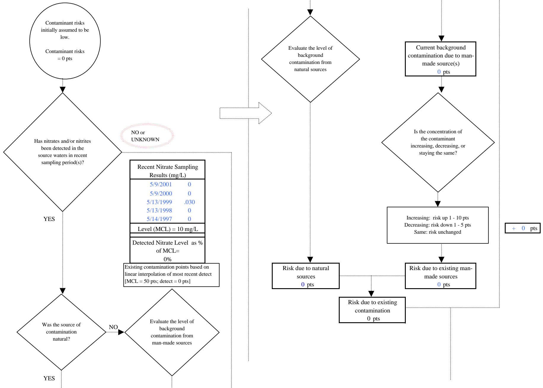
Chart 5. Contaminant risks for Sourdough Cabins - Nitrates and Nitrites
