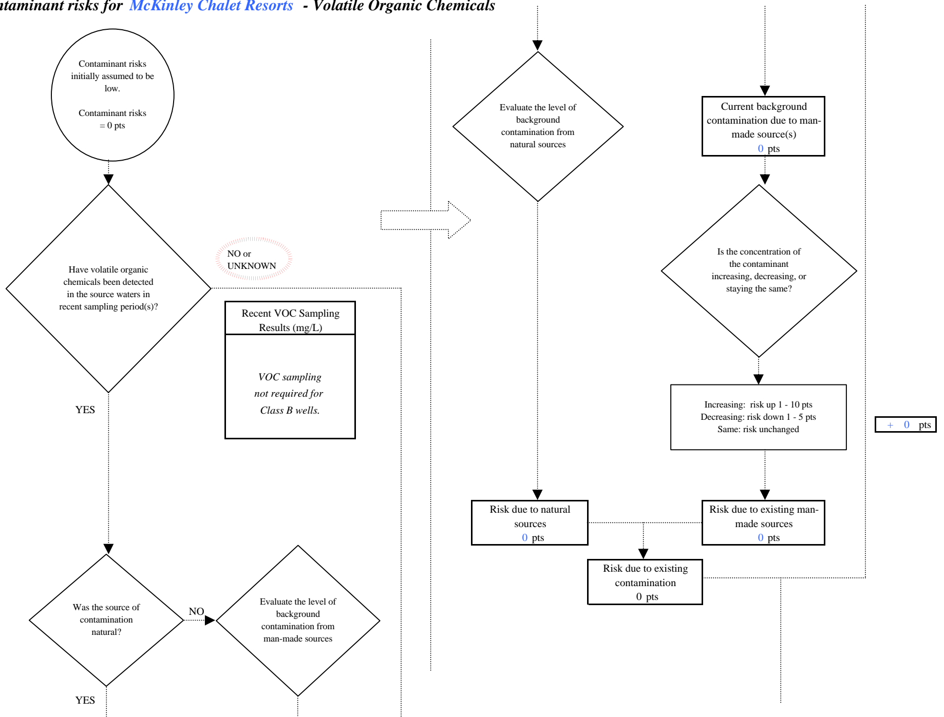
Chart 7. Contaminant risks for McKinley Chalet Resorts - Volatile Organic Chemicals
