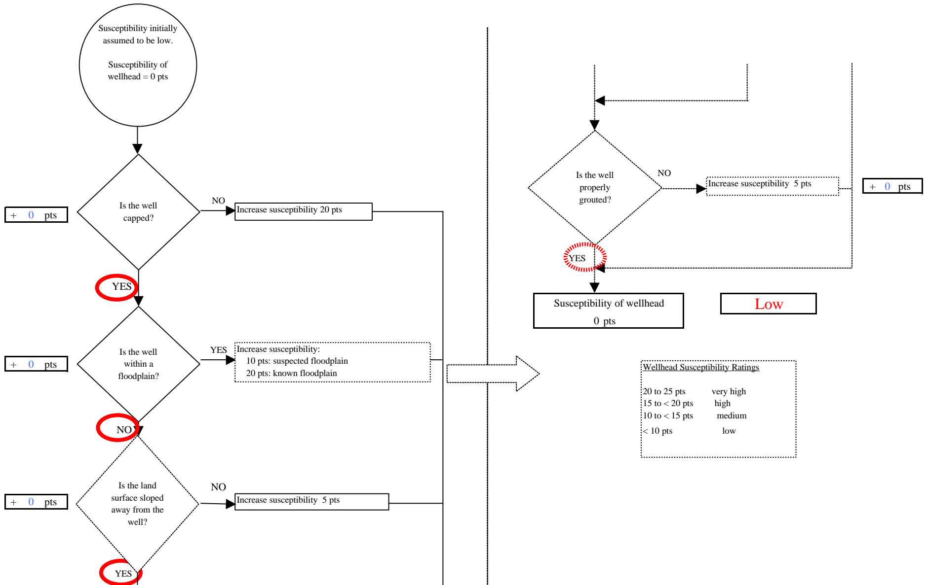
Chart 1. Susceptibility of the wellhead - McKinley Chalet Resorts
