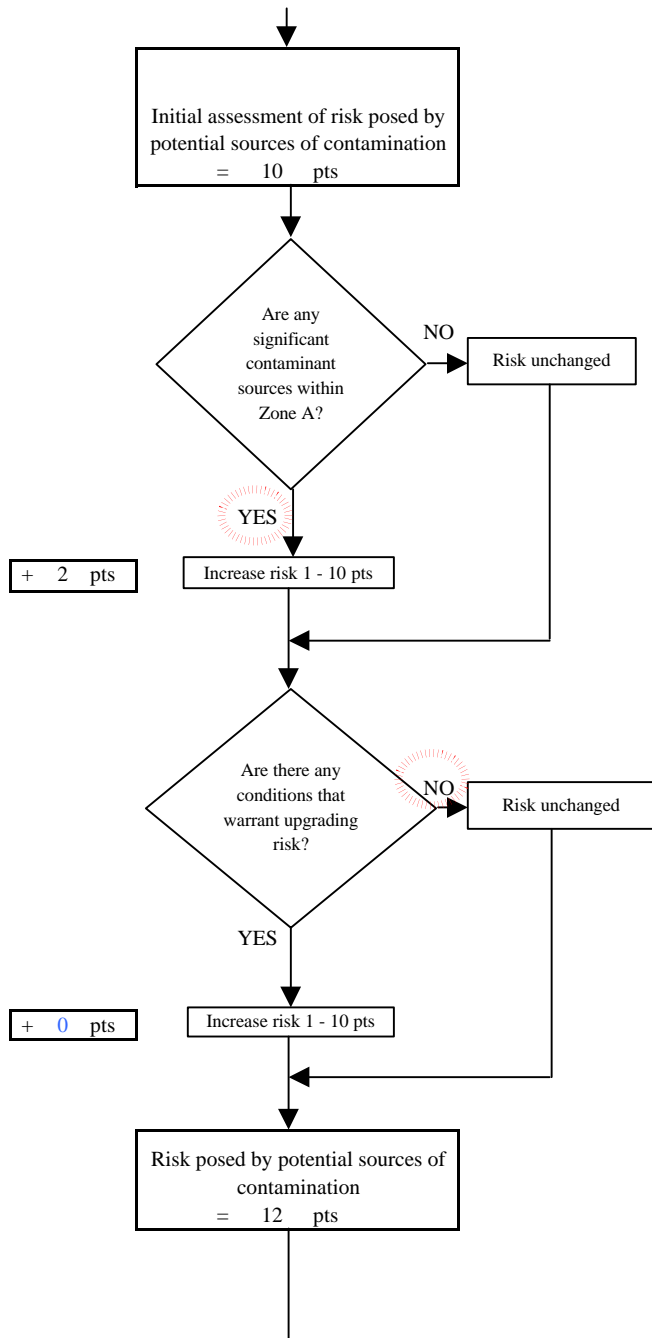
Chart 3. Contaminant risks for McKinley Chalet Resorts - Bacteria & Viruses
