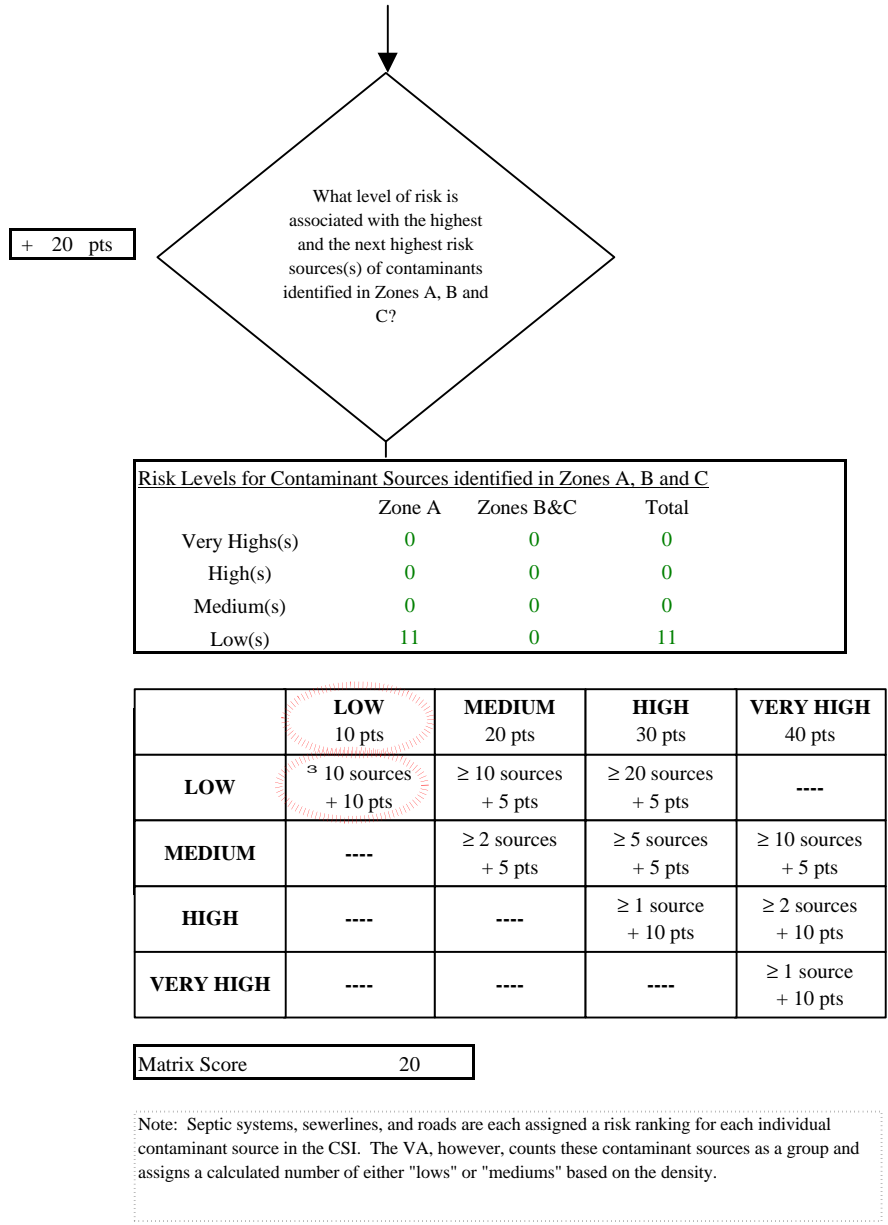
Chart 5. Contaminant risks for McKinley Chalet Resorts - Nitrates and Nitrites
