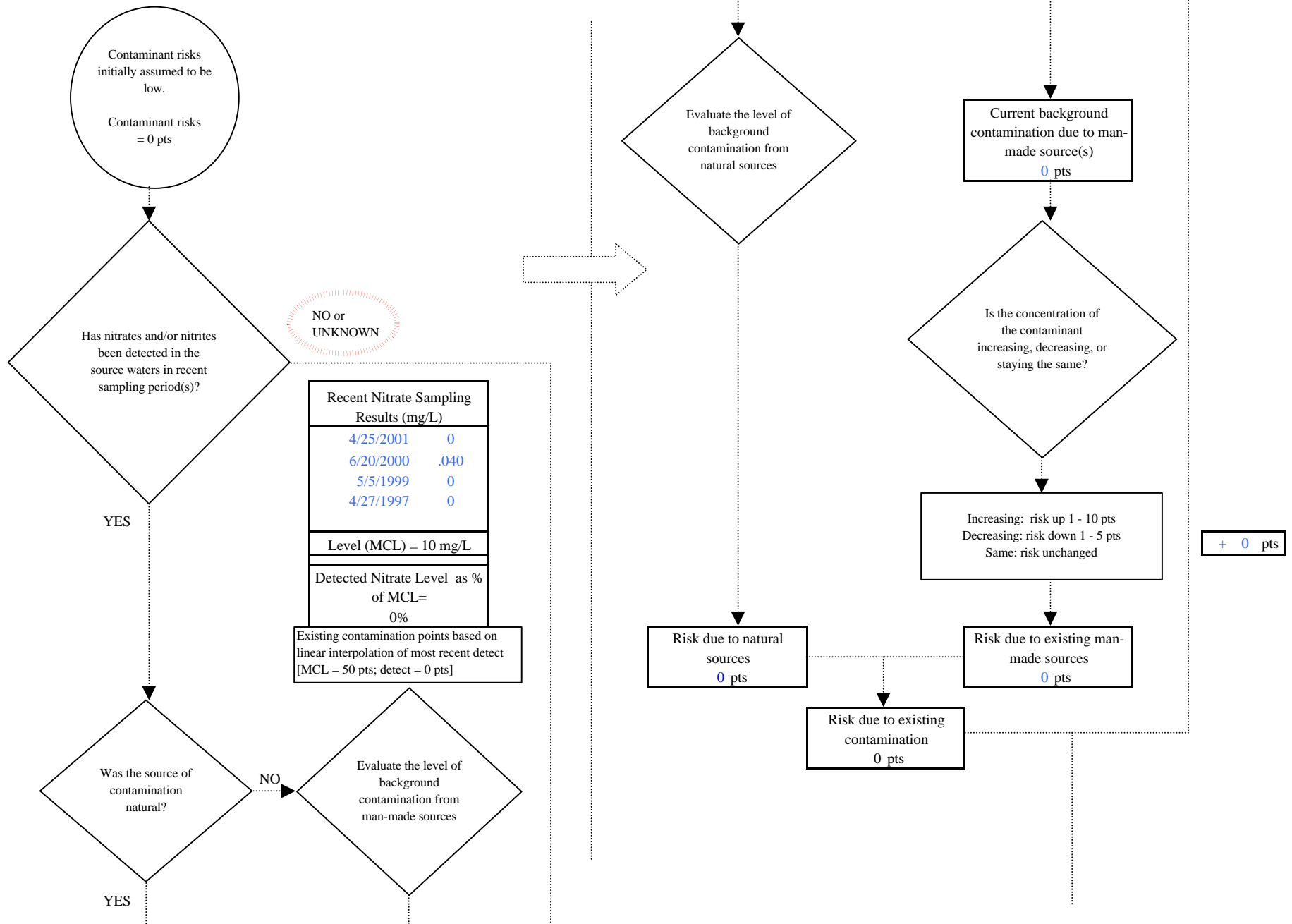
Chart 5. Contaminant risks for McKinley Chalet Resorts - Nitrates and Nitrites
