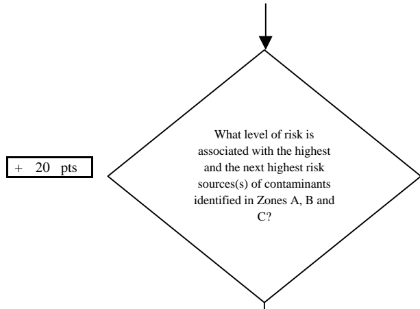
Chart 7. Contaminant risks for McKinley Chalet Resorts - Volatile Organic Chemicals
