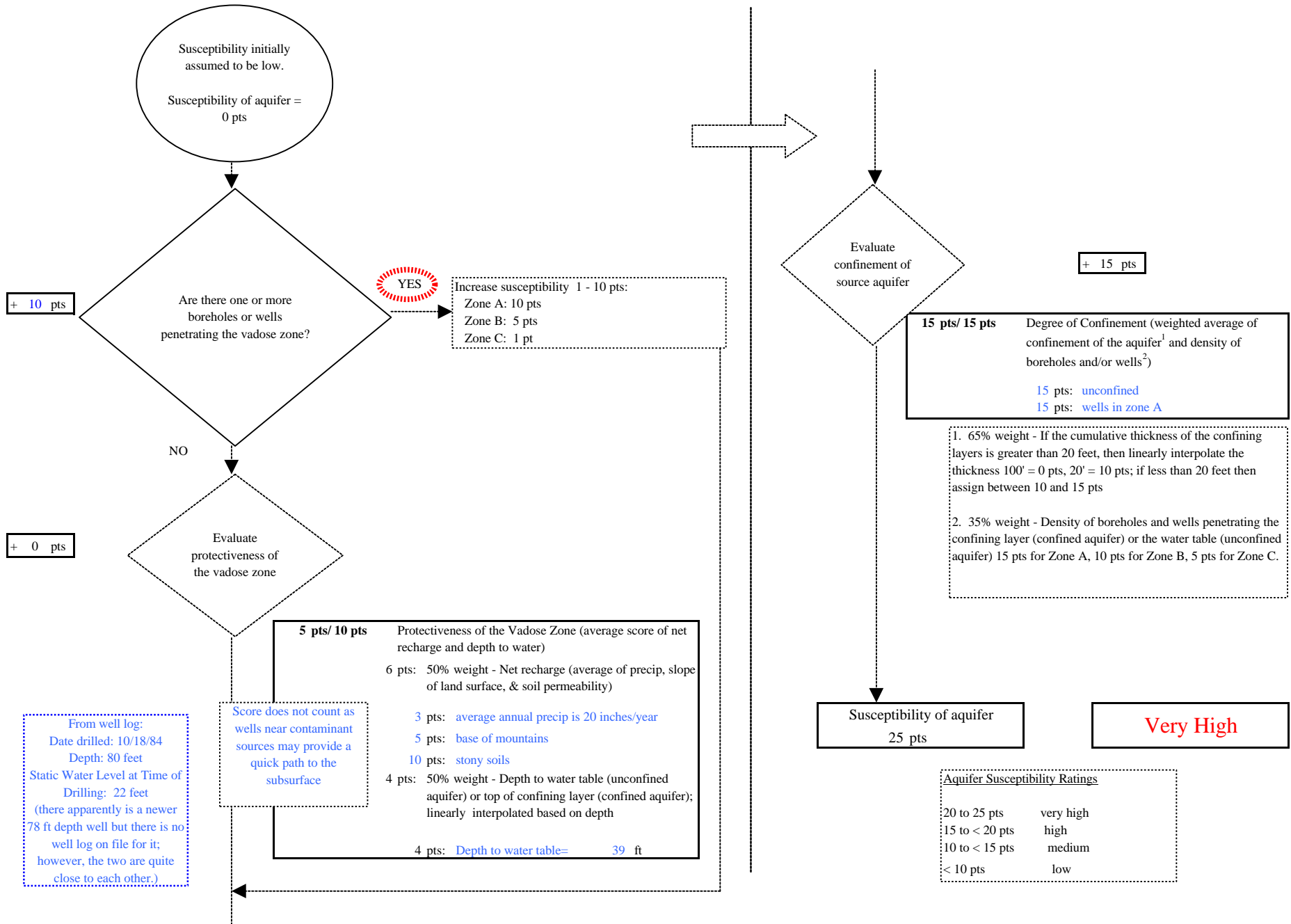
Chart 2. Susceptibility of the aquifer - McKinley Chalet Resorts
