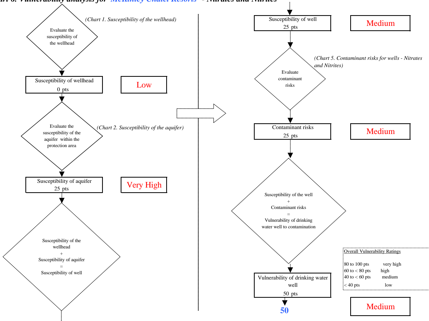
Chart 6. Vulnerability analysis for McKinley Chalet Resorts - Nitrates and Nitrites
