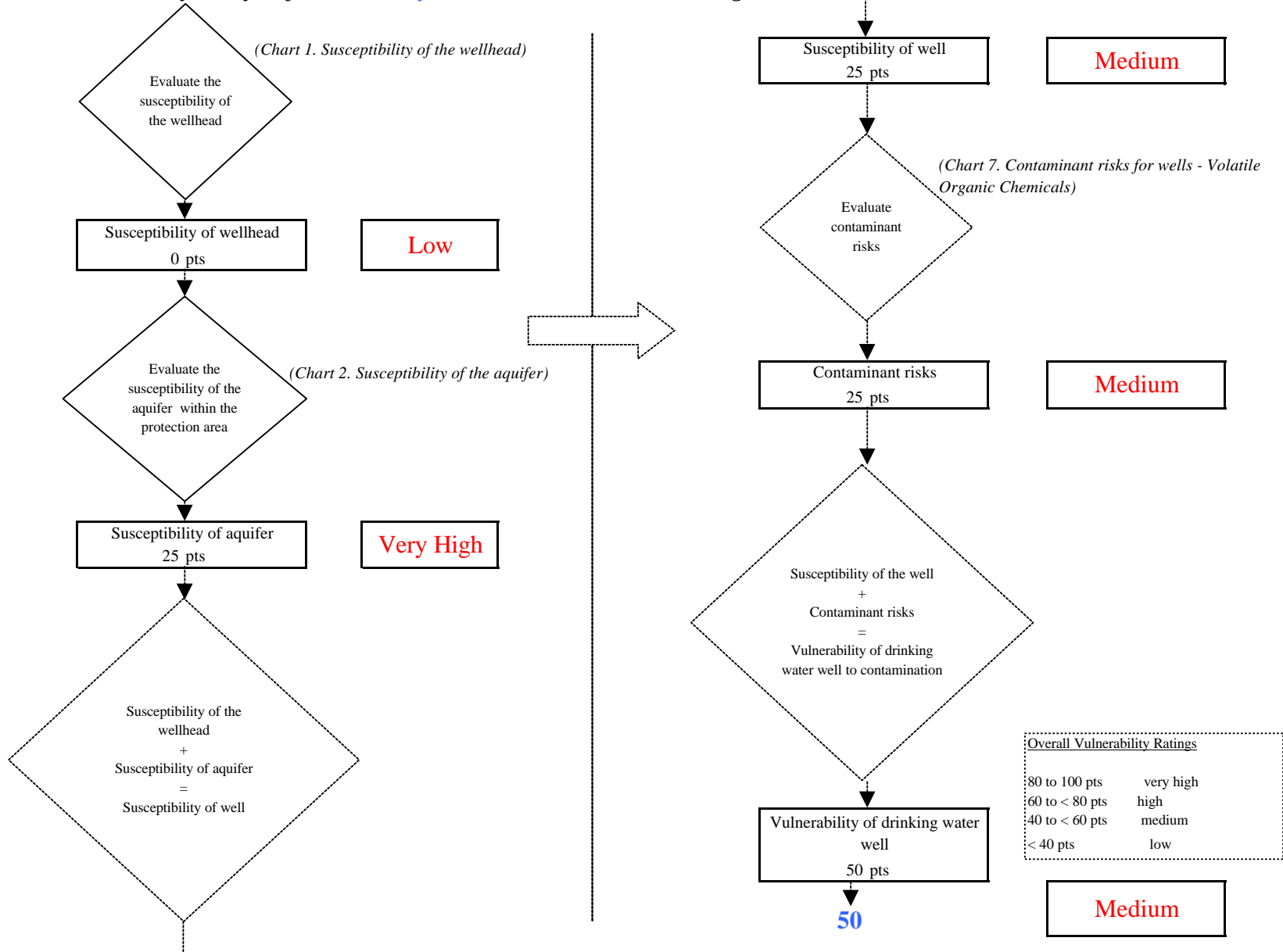
Chart 8. Vulnerability analysis for McKinley Chalet Resorts - Volatile Organic Chemicals
