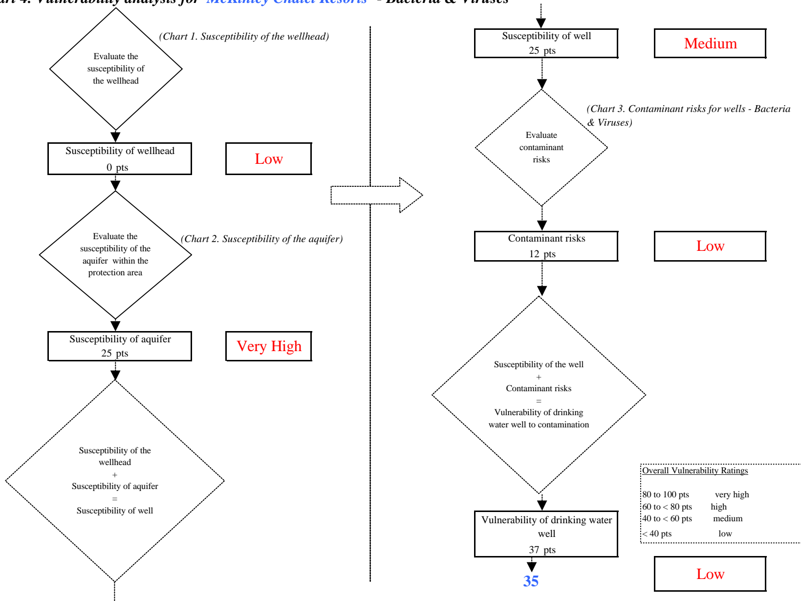
Chart 4. Vulnerability analysis for McKinley Chalet Resorts - Bacteria & Viruses
