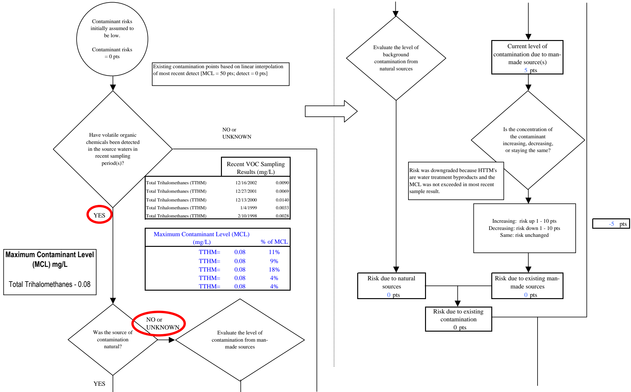
Chart 6. Contaminant risks for LKSD Chief Paul Memorial Kipnuk School Water System (270728.001) - Volatile Organic Chemicals
