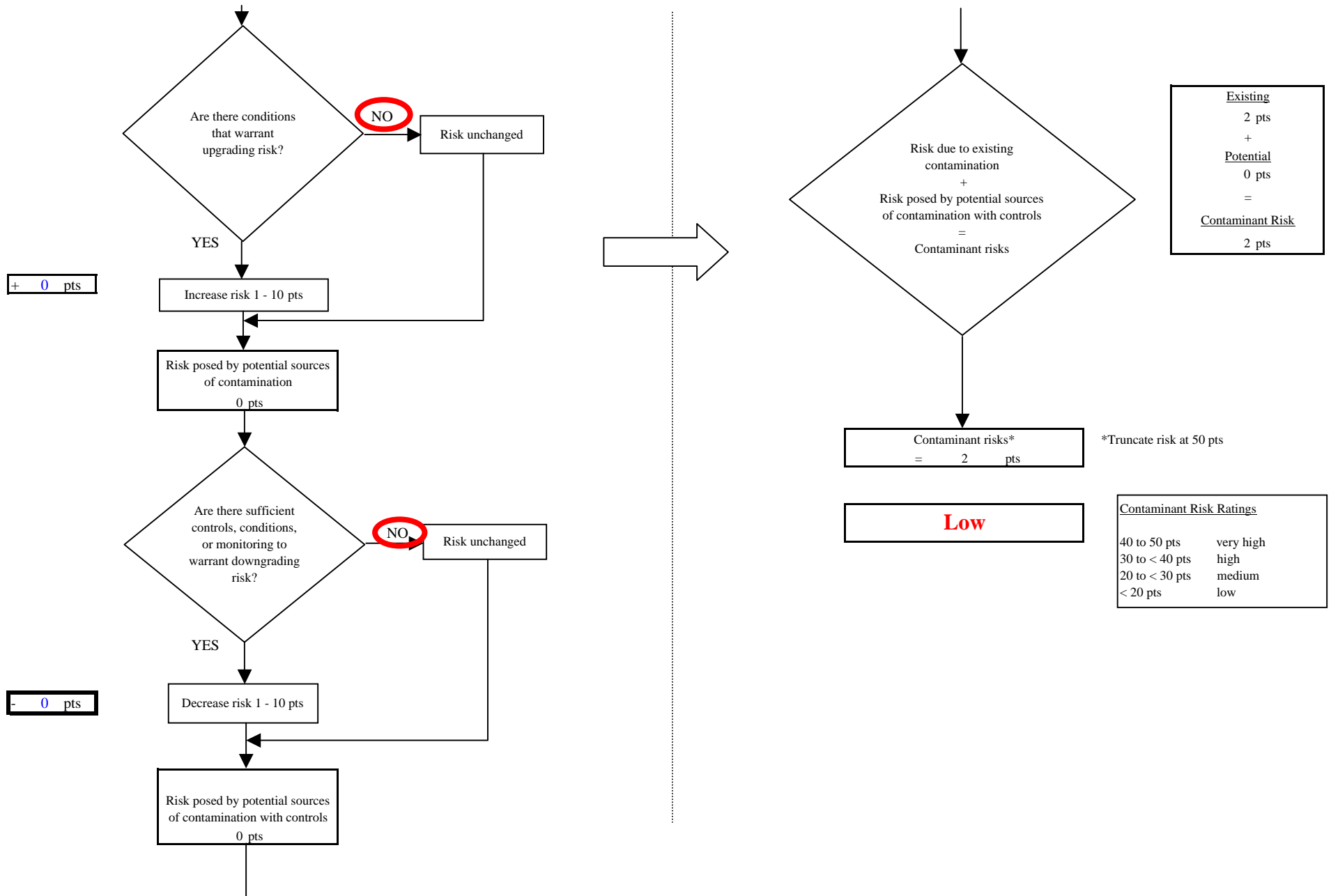
Chart 4. Contaminant risks for LKSD Chief Paul Memorial Kipnuk School Water System (270728.001) - Nitrates and Nitrites
