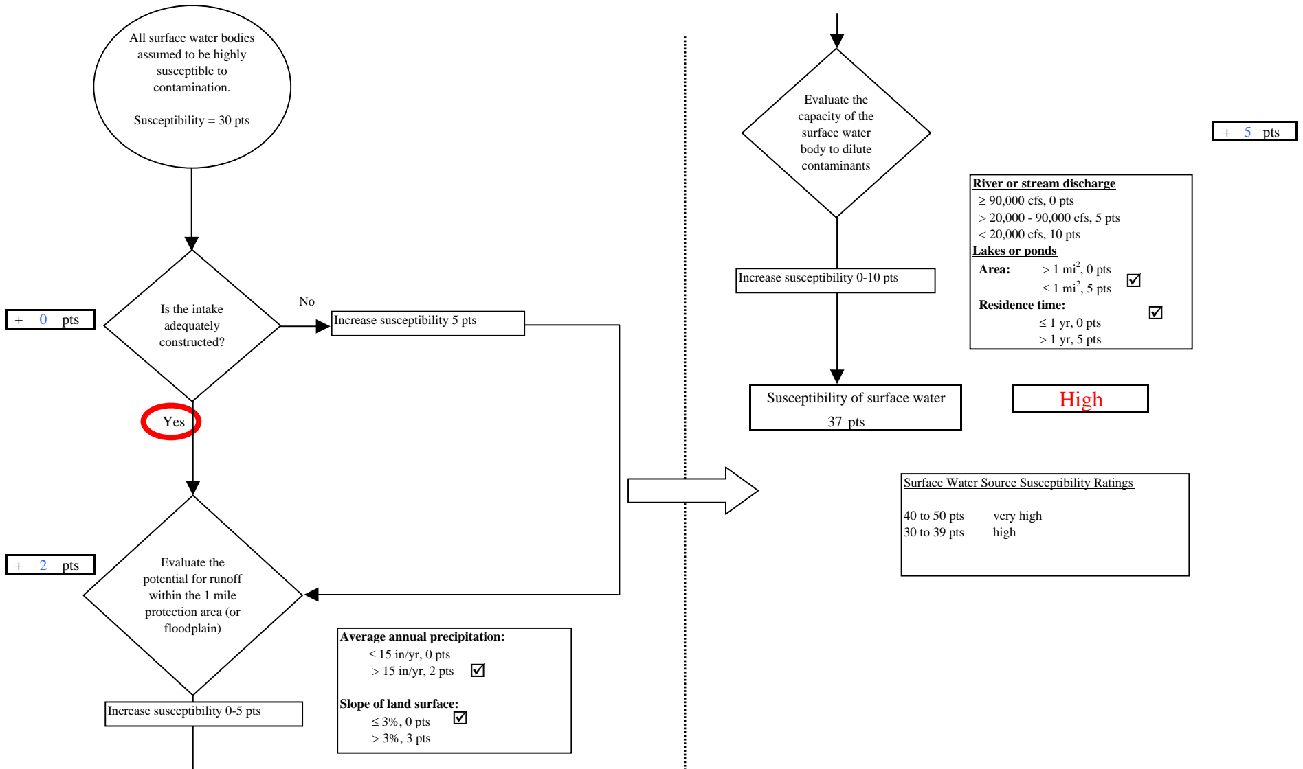
Chart 1. Susceptibility of the Surface Water Source - LKSD Chief Paul Memorial Kipnuk School Water System (270728.001)
