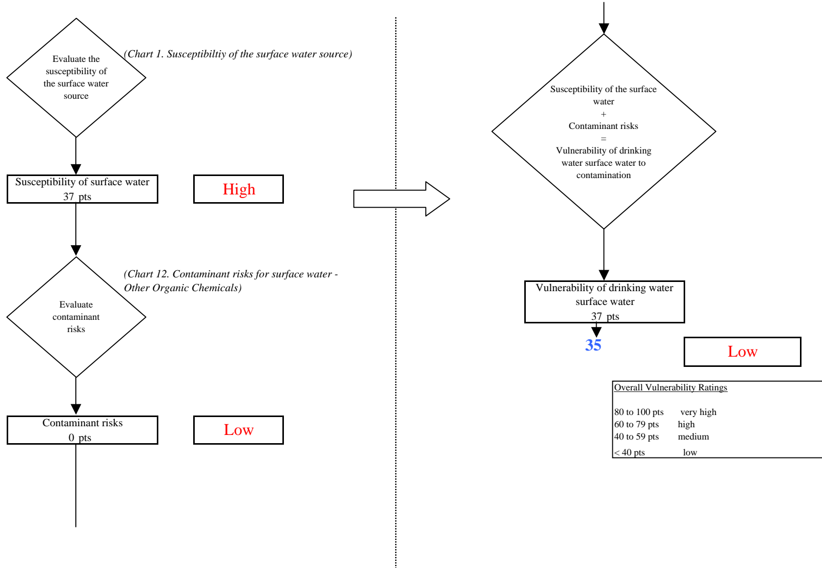
Chart 13. Vulnerability analysis for LKSD Chief Paul Memorial Kipnuk School Water System (270728.001) - Other Organic Chemicals
