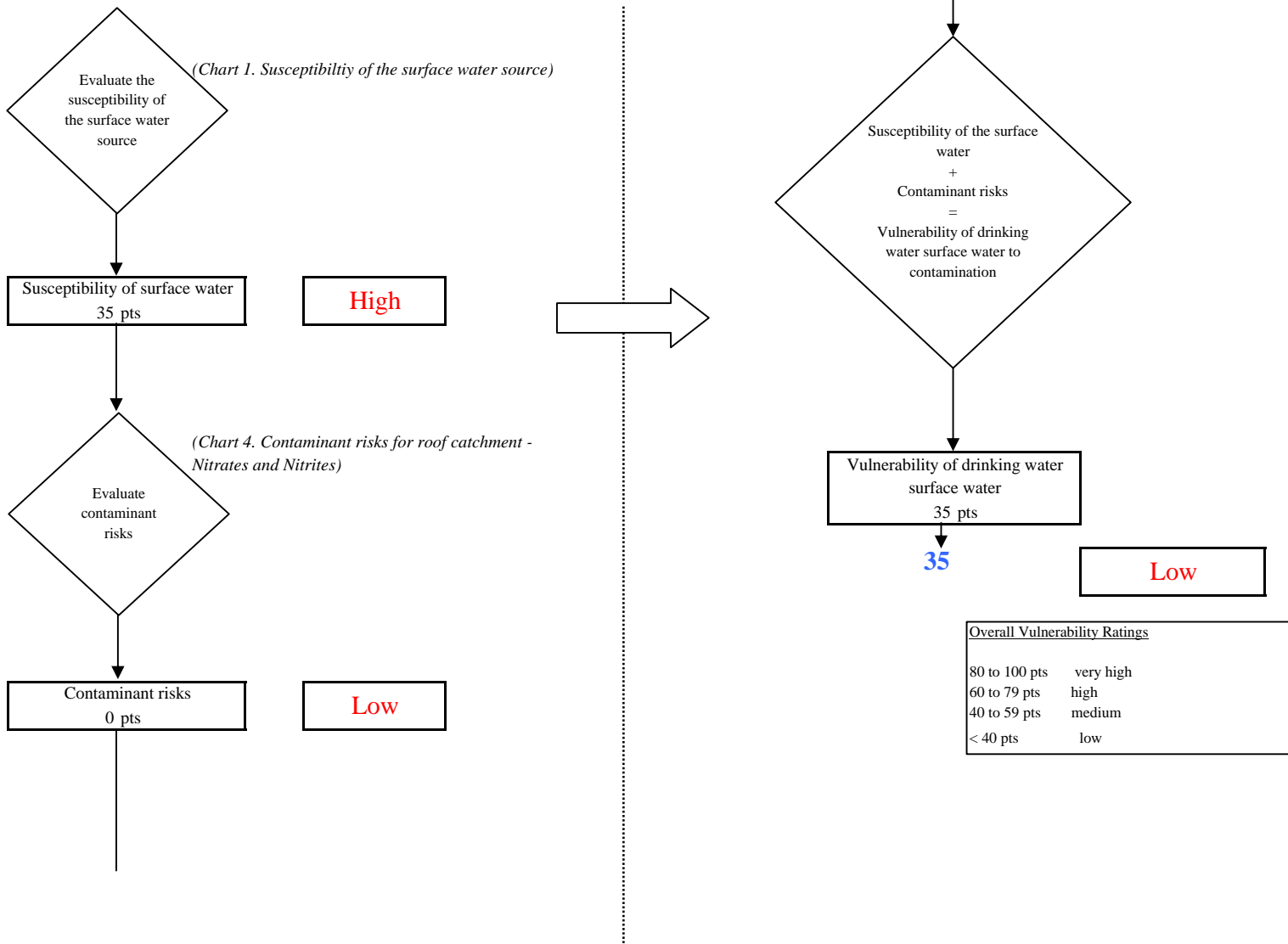
Chart 5. Vulnerability analysis for Mecca Bar - Nitrates and Nitrites
