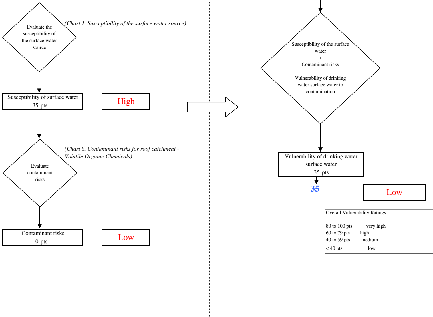
Chart 7. Vulnerability analysis for Mecca Bar - Volatile Organic Chemicals
