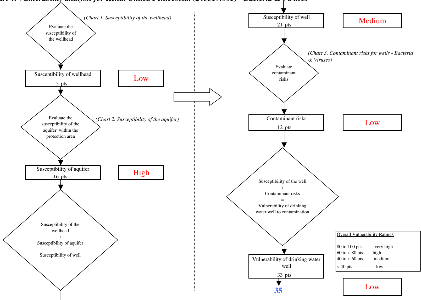
Chart 4. Vulnerability analysis for Kenai United Pentecostal (245317.001) - Bacteria & Viruses
