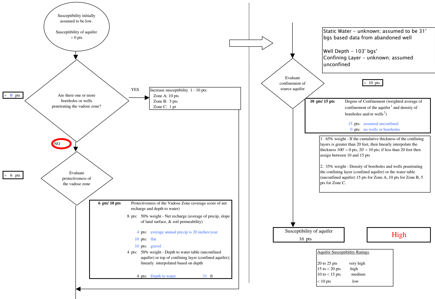
Chart 2. Susceptibility of the aquifer - Kenai United Pentecostal (245317.001)
