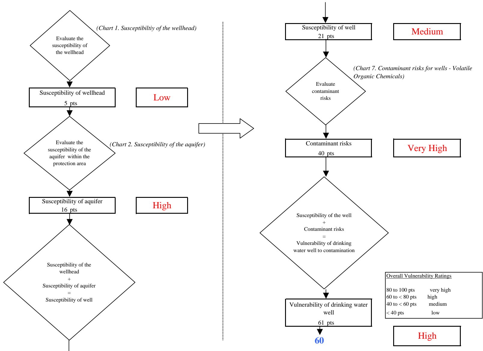
Chart 8. Vulnerability analysis for Kenai United Pentecostal (245317.001) - Volatile Organic Chemicals
