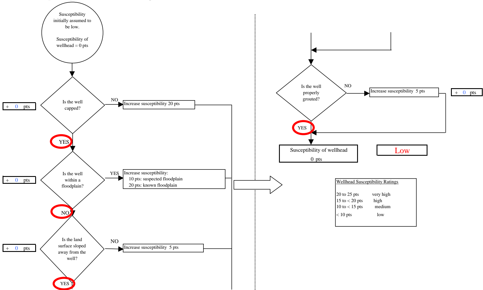
Chart 1. Susceptibility of the wellhead - Snug Harbor Seafoods (242953.002)
