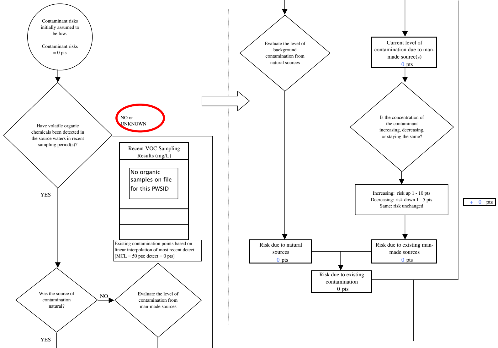
Chart 7. Contaminant risks for Robinson Grocery and Deli (243640.002) - Volatile Organic Chemicals
