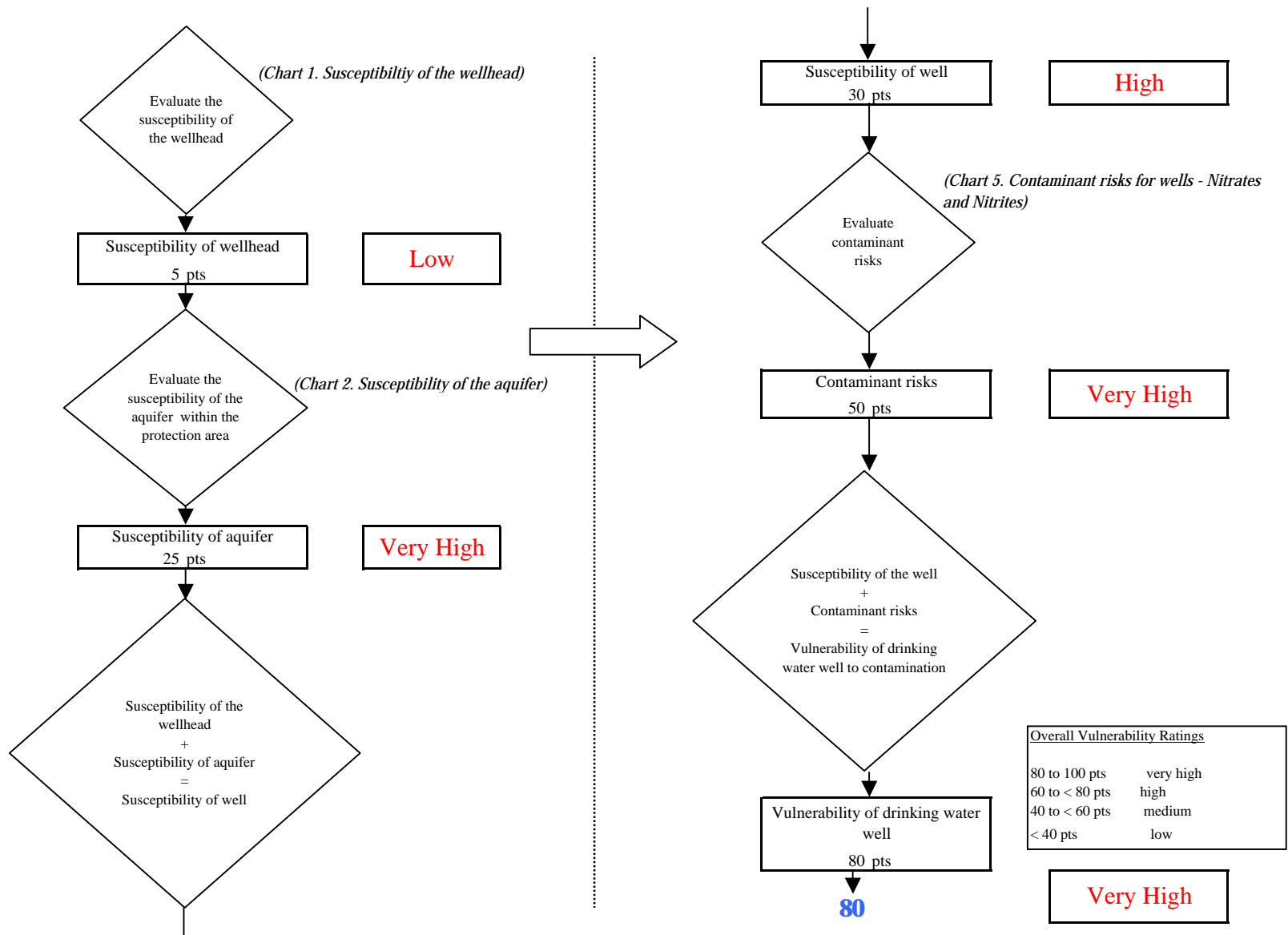
Chart 6. Vulnerability analysis for Robinson Grocery and Deli (243640.002) - Nitrates and Nitrites
