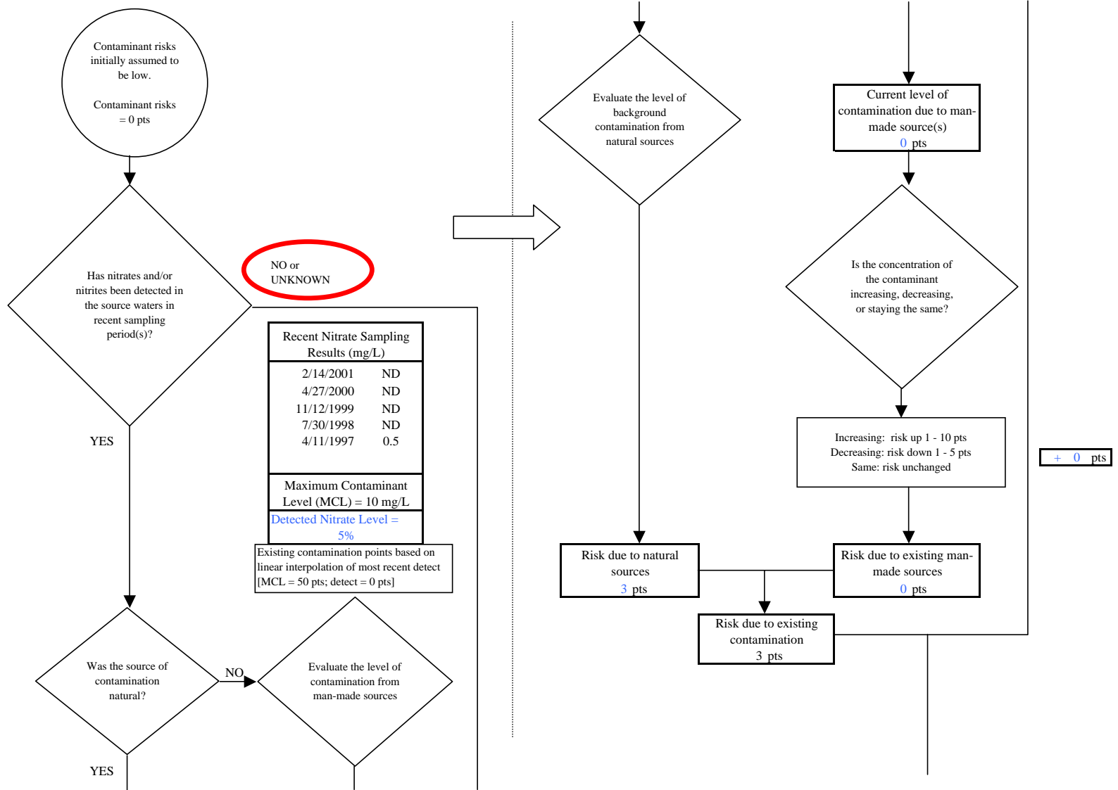
Chart 5. Contaminant risks for Robinson Grocery and Deli (243640.002) - Nitrates and Nitrites
