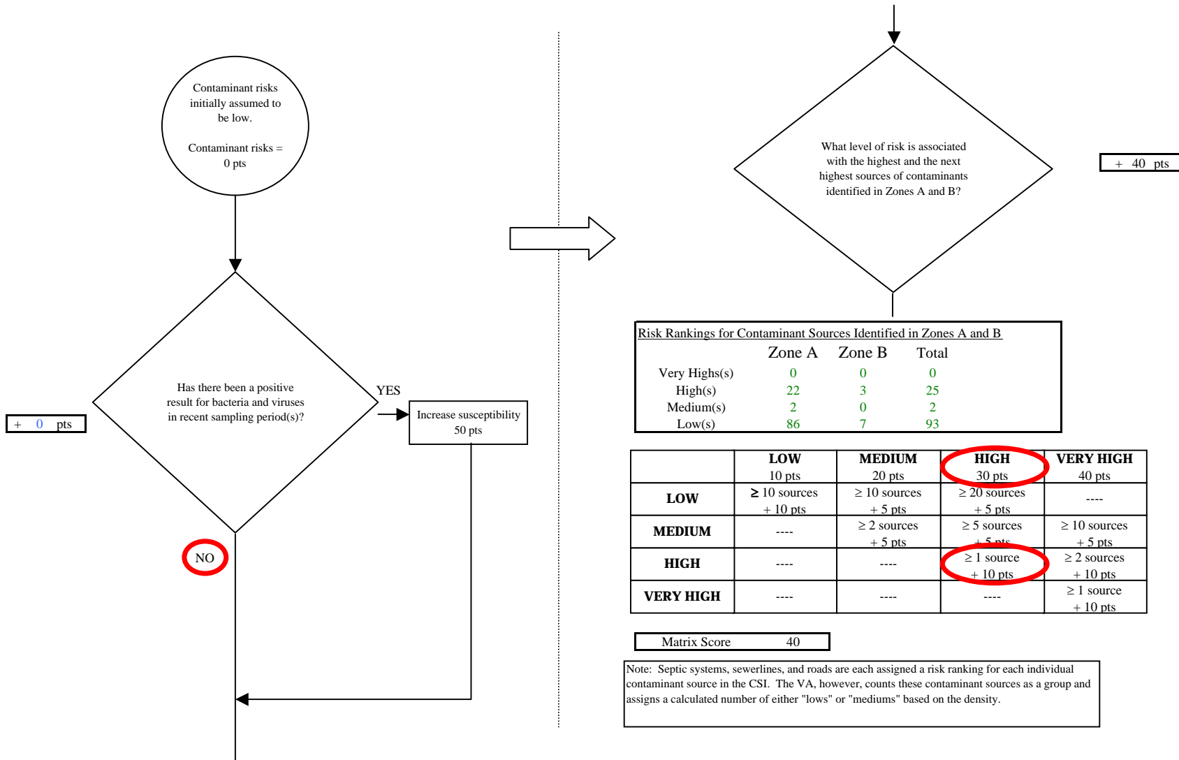
Chart 3. Contaminant risks for Robinson Grocery and Deli (243640.002) - Bacteria & Viruses
