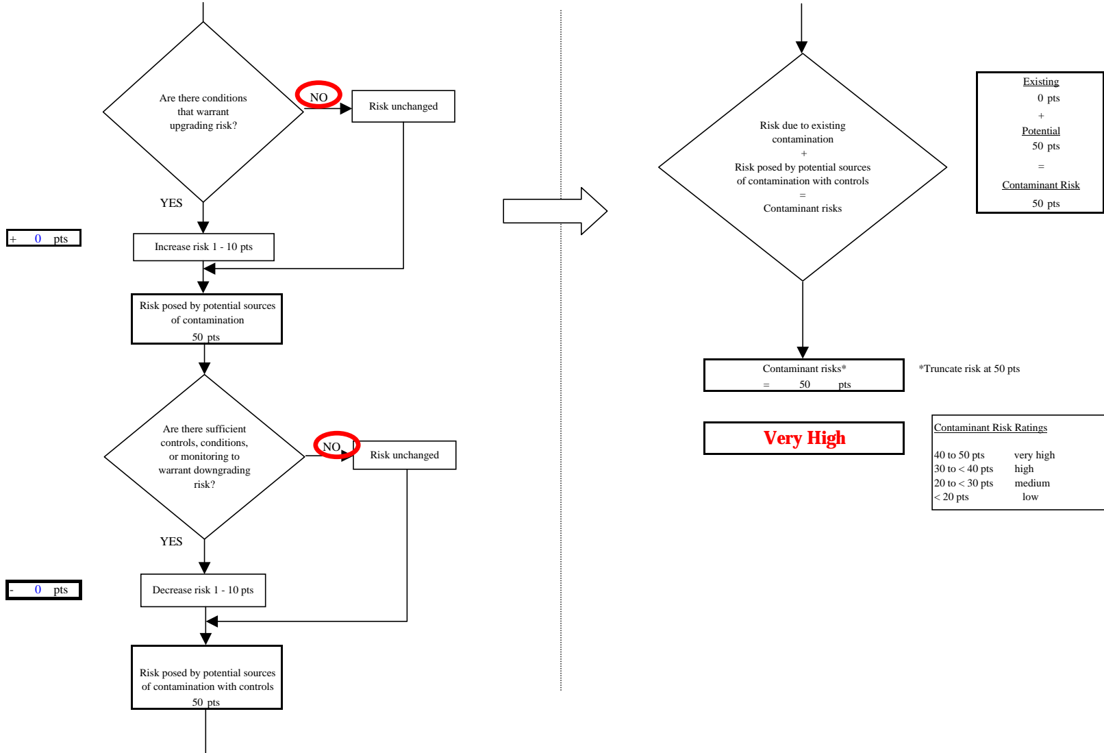
Chart 7. Contaminant risks for Robinson Grocery and Deli (243640.002) - Volatile Organic Chemicals
