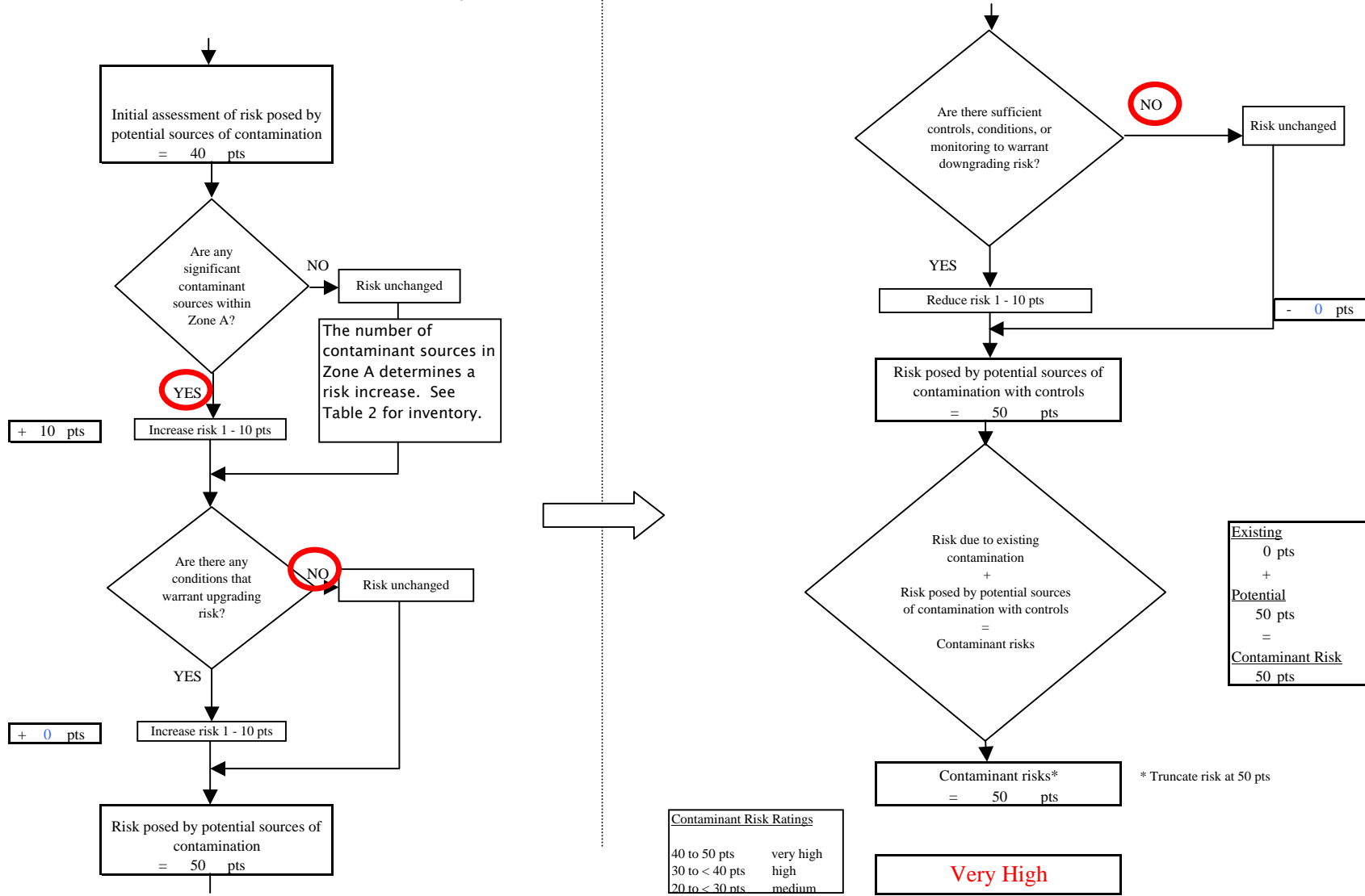
Chart 3. Contaminant risks for Robinson Grocery and Deli (243640.002) - Bacteria & Viruses
