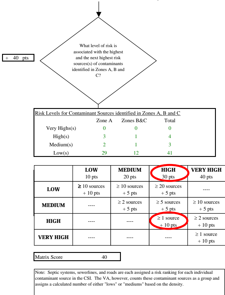
Chart 7. Contaminant risks for Robinson Grocery and Deli (243640.002) - Volatile Organic Chemicals
