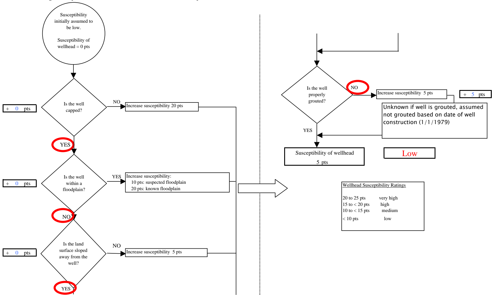
Chart 1. Susceptibility of the wellhead - Robinson Grocery and Deli (243640.002)
