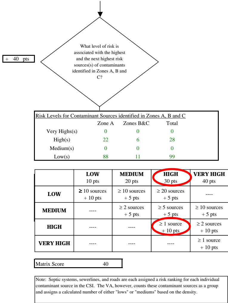
Chart 5. Contaminant risks for Robinson Grocery and Deli (243640.002) - Nitrates and Nitrites
