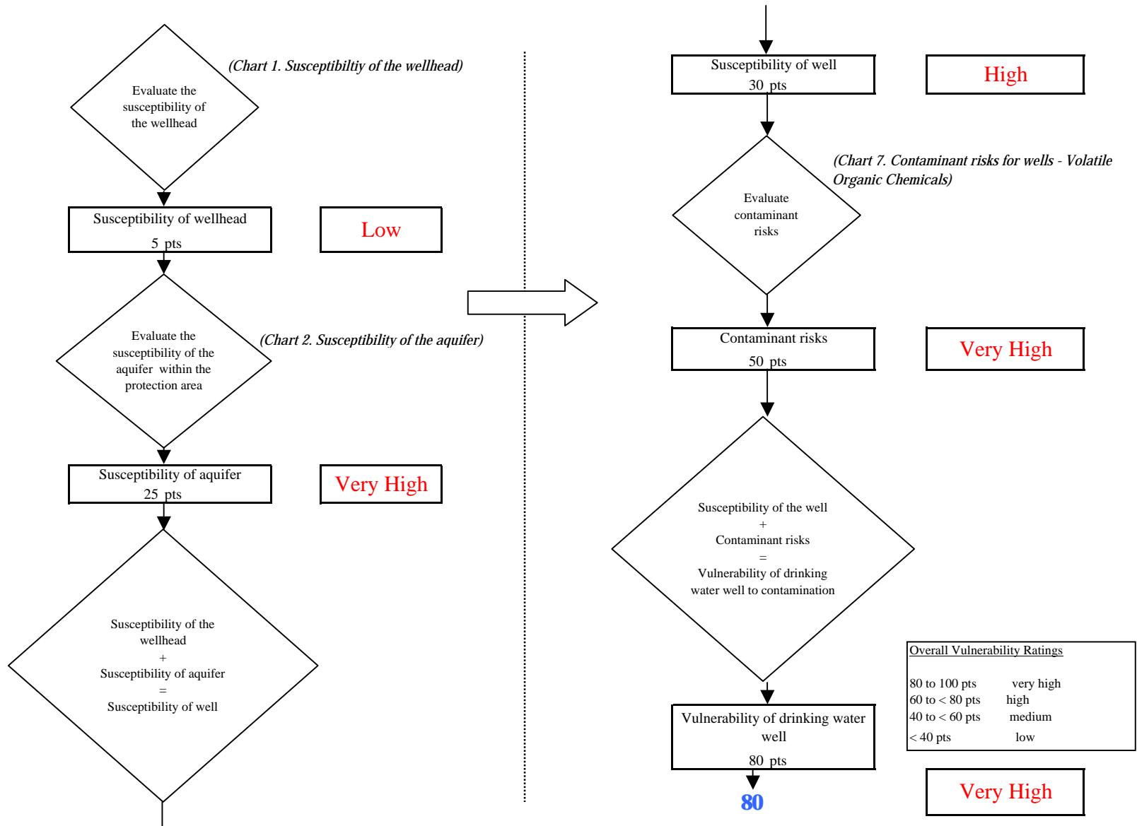
Chart 8. Vulnerability analysis for Robinson Grocery and Deli (243640.002) - Volatile Organic Chemicals
