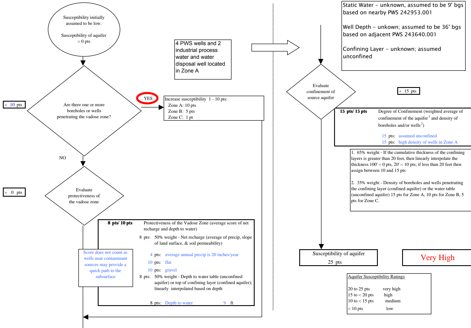
Chart 2. Susceptibility of the aquifer - Robinson Grocery and Deli (243640.002)
