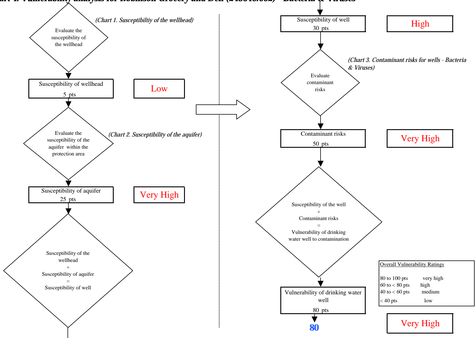
Chart 4. Vulnerability analysis for Robinson Grocery and Deli (243640.002) - Bacteria & Viruses
