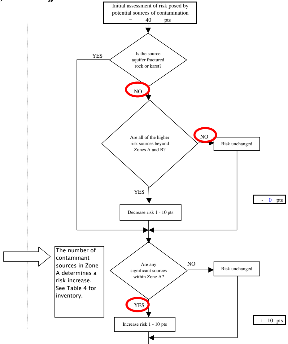
Chart 7. Contaminant risks for Robinson Grocery and Deli (243640.002) - Volatile Organic Chemicals
