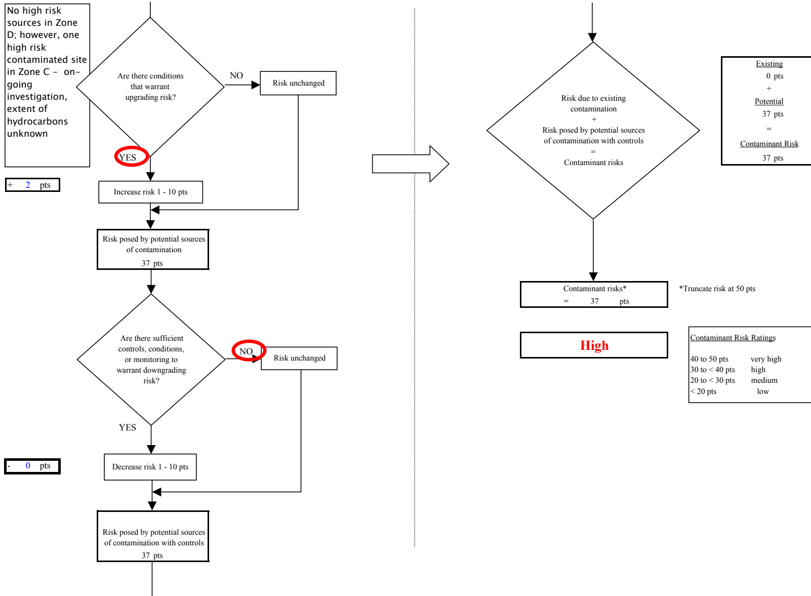
Chart 7. Contaminant risks for Kenai Boating Facility (244353.001) - Volatile Organic Chemicals
