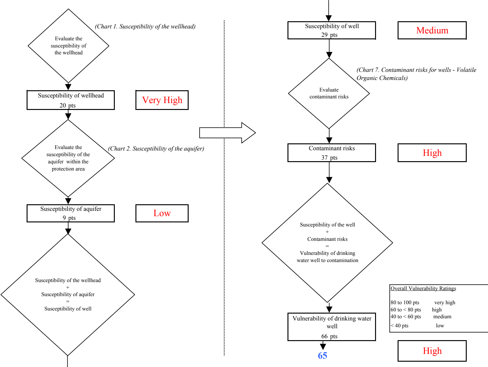
Chart 8. Vulnerability analysis for Kenai Boating Facility (244353.001) - Volatile Organic Chemicals
