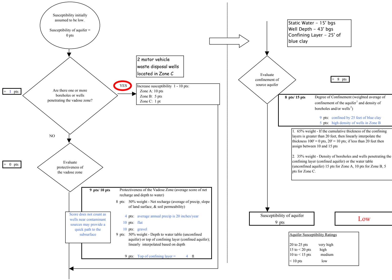
Chart 2. Susceptibility of the aquifer - Kenai Boating Facility (244353.001)
