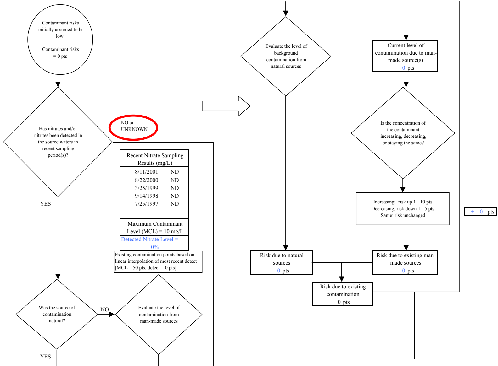
Chart 5. Contaminant risks for Kenai Boating Facility (244353.001) - Nitrates and Nitrites
