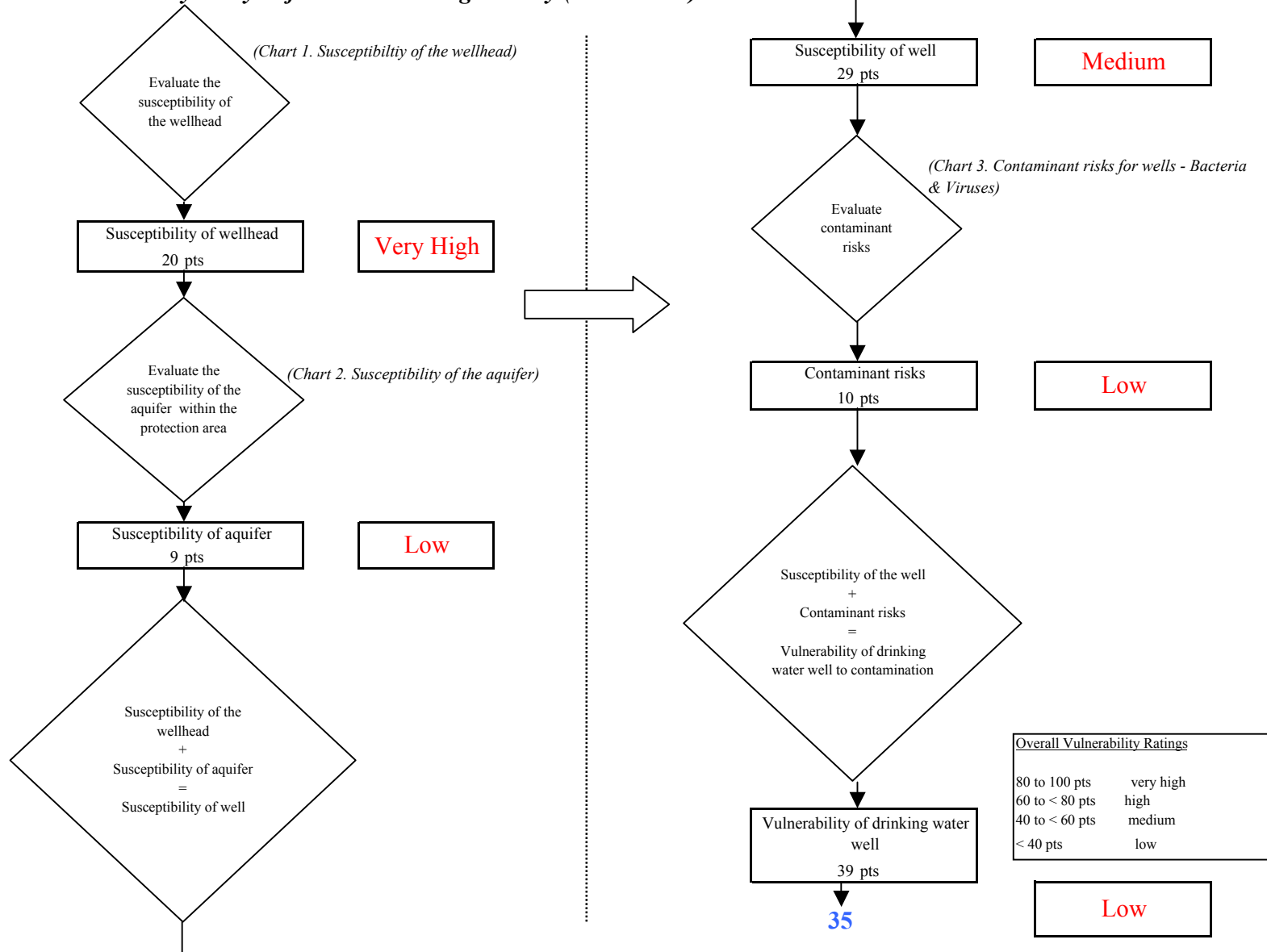
Chart 4. Vulnerability analysis for Kenai Boating Facility (244353.001) - Bacteria & Viruses
