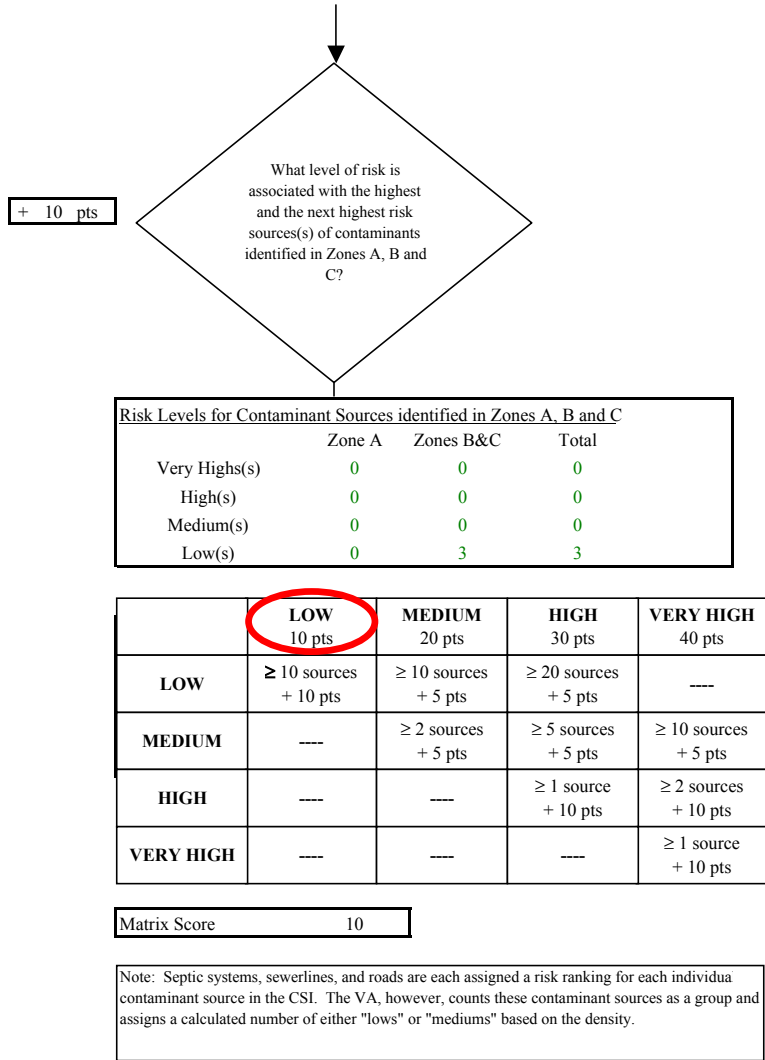
Chart 5. Contaminant risks for Kenai Boating Facility (244353.001) - Nitrates and Nitrites
