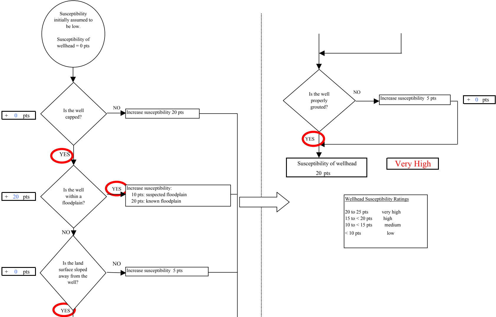
Chart 1. Susceptibility of the wellhead - Kenai Boating Facility (244353.001)
