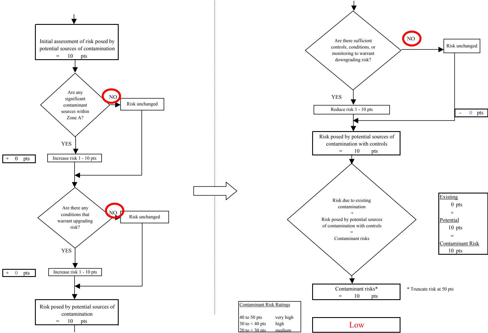
Chart 3. Contaminant risks for Kenai Boating Facility (244353.001) - Bacteria & Viruses
