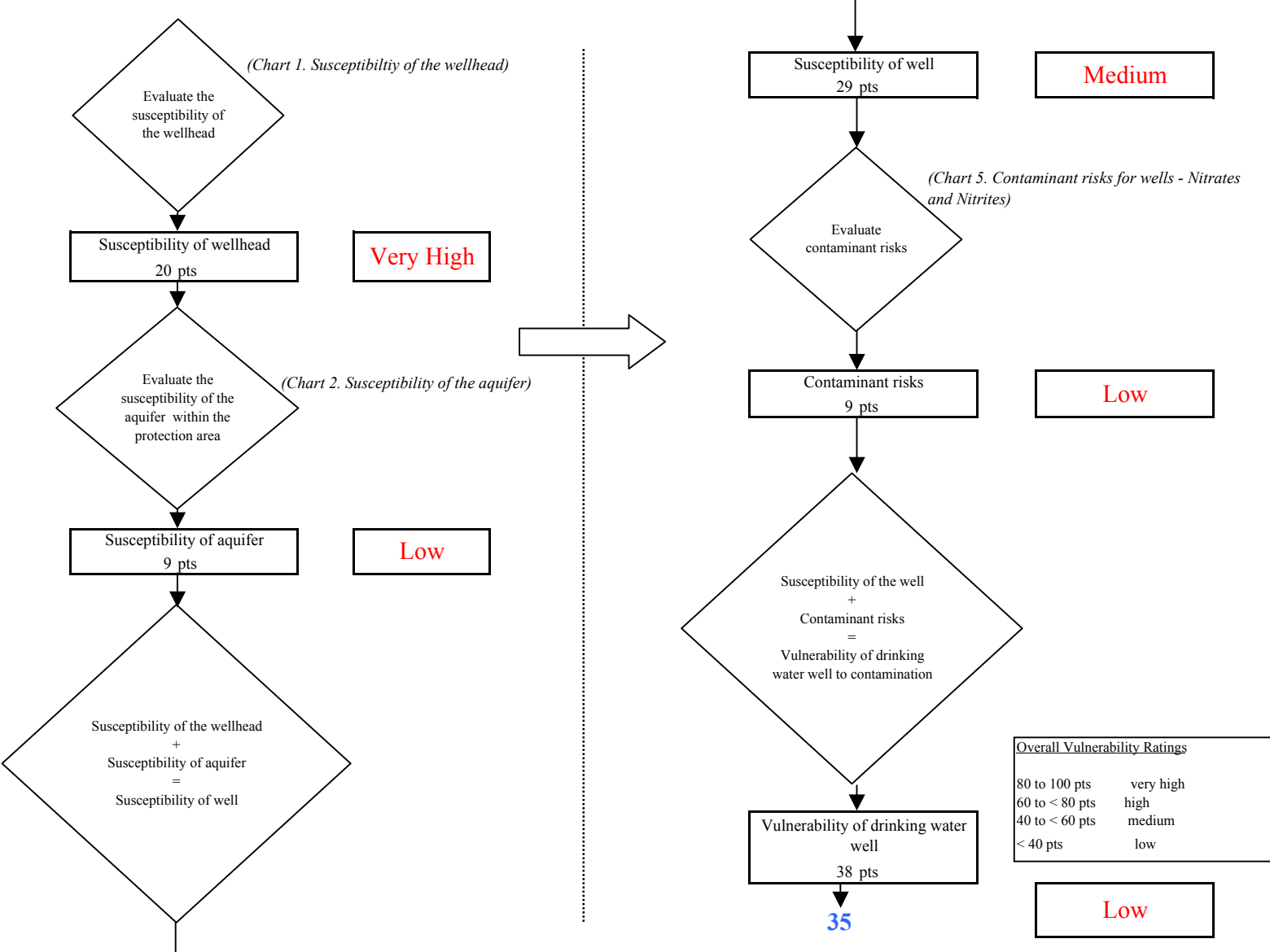
Chart 6. Vulnerability analysis for Kenai Boating Facility (244353.001) - Nitrates and Nitrites
