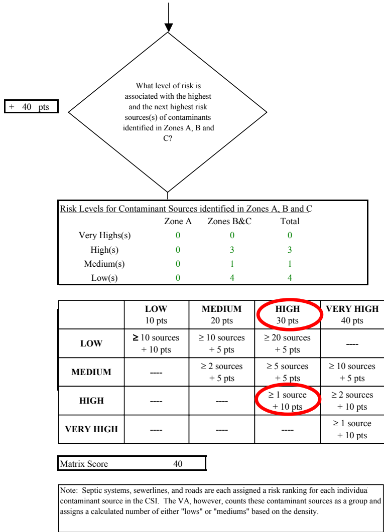
Chart 7. Contaminant risks for Kenai Boating Facility (244353.001) - Volatile Organic Chemicals
