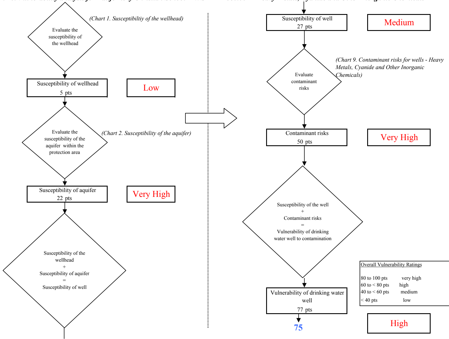
Chart 10. Vulnerability analysis for Kalifornsky Christian School- PWSID 242660.001 - Heavy Metals, Cyanide and Other Inorganic Chemicals
