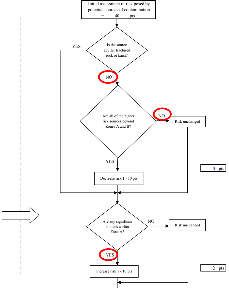
Chart 7. Contaminant risks for Kalifornsky Christian School- PWSID 242660.001 - Volatile Organic Chemicals
