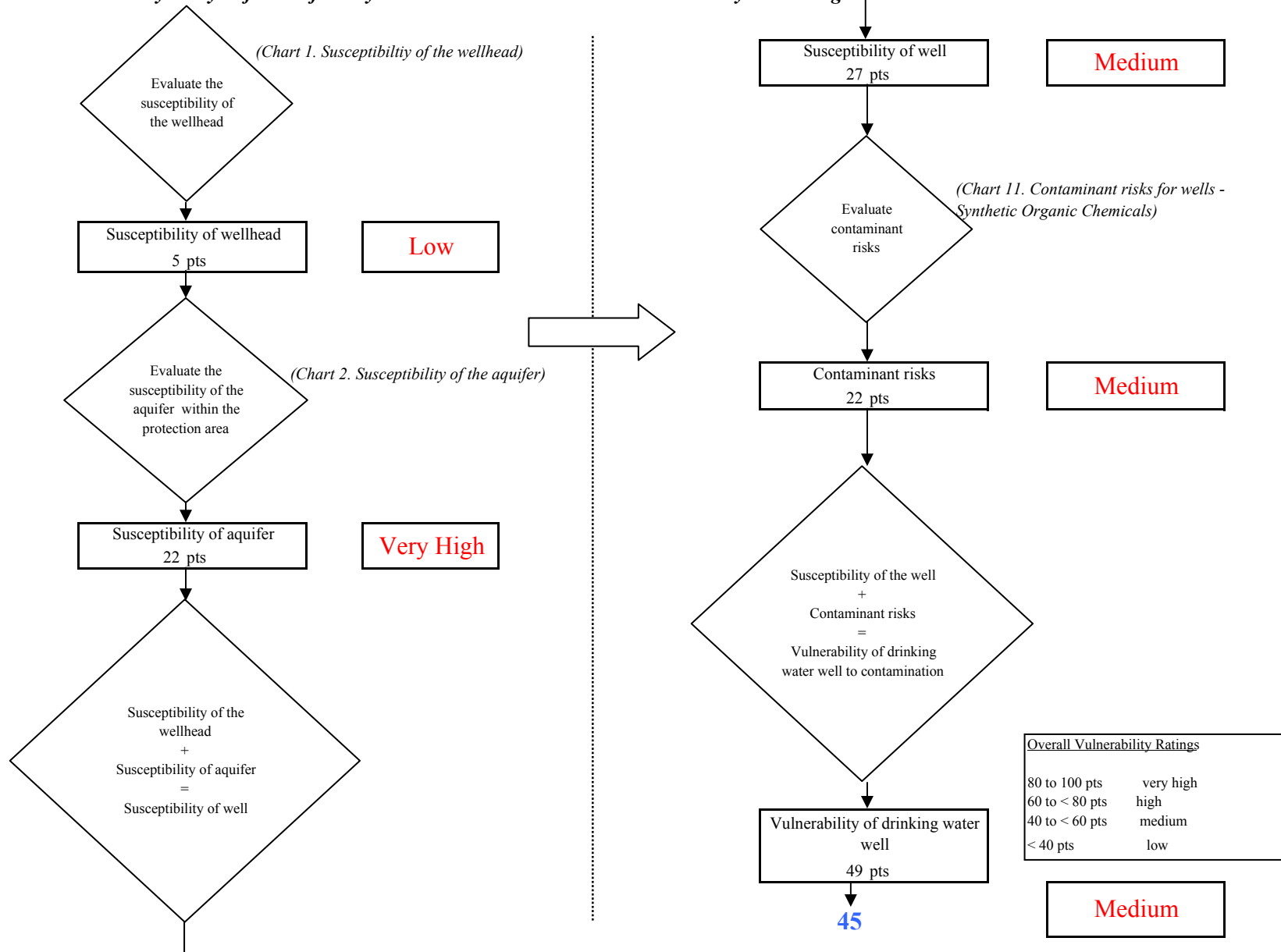
Chart 12. Vulnerability analysis for Kalifornsky Christian School- PWSID 242660.001 - Synthetic Organic Chemicals
