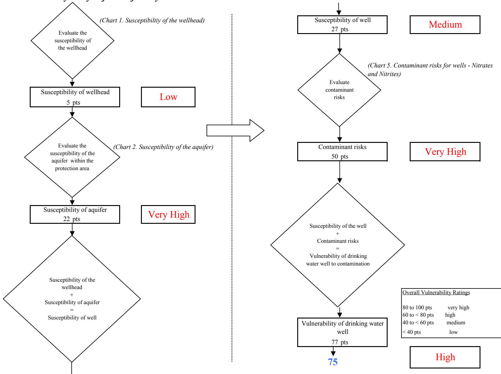
Chart 6. Vulnerability analysis for Kalifornsky Christian School- PWSID 242660.001 - Nitrates and Nitrites
