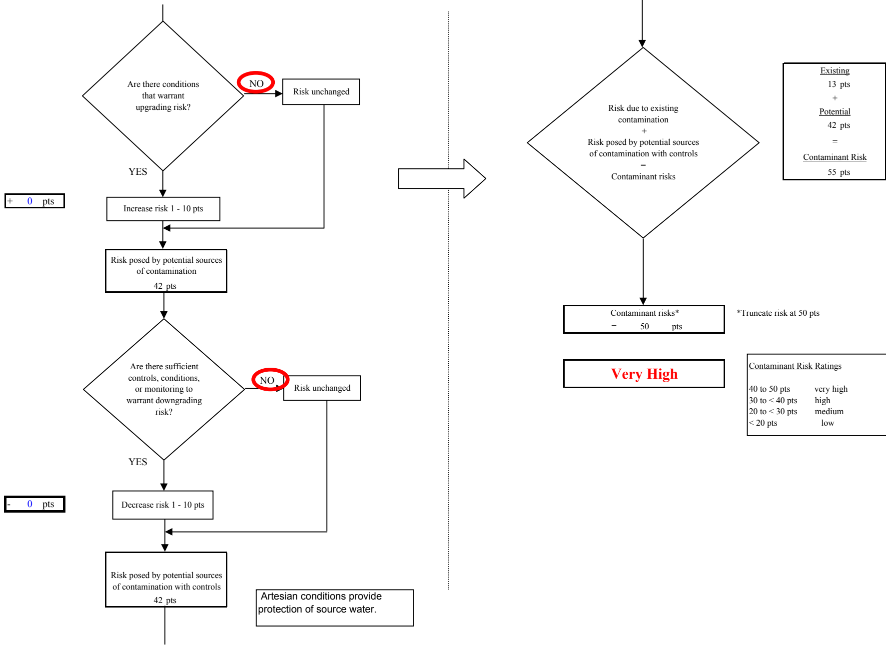
Chart 9. Contaminant risks for Kalifornsky Christian School- PWSID 242660.001 - Heavy Metals, Cyanide and Other Inorganic Chemicals
