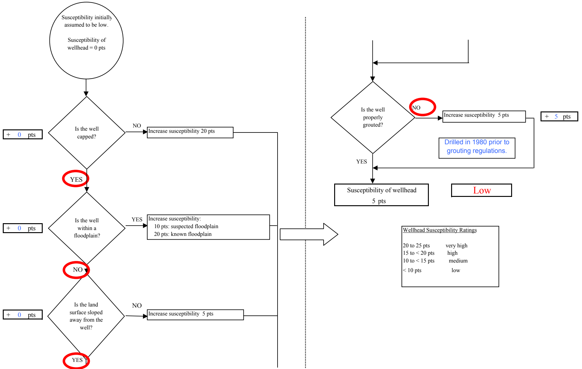
Chart 1. Susceptibility of the wellhead - Kalifornsky Christian School- PWSID 242660.001
