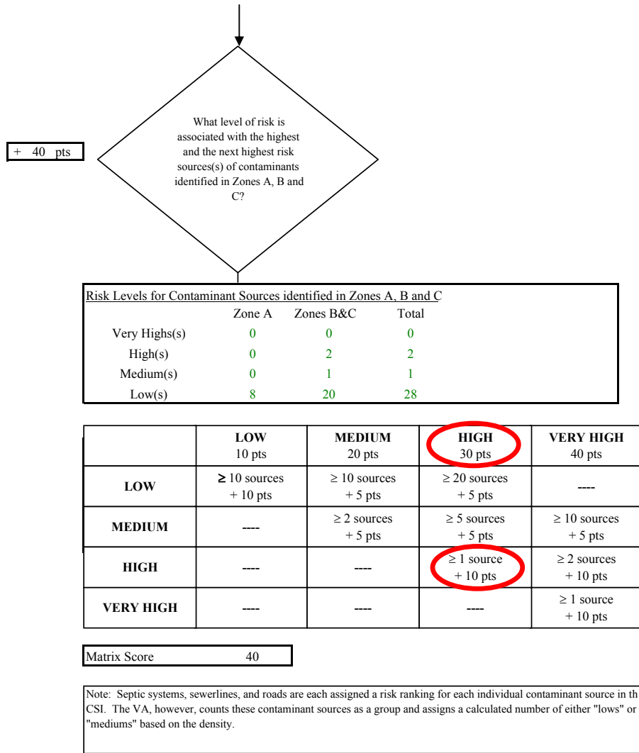
Chart 7. Contaminant risks for Kalifornsky Christian School- PWSID 242660.001 - Volatile Organic Chemicals
