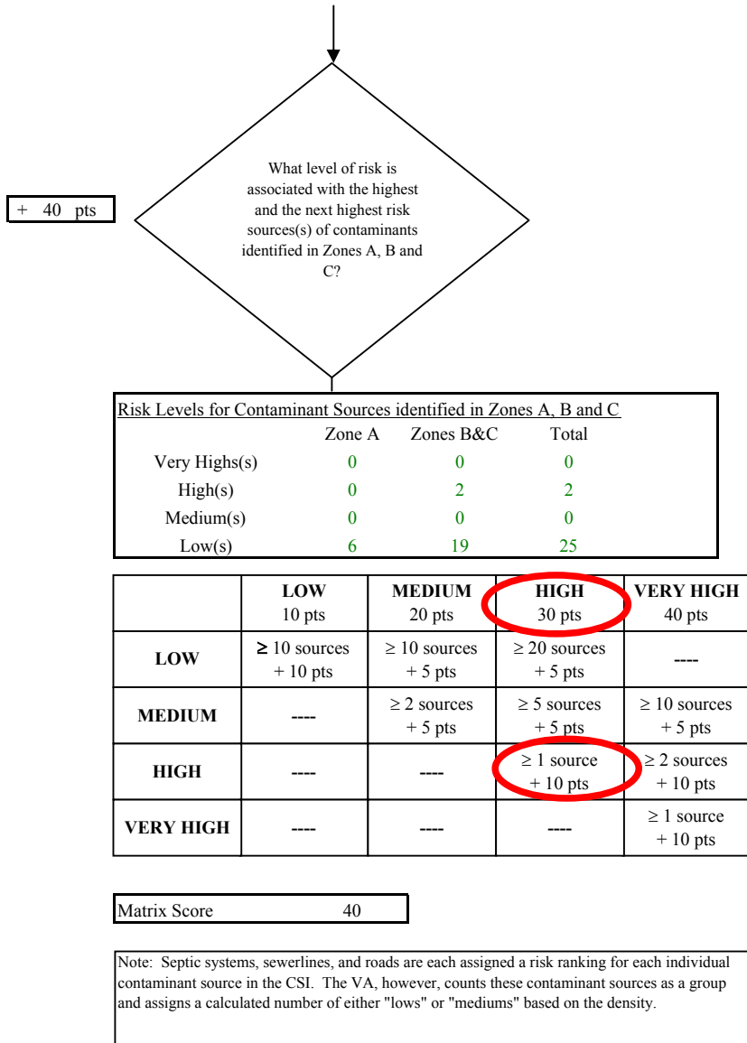
Chart 9. Contaminant risks for Kalifornsky Christian School- PWSID 242660.001 - Heavy Metals, Cyanide and Other Inorganic Chemicals
